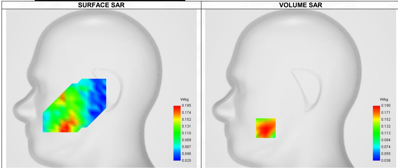
Maximum location: X=-57.00, Y=-65.00 ; SAR Peak: 0.32 W/kg
