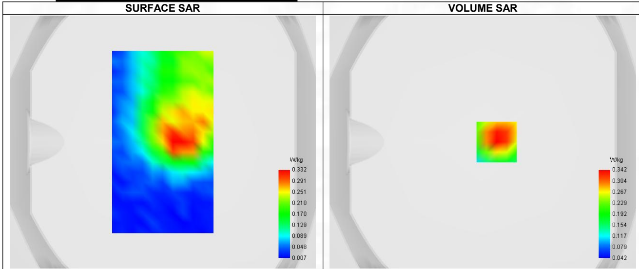
Maximum location: X=11.00, Y=0.00 ; SAR Peak: 0.58 W/kg
