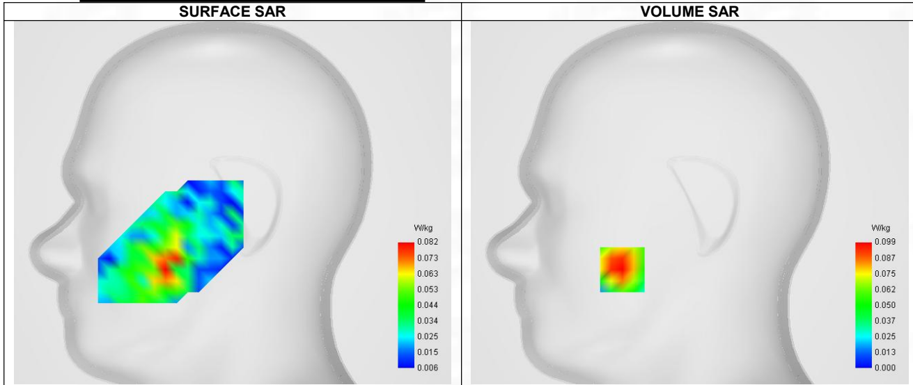
Maximum location: X=-48.00, Y=-48.00 ; SAR Peak: 0.18 W/kg
