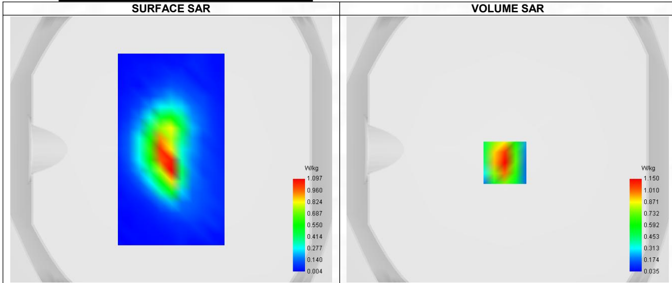
Maximum location: X=0.00, Y=16.00 ; SAR Peak: 1.20 W/kg
