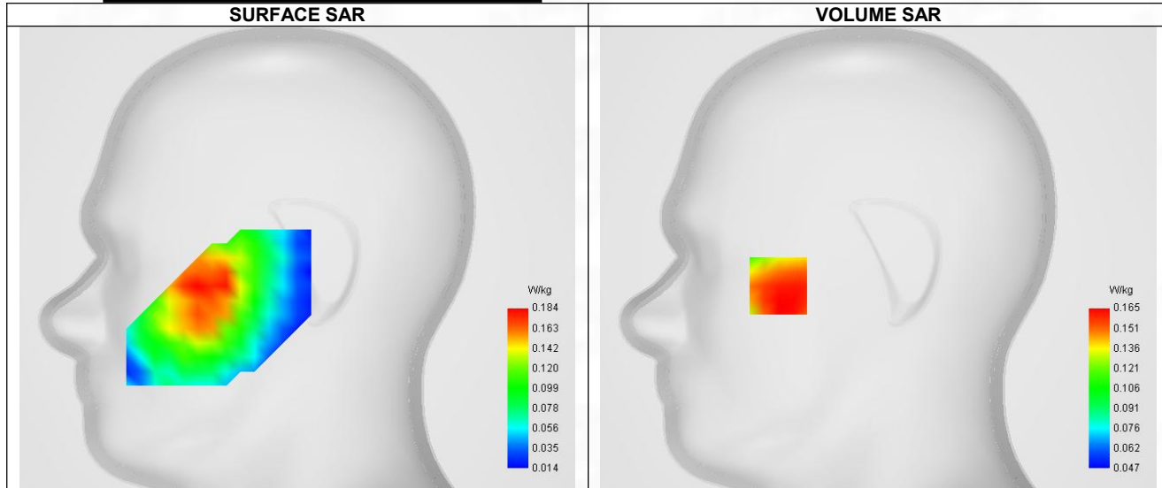
Maximum location: X=-56.00, Y=-16.00 ; SAR Peak: 0.20 W/kg
