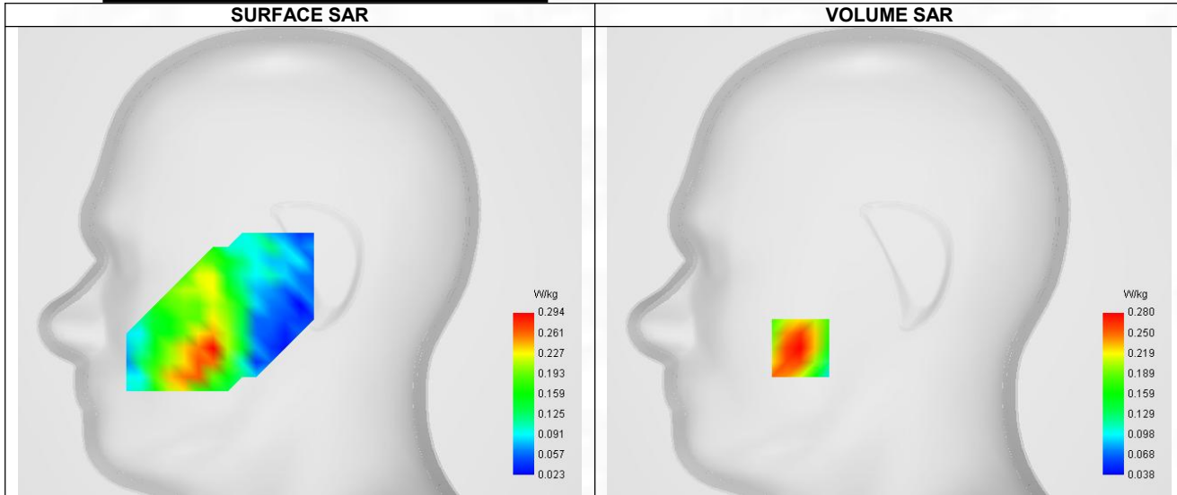
Maximum location: X=-49.00, Y=-48.00 ; SAR Peak: 0.43 W/kg
