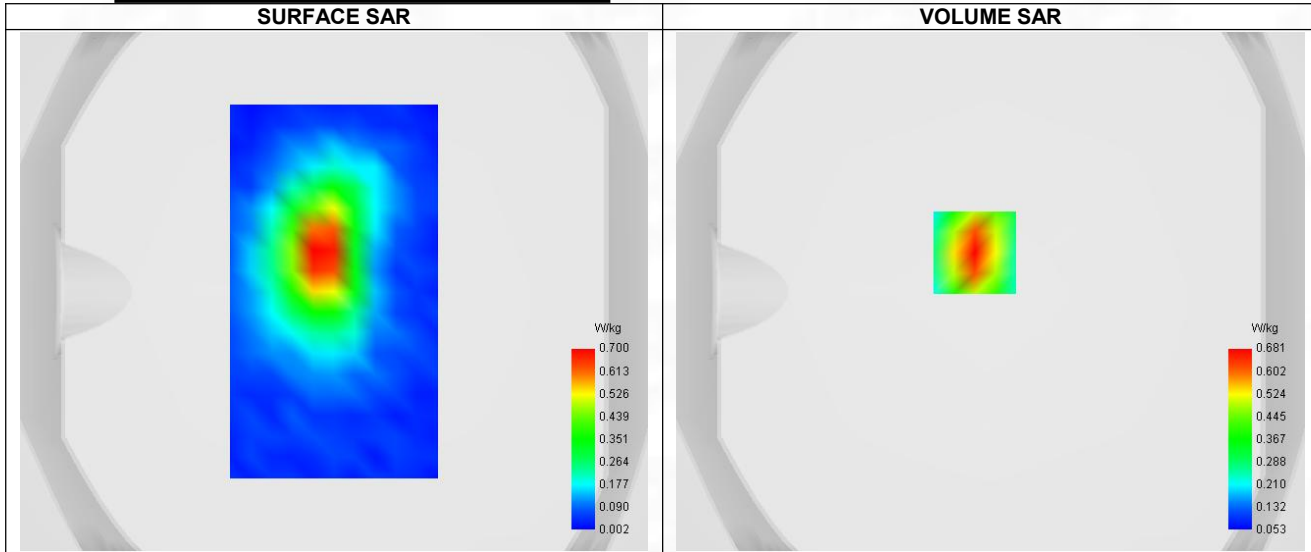
Maximum location: X=-6.00, Y=15.00 ; SAR Peak: 1.07 W/kg
