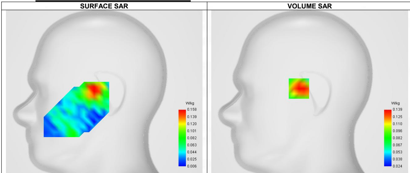
Maximum location: X=-17.00, Y=5.00 ; SAR Peak: 0.20 W/kg
