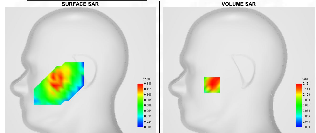
Maximum location: X=-55.00, Y=-31.00 ; SAR Peak: 0.17 W/kg
