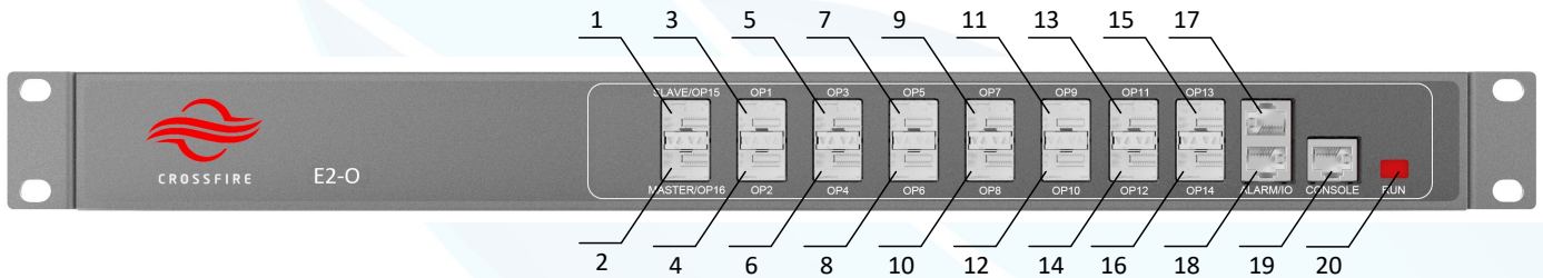
E2 Front Panel Interfaces
