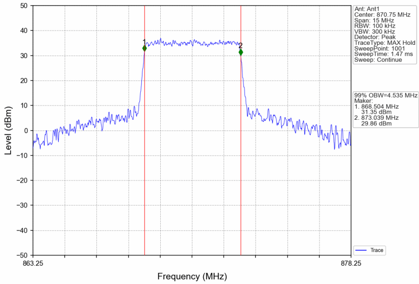
Band26b_870.75MHz_AWGN_SISO_Ant1_NTNV_AGC
