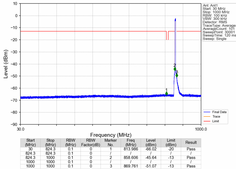
Band26a_861.5MHz_AWGN_SISO_Ant1_NTNV
