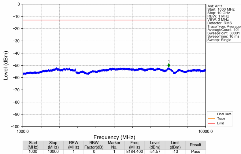
Band26a_861.5MHz_AWGN_SISO_Ant1_NTNV
