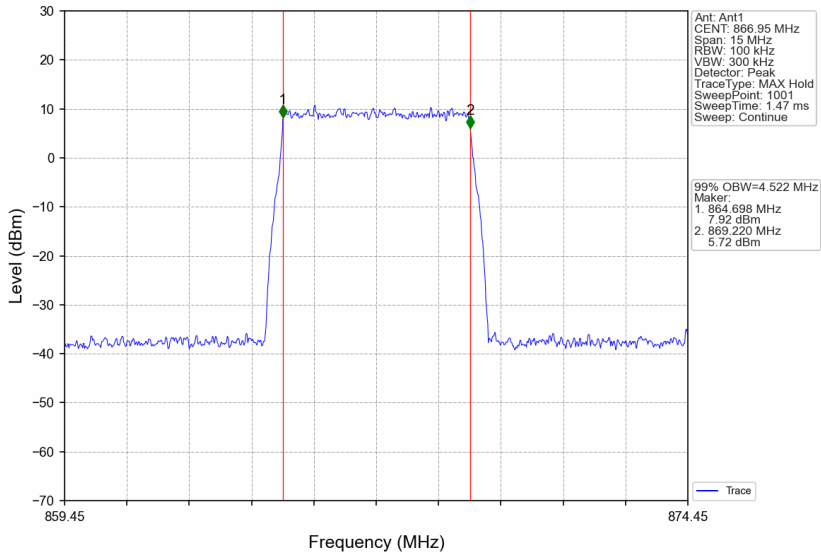
Band26a_866.95MHz_AWGN_SISO_Ant1_NTNV_AGC
