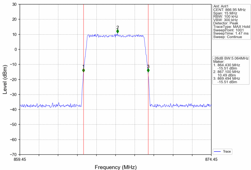
Band26a_866.95MHz_AWGN_SISO_Ant1_NTNV_AGC
