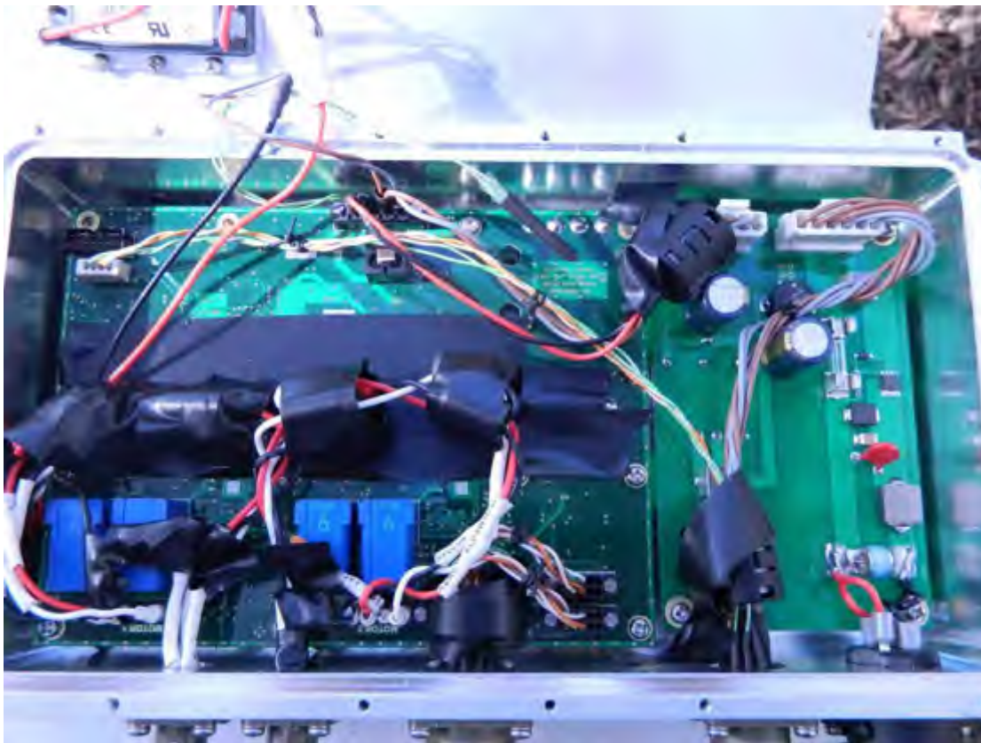
Photo 7 - Internal view of control module, 1.2m dish
