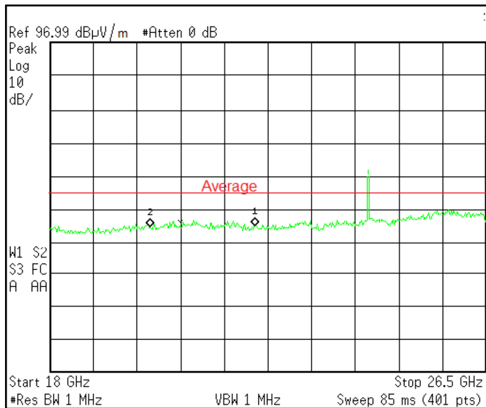
Figure 5b. Radiated Emissions, 1.2m dish - 18 GHz to 26.5 GHz (Horizontal)
