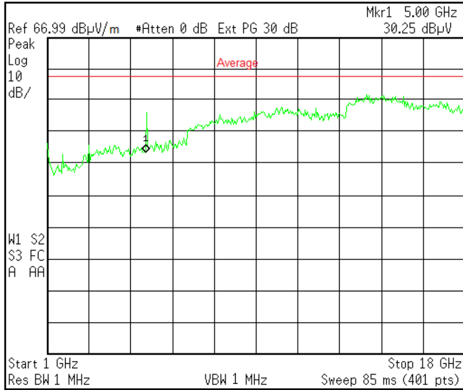
Figure 3a. Radiated Emissions, 1.2m dish - 1 GHz to 18 GHz (Vertical)
