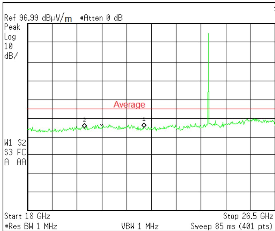
Figure 5a. Radiated Emissions, 1.2m dish - 18 GHz to 26.5 GHz (Vertical)
