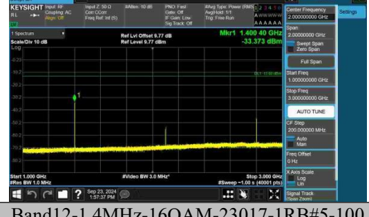
Band12-1.4MHz-16QAM-23017-1RB#5-100 0~3000-PASS
