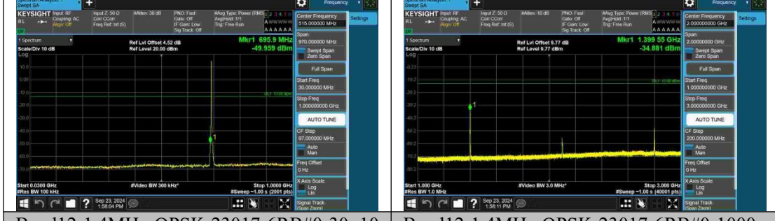
Band12-1.4MHz-QPSK-23017-6RB#0-30~1000-PASS
