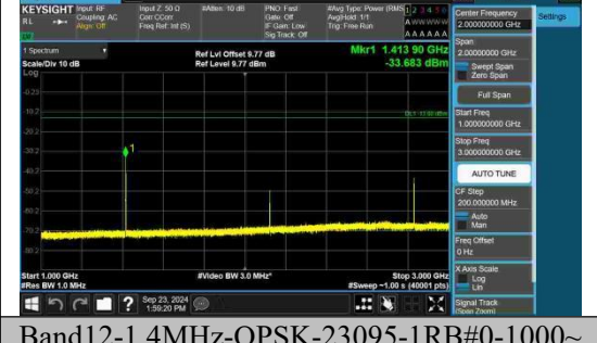
Band12-1.4MHz-QPSK-23095-1RB#0-1000~ 3000-PASS
