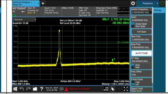
Band4-20MHz-16QAM-20300-100RB#0-1000~3000-PASS
