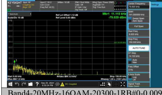
Band4-20MHz-16QAM-20300-1RB#0-0.009~0.15-PASS
