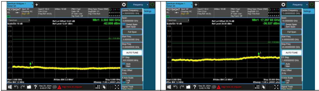
Band4-10MHz-QPSK-20350-50RB#0-3000~6000-PASS
