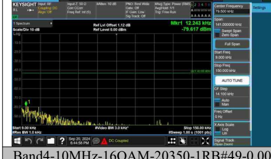
Band4-10MHz-16QAM-20350-1RB#49-0.009~0.15-PASS
