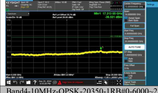
Band4-10MHz-QPSK-20350-1RB#0-6000~20000-PASS
