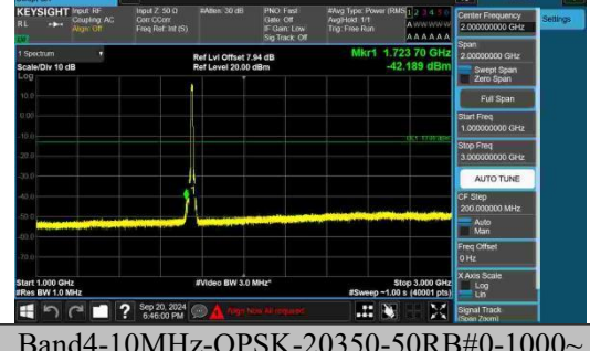
Band4-10MHz-QPSK-20350-50RB#0-1000~3000-PASS
