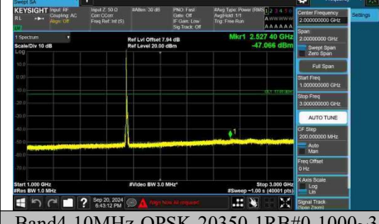
Band4-10MHz-QPSK-20350-1RB#0-1000~3000-PASS
