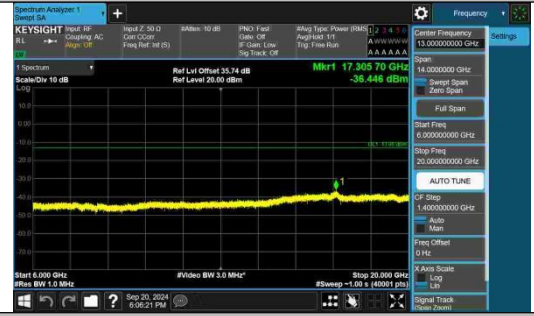
Band4-3MHz-16QAM-20385-15RB#0-6000~20000-PASS
