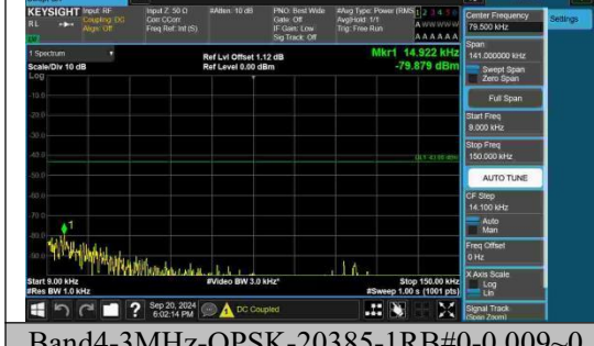
Band4-3MHz-QPSK-20385-1RB#0-0.009~0.15-PASS
