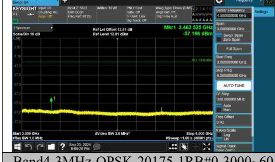
Band4-3MHz-QPSK-20175-1RB#0-3000~6000-PASS
