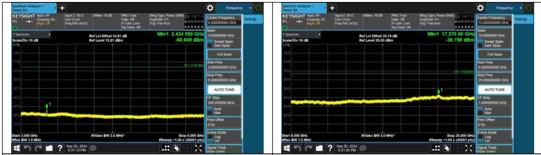
Band4-5MHz-QPSK-19975-25RB#0-3000~6000-PASS
