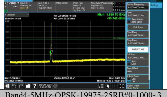
Band4-5MHz-QPSK-19975-25RB#0-1000~3000-PASS
