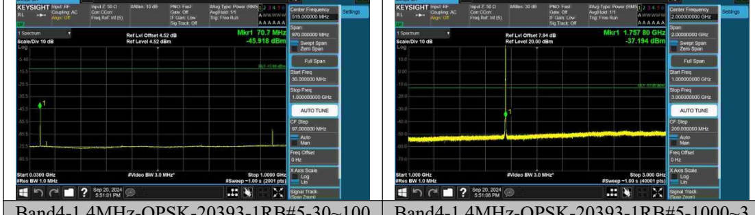
Band4-1.4MHz-QPSK-20393-1RB#5-30~1000-PASS
