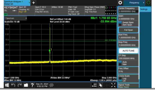
Band4-1.4MHz-QPSK-20393-6RB#0-1000~3000-PASS
