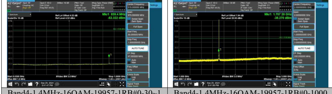
Band4-1.4MHz-16QAM-19957-1RB#0-30~1000-PASS
