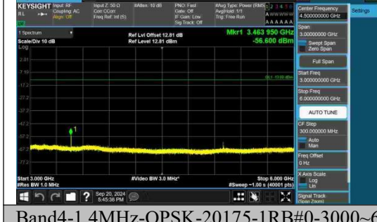
Band4-1.4MHz-QPSK-20175-1RB#0-3000~6000-PASS
