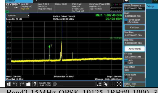
Band2-15MHz-QPSK-19125-1RB#0-1000~3000-PASS
