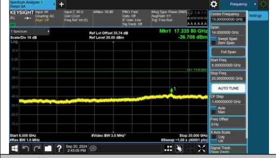
Band2-15MHz-QPSK-18900-1RB#0-6000~20000-PASS
