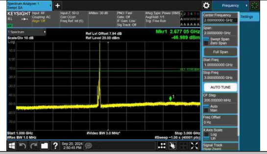
Band2-15MHz-QPSK-19125-1RB#74-1000~3000-PASS
