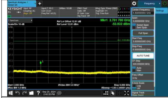
Band2-15MHz-QPSK-18675-1RB#0-3000~6000-PASS
