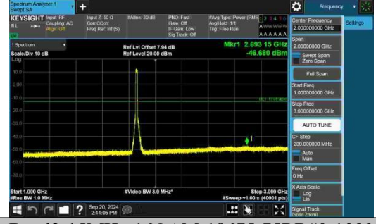
Band2-15MHz-16QAM-18675-75RB#0-1000 ~3000-PASS
