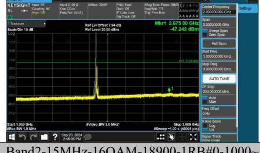
Band2-15MHz-16QAM-18900-1RB#0-1000~3000-PASS
