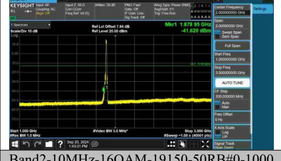
Band2-10MHz-16QAM-19150-50RB#0-1000 ~3000-PASS
