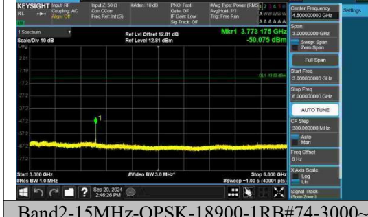
Band2-15MHz-QPSK-18900-1RB#74-3000~6000-PASS
