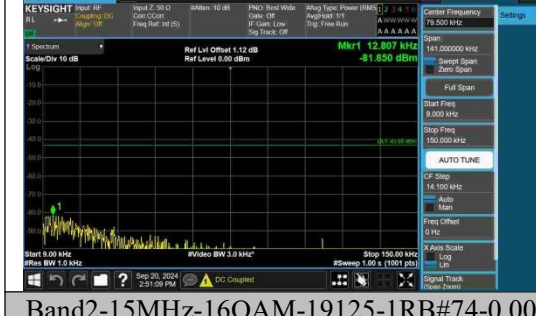
Band2-15MHz-16QAM-19125-1RB#74-0.009~0.15-PASS
