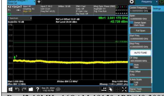
Band2-10MHz-16QAM-19150-1RB#49-3000 ~6000-PASS
