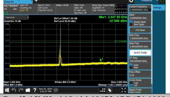
Band2-15MHz-16QAM-18675-1RB#74-1000 ~3000-PASS
