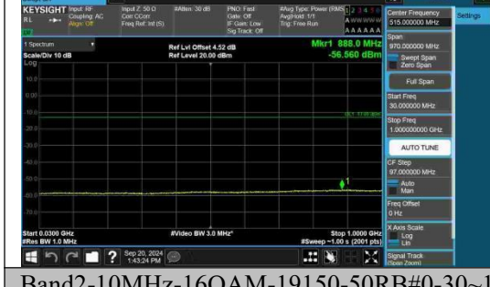
Band2-10MHz-16QAM-19150-50RB#0-30~1 000-PASS
