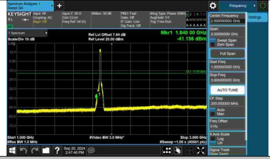
Band2-15MHz-QPSK-18900-75RB#0-1000~3000-PASS
