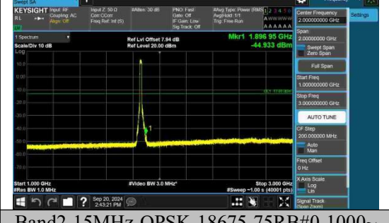
Band2-15MHz-QPSK-18675-75RB#0-1000~3000-PASS
