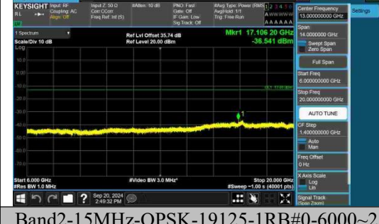
Band2-15MHz-QPSK-19125-1RB#0-6000~20000-PASS
