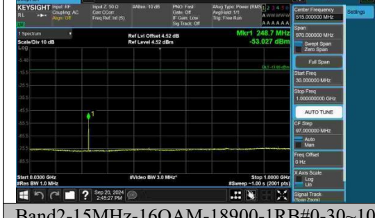
Band2-15MHz-16QAM-18900-1RB#0-30~1000-PASS
