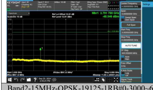
Band2-15MHz-QPSK-19125-1RB#0-3000~6000-PASS
