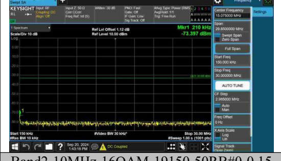
Band2-10MHz-16QAM-19150-50RB#0-0.15 ~30-PASS
