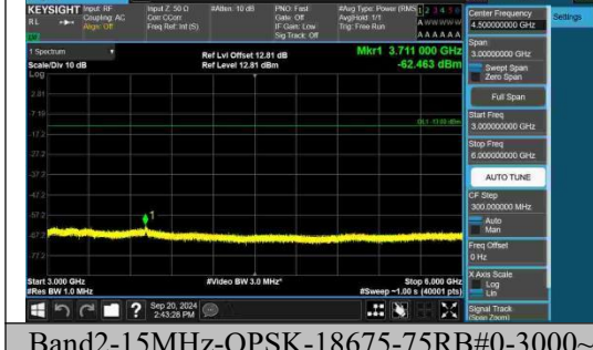
Band2-15MHz-QPSK-18675-75RB#0-3000~6000-PASS
