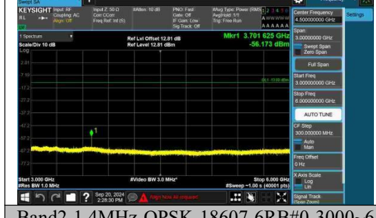
Band2-1.4MHz-QPSK-18607-6RB#0-3000~6000-PASS
