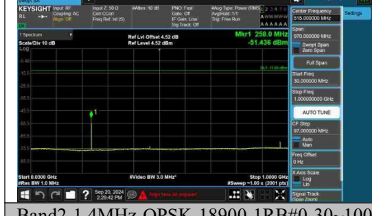
Band2-1.4MHz-QPSK-18900-1RB#0-30~1000-PASS
