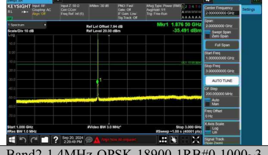
Band2-1.4MHz-QPSK-18900-1RB#0-1000~3000-PASS
