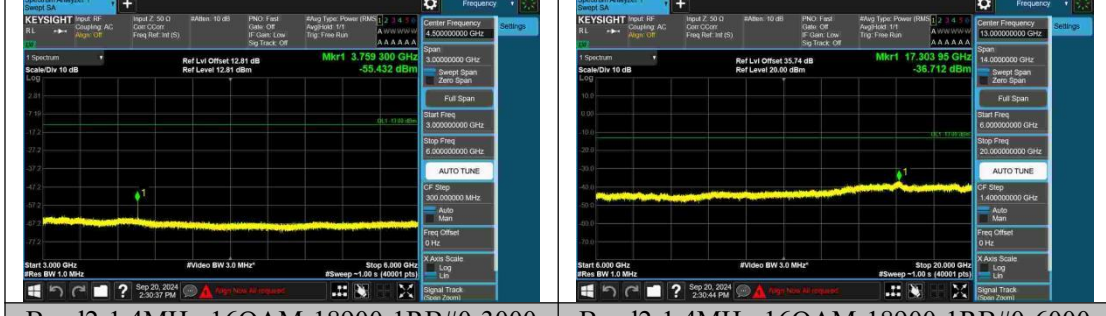
Band2-1.4MHz-16QAM-18900-1RB#0-3000 ~6000-PASS
