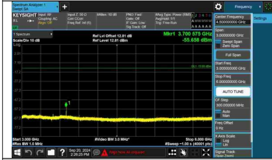
Band2-1.4MHz-16QAM-18607-1RB#0-3000~6000-PASS
