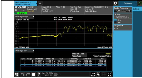
Band12-1.4MHz-QPSK-23017-6RB#0-PASS
