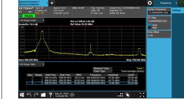
Band12-10MHz-QPSK-23060-1RB#0-PASS
