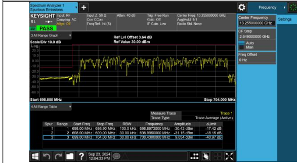
Band12-5MHz-QPSK-23035-25RB#0-PASS
