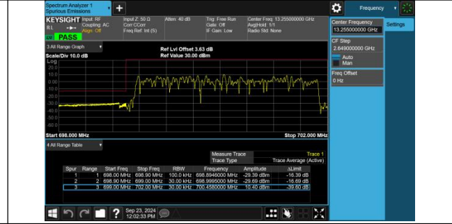
Band12-3MHz-16QAM-23025-15RB#0-PASS
