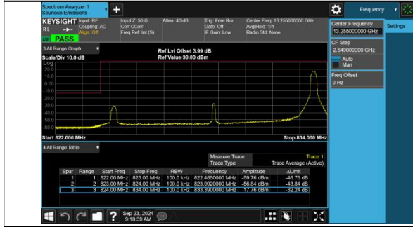
Band5-10MHz-16QAM-20450-1RB#49-PASS
