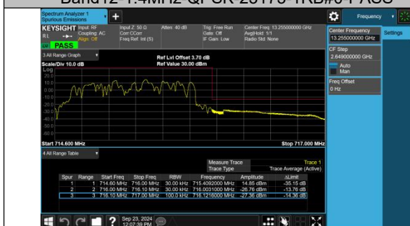
Band12-1.4MHz-QPSK-23173-6RB#0-PASS
