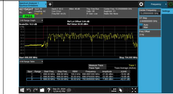
Band12-5MHz-16QAM-23035-25RB#0-PASS
