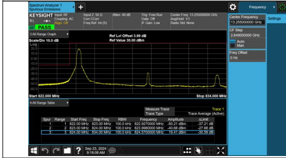
Band5-10MHz-QPSK-20450-1RB#0-PASS
