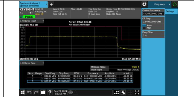
Band5-10MHz-16QAM-20600-50RB#0-PASS
