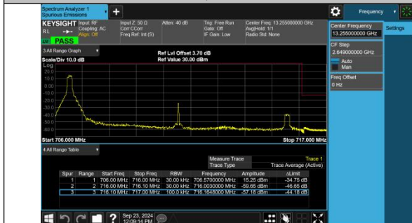
Band12-10MHz-QPSK-23130-1RB#0-PASS
