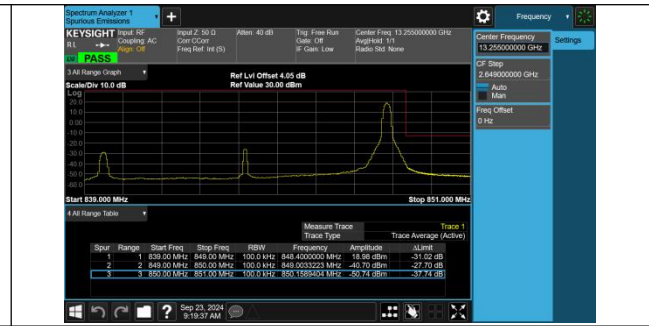
Band5-10MHz-QPSK-20600-1RB#49-PASS
