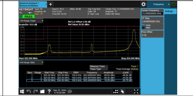
Band5-10MHz-QPSK-20450-1RB#49-PASS
