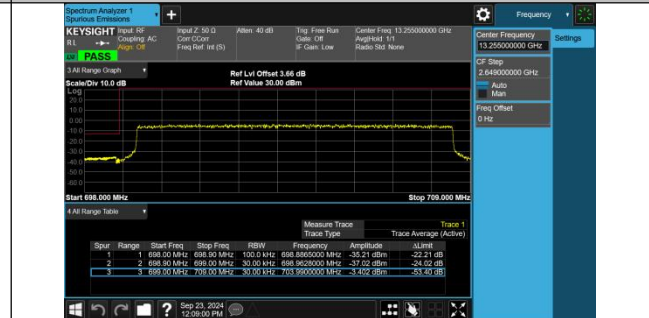
Band12-10MHz-16QAM-23060-50RB#0-PASS
