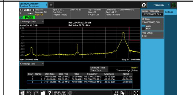
Band12-10MHz-QPSK-23130-1RB#49-PASS
