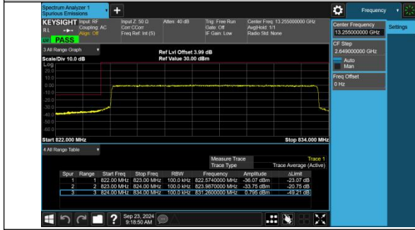
Band5-10MHz-QPSK-20450-50RB#0-PASS
