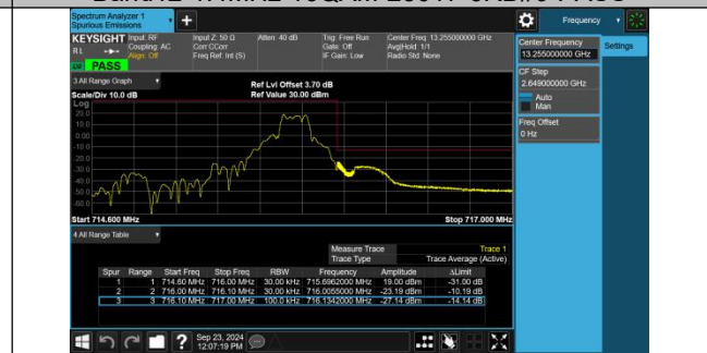
Band12-1.4MHz-QPSK-23173-1RB#5-PASS
