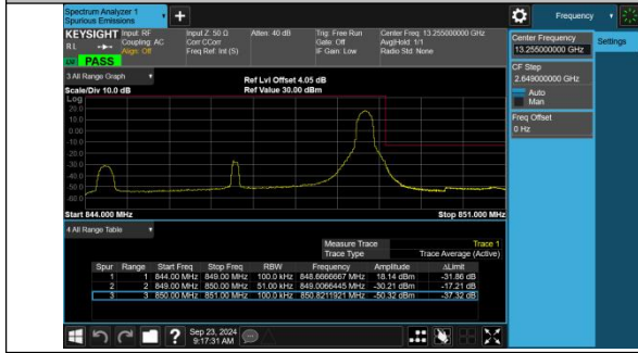
Band5-5MHz-16QAM-20625-1RB#24-PASS
