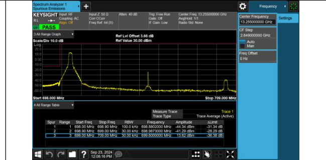
Band12-10MHz-16QAM-23060-1RB#0-PASS
