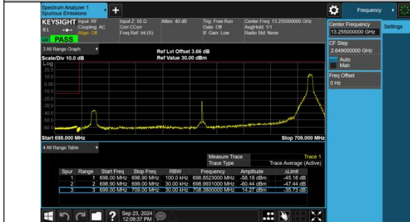
Band12-10MHz-16QAM-23060-1RB#49-PASS
