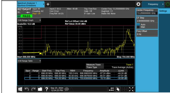
Band12-5MHz-16QAM-23035-1RB#24-PASS
