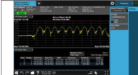
Band17-5MHz-QPSK-23755-25RB#0-PASS
