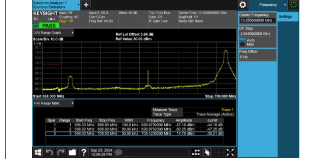
Band12-10MHz-QPSK-23060-1RB#49-PASS
