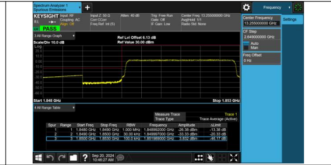
Band2-3MHz-16QAM-18615-15RB#0-PASS
