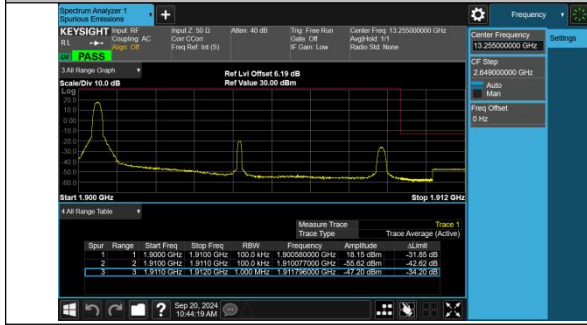
Band2-10MHz-QPSK-19150-1RB#0-PASS
