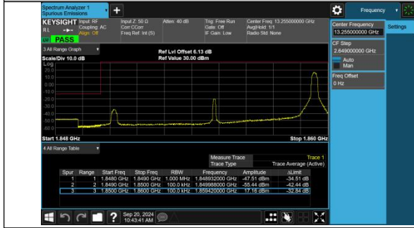
Band2-10MHz-16QAM-18650-1RB#49-PASS
