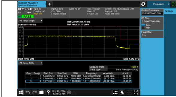
Band2-10MHz-QPSK-19150-50RB#0-PASS
