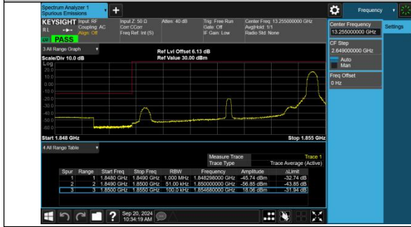
Band2-5MHz-16QAM-18625-1RB#24-PASS
