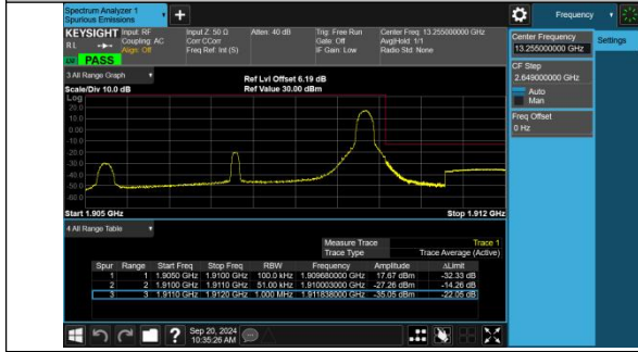
Band2-5MHz-QPSK-19175-25RB#24-PASS
