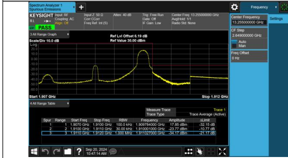
Band2-3MHz-QPSK-19185-15RB#0-PASS
