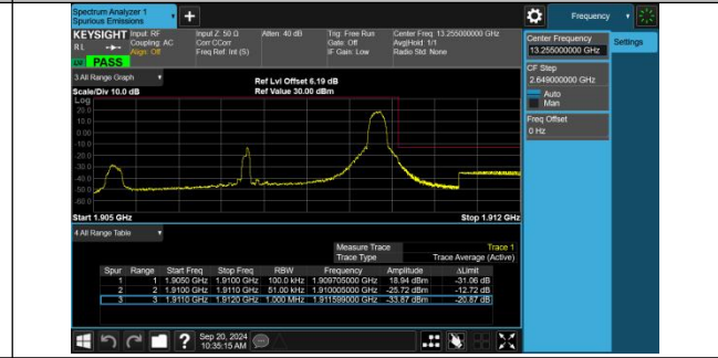
Band2-5MHz-QPSK-19175-1RB#24-PASS
