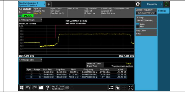
Band2-5MHz-16QAM-18625-25RB#0-PASS
