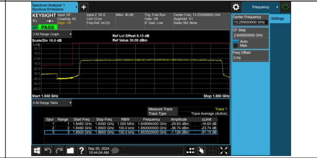
Band2-10MHz-16QAM-18650-50RB#0-PASS
