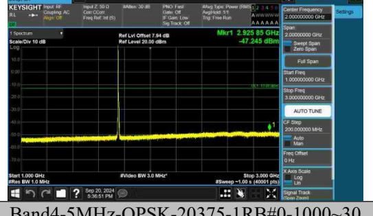
Band4-5MHz-QPSK-20375-1RB#0-1000~3000-PASS
