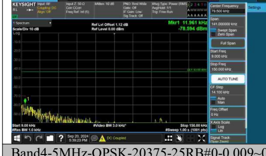
Band4-5MHz-QPSK-20375-25RB#0-0.009~0.15-PASS
