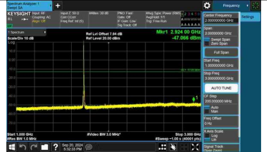
Band4-5MHz-QPSK-20175-1RB#0-1000~3000-PASS
