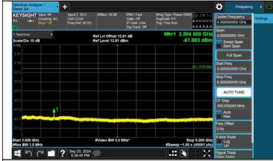
Band4-5MHz-QPSK-20375-25RB#0-3000~6 000-PASS
