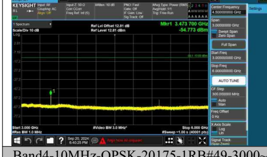
Band4-10MHz-QPSK-20175-1RB#49-3000~6000-PASS
