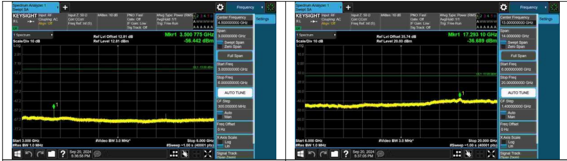
Band4-5MHz-QPSK-20375-1RB#0-3000~6000-PASS
