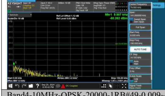
Band4-10MHz-QPSK-20000-1RB#49-0.009~0.15-PASS
