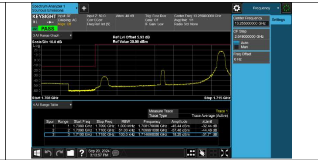
Band4-5MHz-QPSK-19975-1RB#24-PASS
