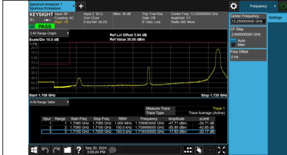
Band4-10MHz-16QAM-20000-1RB#49-PASS
