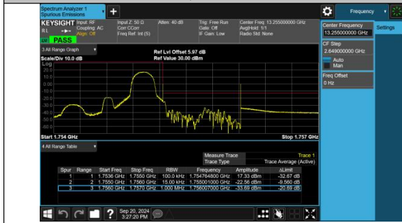
Band4-1.4MHz-16QAM-20393-1RB#5-PASS
