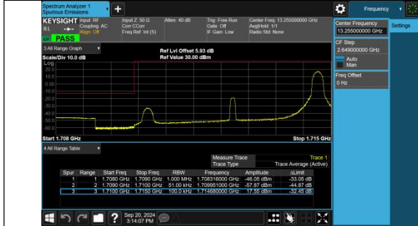
Band4-5MHz-16QAM-19975-1RB#24-PASS
