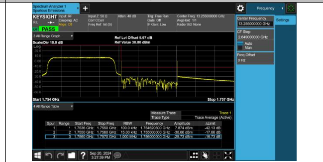
Band4-1.4MHz-16QAM-20393-6RB#0-PASS
