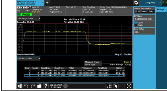
Band5-3MHz-QPSK-20635-15RB#0-PASS
