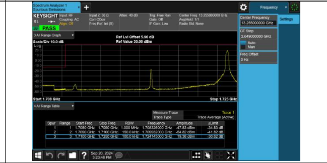
Band4-15MHz-QPSK-20025-1RB#74-PASS
