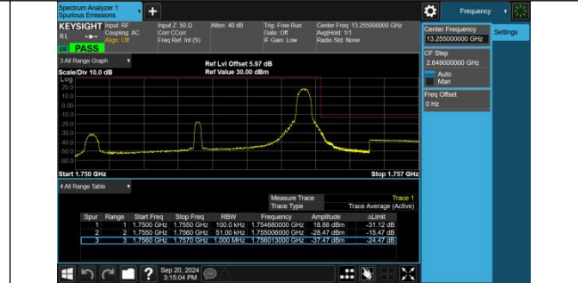
Band4-5MHz-QPSK-20375-1RB#24-PASS
