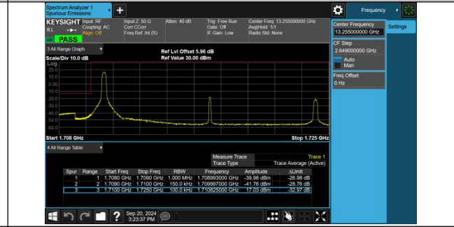
Band4-15MHz-16QAM-20025-1RB#0-PASS
