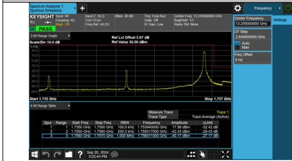
Band4-20MHz-16QAM-20300-1RB#99-PASS
