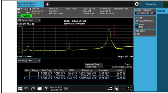
Band4-10MHz-16QAM-20350-1RB#49-PASS
