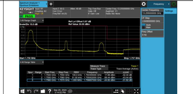
Band4-5MHz-16QAM-20375-1RB#0-PASS
