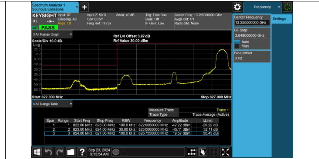
Band5-3MHz-QPSK-20415-1RB#14-PASS
