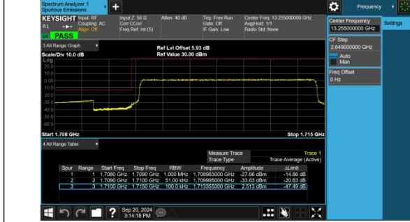
Band4-5MHz-QPSK-19975-25RB#0-PASS
