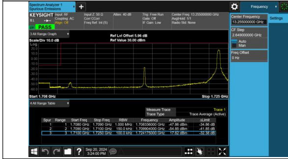
Band4-15MHz-16QAM-20025-1RB#74-PASS
