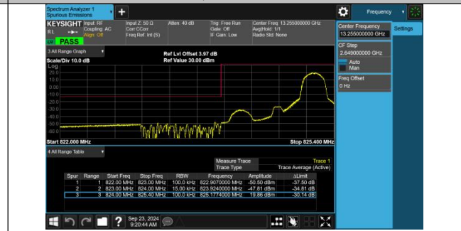
Band5-1.4MHz-QPSK-20407-1RB#5-PASS
