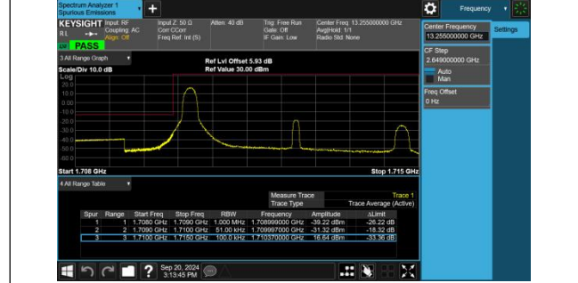
Band4-5MHz-16QAM-19975-1RB#0-PASS
