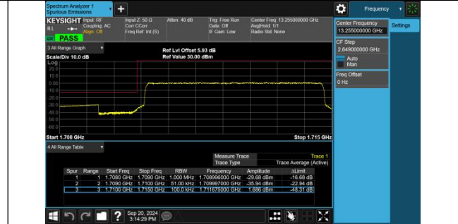
Band4-5MHz-16QAM-19975-25RB#0-PASS
