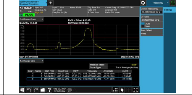
Band5-3MHz-QPSK-20635-1RB#14-PASS
