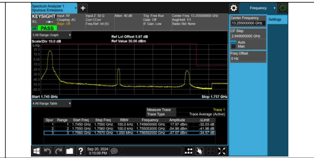
Band4-10MHz-16QAM-20350-1RB#0-PASS
