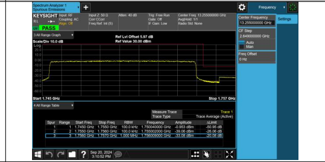
Band4-10MHz-16QAM-20350-50RB#0-PASS
