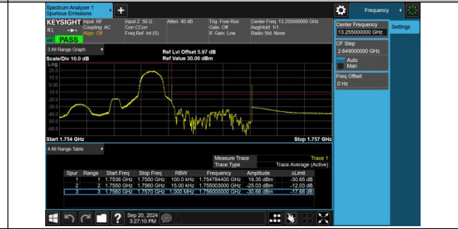
Band4-1.4MHz-QPSK-20393-1RB#5-PASS
