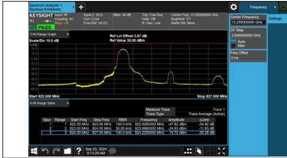
Band5-3MHz-QPSK-20415-1RB#0-PASS
