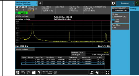
Band4-20MHz-16QAM-20050-1RB#0-PASS
