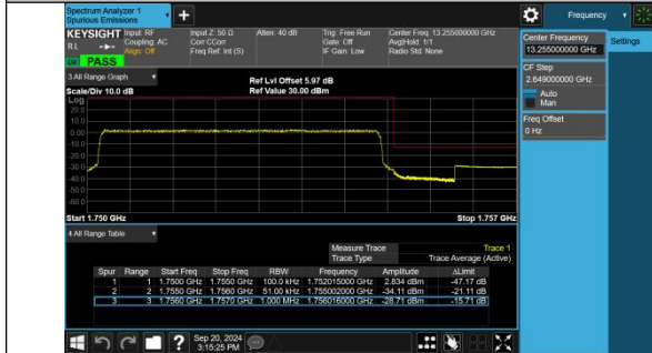
Band4-5MHz-QPSK-20375-25RB#0-PASS
