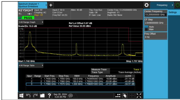
Band4-15MHz-QPSK-20325-1RB#0-PASS
