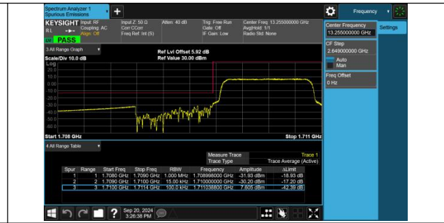
Band4-1.4MHz-16QAM-19957-6RB#0-PASS
