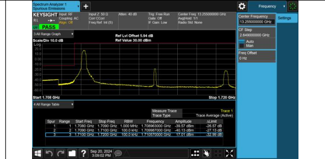
Band4-10MHz-16QAM-20000-1RB#0-PASS
