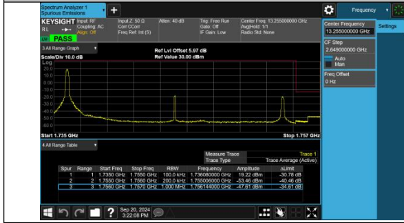
Band4-20MHz-QPSK-20300-1RB#0-PASS
