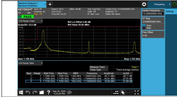
Band4-15MHz-QPSK-20025-1RB#0-PASS
