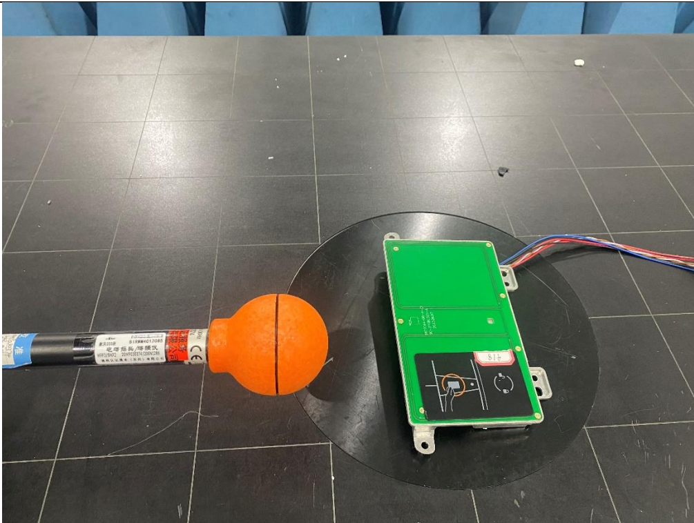
Description: RF Exposure Setup –NFC(Above 100kHz)
