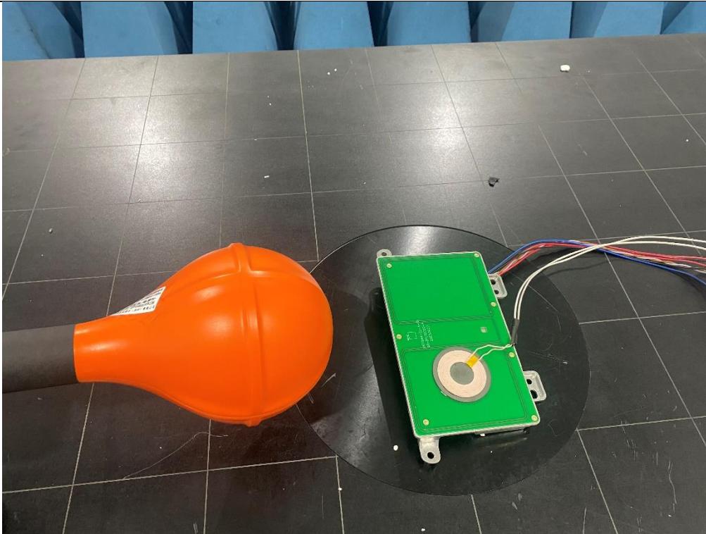
Description: RF Exposure Setup –WPT(Above 100kHz)
