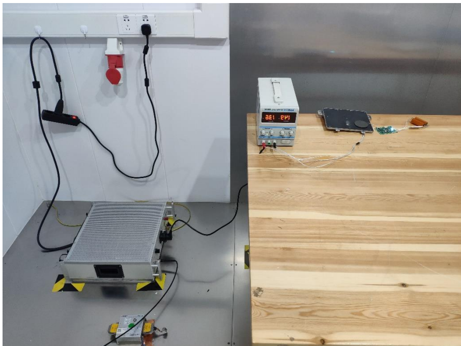
Test Photo 3
