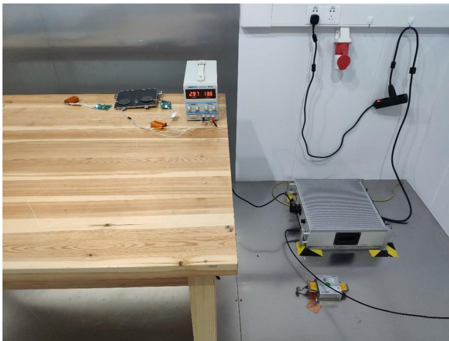
Test Photo 5
