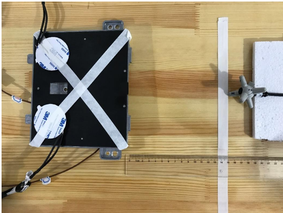
E-field Test Setup Photo Positon C Load2&3 (15cm)
