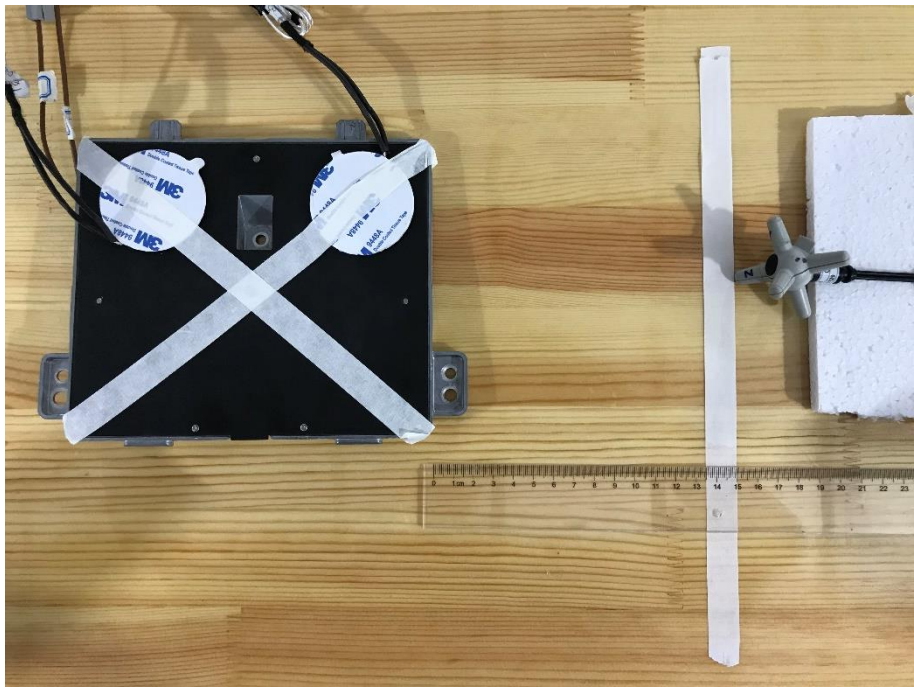
E-field Test Setup Photo Positon D Load2&3 (15cm)
