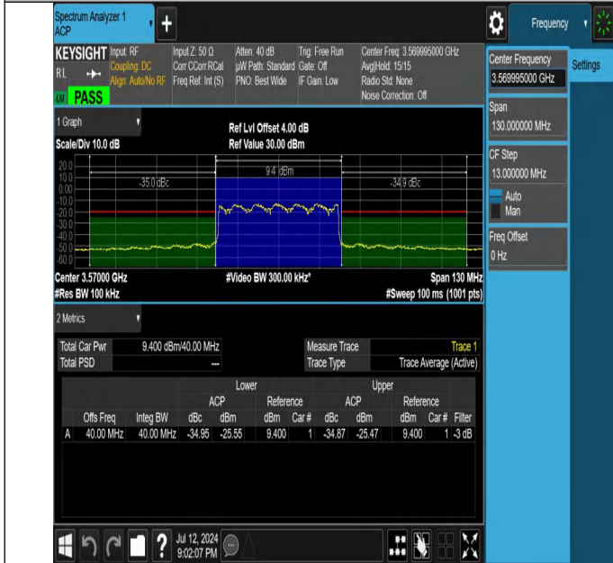
NTNV-N48-PC3-30-40-L-CP-64QAM-Outer_Full-Ant1-PASS
