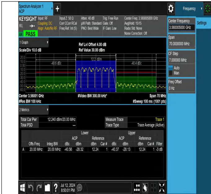
NTNV-N48-PC3-30-20-L-DFT-QPSK-Outet_Full-Ant1-PASS
