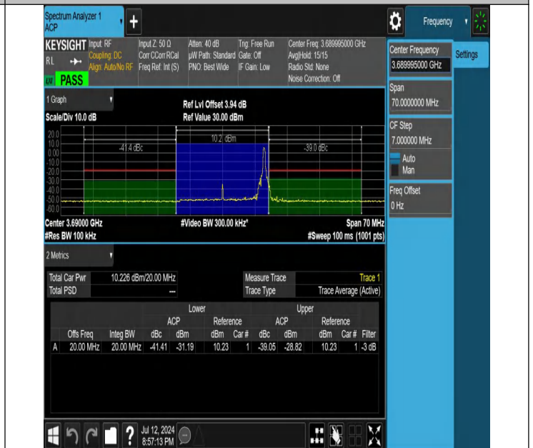
NTNV-N48-PC3-30-20-H-CP-16QAM-Edge_1RB_Right-Ant1-PAS
