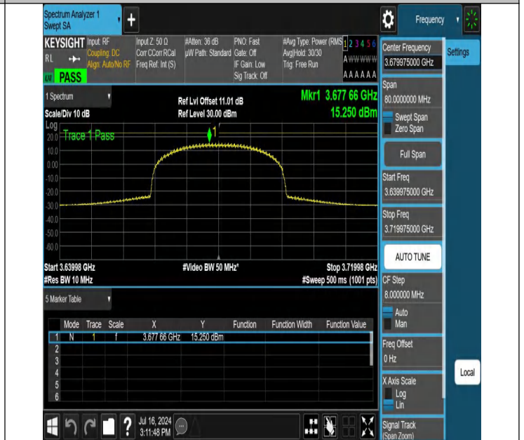
NTNV-N48-PC3-30-40-H-CP-64QAM-Inner_Full-3639.975-3719.975-Ant1-PASS
