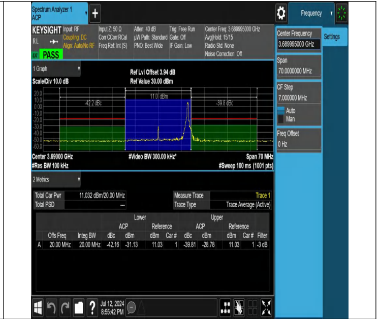
NTNV-N48-PC3-30-20-H-DFT-64QAM-Edge_1RB_Right-Ant1-PA SS
