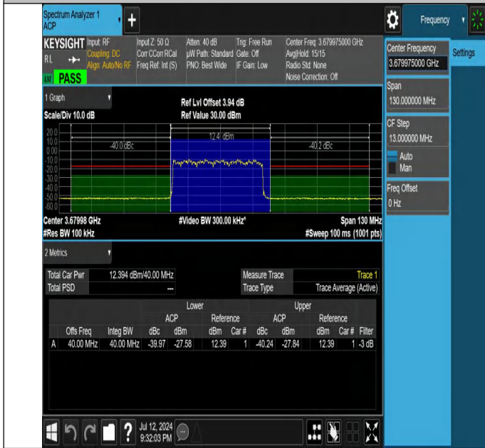
NTNV-N48-PC3-30-40-H-DFT-PI2BPSK-Outer_Full-Ant1-PASS
