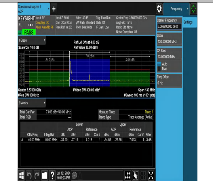
NTNV-N48-PC3-30-40-L-CP-QPSK-Edge_1RB_Left-Ant1-PASS
