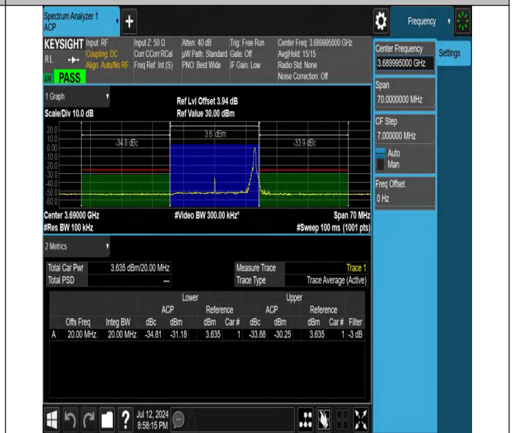
NTNV-N48-PC3-30-20-H-CP-256QAM-Edge_1RB_Right-Ant1-PASS
