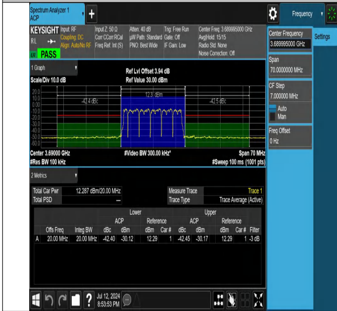
NTNV-N48-PC3-30-20-H-DFT-PI2BPSK-Outer_Full-Ant1-PASS
