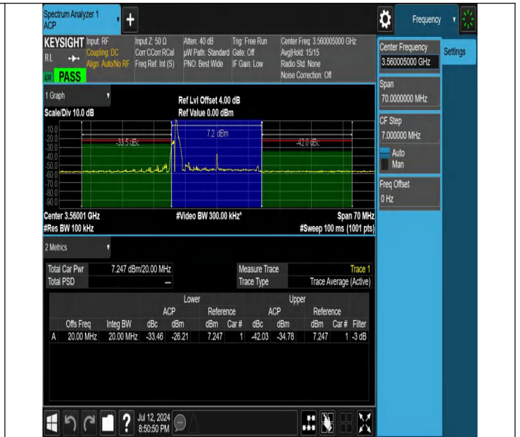
NTNV-N48-PC3-30-20-L-DFT-16QAM-Edge_1RB_Left-Ant1-PASS
