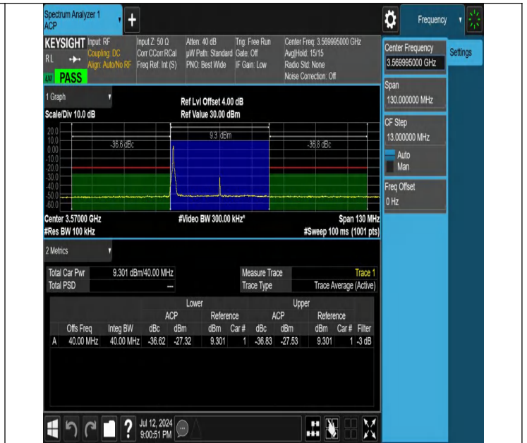
NTNV-N48-PC3-30-40-L-DFT-256QAM-Edge_1RB_Left-Ant1-PA SS
