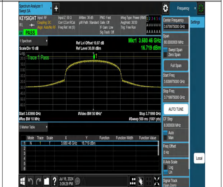
NTNV-N48-PC3-30-40-H-CP-16QAM-Inner_Full-3639.975-3719.975-Ant1-PASS
