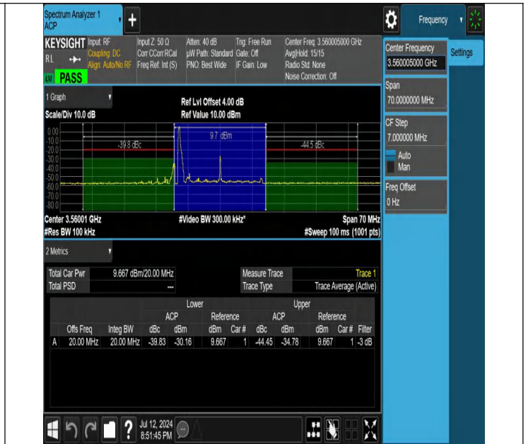
NTNV-N48-PC3-30-20-L-DFT-256QAM-Edge_1RB_Left-Ant1-PA SS
