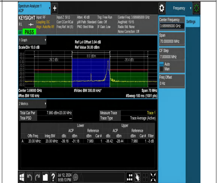
NTNV-N48-PC3-30-20-H-DFT-16QAM-Edge_1RB_Right-Ant1-PASS
