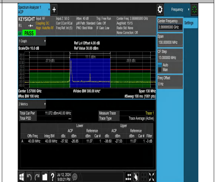
NTNV-N48-PC3-30-40-L-DFT-64QAM-Edge_1RB_Left-Ant1-PASS
