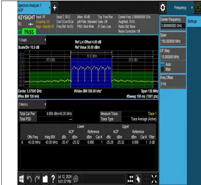
NTNV-N48-PC3-30-40-L-CP-16QAM-Outer_Full-Ant1-PASS
