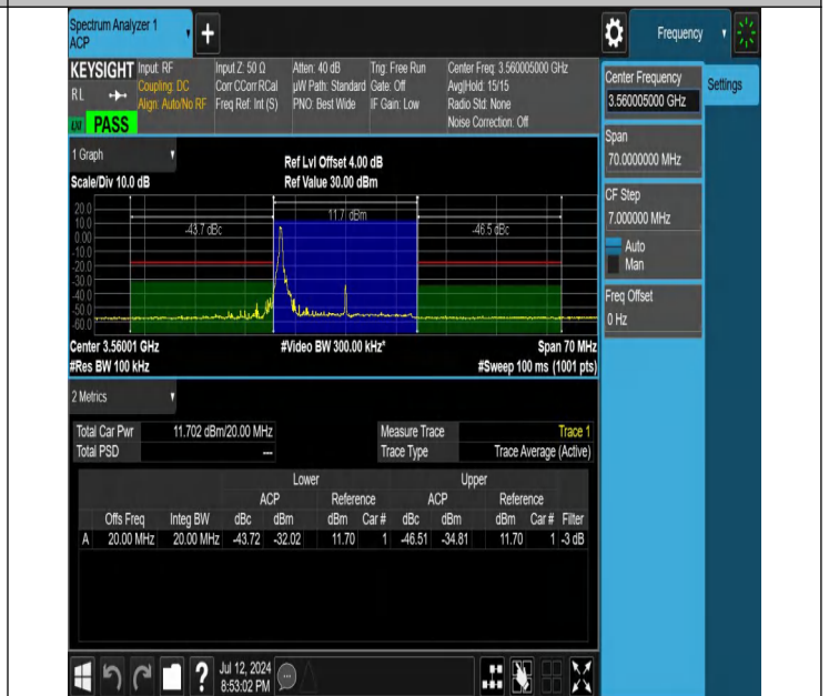
NTNV-N48-PC3-30-20-L-CP-64QAM-Edge_1RB_Left-Ant1-PASS
