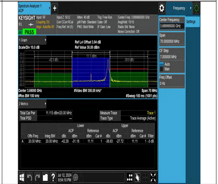
NTNV-N48-PC3-30-20-H-DFT-PI2BPSK-Edge_1RB_Right-Ant1-PASS
