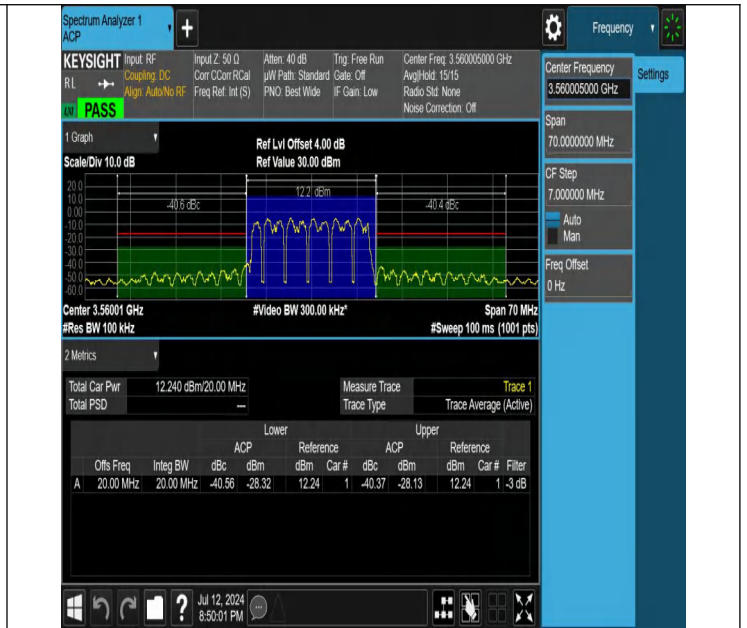
NTNV-N48-PC3-30-20-L-DFT-QPSK-Outet_Full-Ant1-PASS
