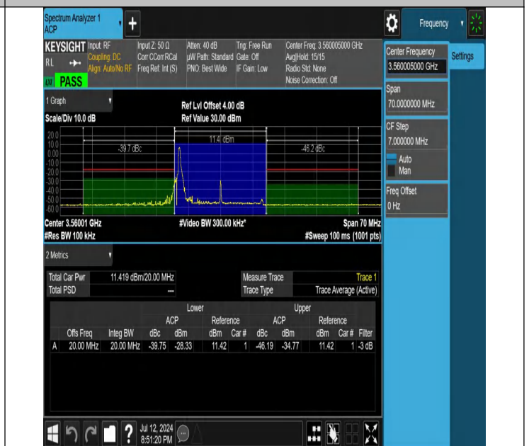
NTNV-N48-PC3-30-20-L-DFT-64QAM-Edge_1RB_Left-Ant1-PASS
