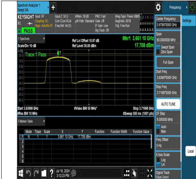
NTNV-N48-PC3-30-40-H-CP-64QAM-Edge_1RB_Left-3639.975-3719.975-Ant1-PASS
