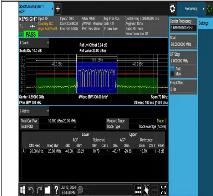
NTNV-N48-PC3-30-20-H-DFT-16QAM-Outer_Full-Ant1-PASS
