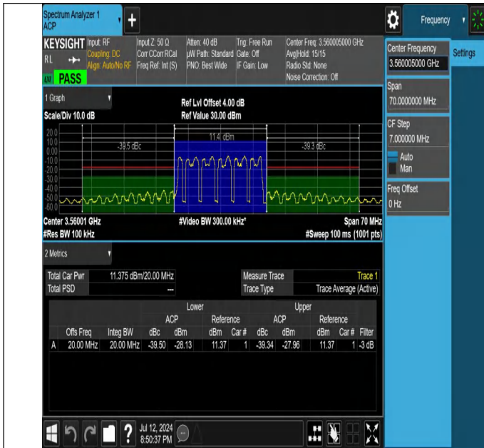
NTNV-N48-PC3-30-20-L-DFT-16QAM-Outer_Full-Ant1-PASS
