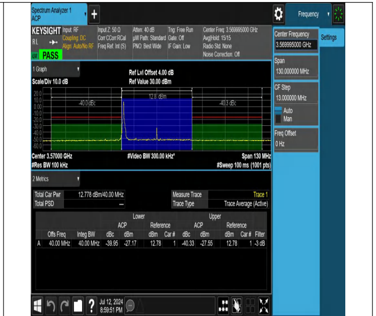
NTNV-N48-PC3-30-40-L-DFT-16QAM-Edge_1RB_Left-Ant1-PASS
