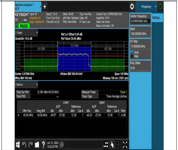
NTNV-N48-PC3-30-40-H-DFT-PI2BPSK-Outer_Full-Ant1-PASS
