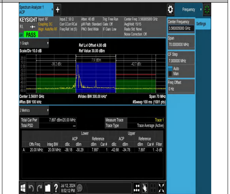
NTNV-N48-PC3-30-20-L-CP-QPSK-Edge_1RB_Left-Ant1-PASS
