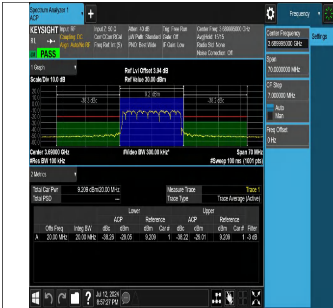
NTNV-N48-PC3-30-20-H-CP-64QAM-Outer_Full-Ant1-PASS
