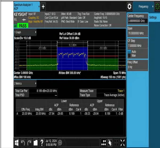
NTNV-N48-PC3-30-20-H-DFT-256QAM-Outer_Full-Ant1-PASS
