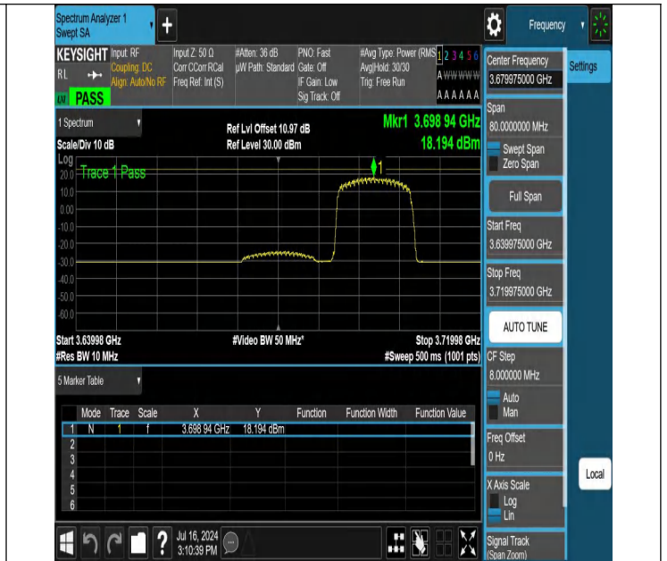
NTNV-N48-PC3-30-40-H-CP-16QAM-Edge_1RB_Right-3639.975-3719.975-Ant1-PASS
