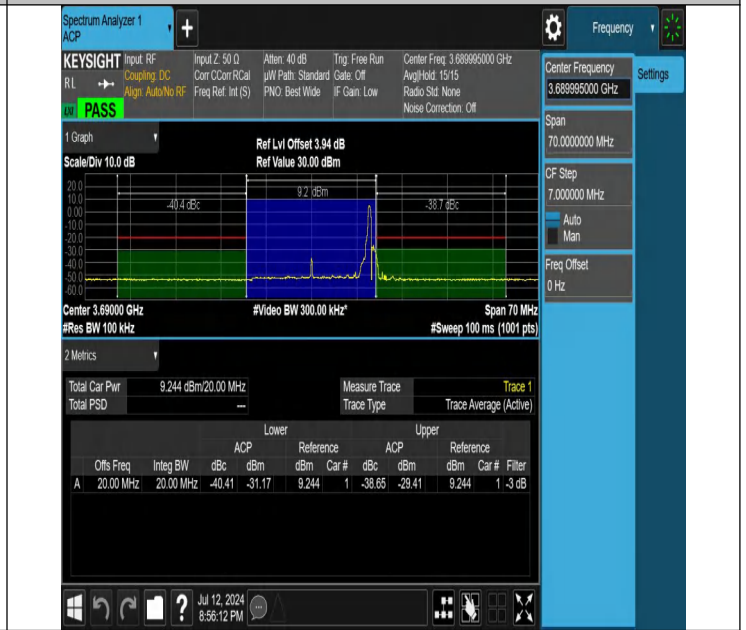
NTNV-N48-PC3-30-20-H-DFT-256QAM-Edge_1RB_Right-Ant1-PASS
