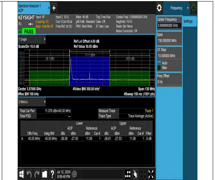
NTNV-N48-PC3-30-40-L-DFT-PI2BPSK-Edge_1RB_Left-Ant1-PA SS
