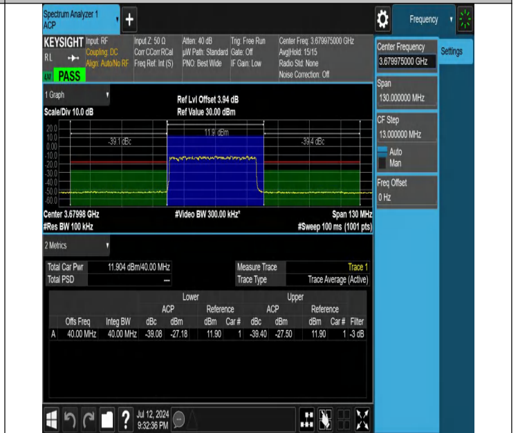
NTNV-N48-PC3-30-40-H-DFT-QPSK-Outer_Full-Ant1-PASS
