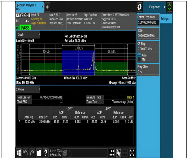
NTNV-N48-PC3-30-20-H-CP-QPSK-Edge_1RB_Right-Ant1-PASS
