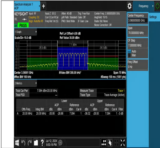
NTNV-N48-PC3-30-20-L-CP-256QAM-Outer_Full-Ant1-PASS
