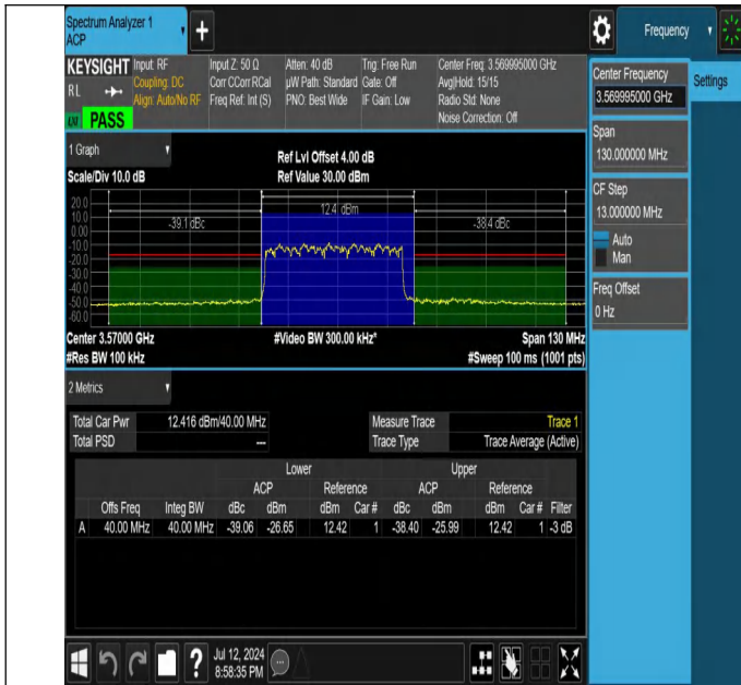
NTNV-N48-PC3-30-40-L-DFT-PI2BPSK-Outer_Full-Ant1-PASS
