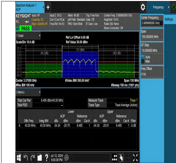
NTNV-N48-PC3-30-40-L-DFT-256QAM-Outer_Full-Ant1-PASS
