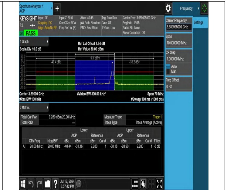
NTNV-N48-PC3-30-20-H-CP-64QAM-Edge_1RB_Right-Ant1-PASS
