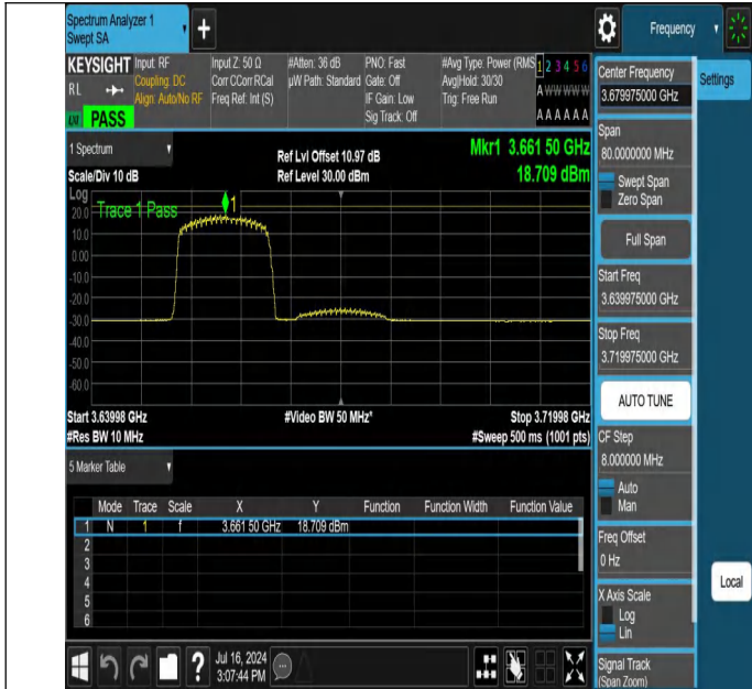
NTNV-N48-PC3-30-40-H-CP-QPSK-Edge_1RB_Left-3639.975-3719.975-Ant1-PASS
