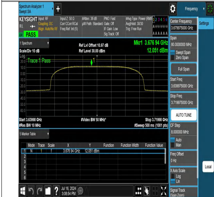
NTNV-N48-PC3-30-40-H-CP-16QAM-Outer_Full-3639.975-3719.975-Ant1-PASS
