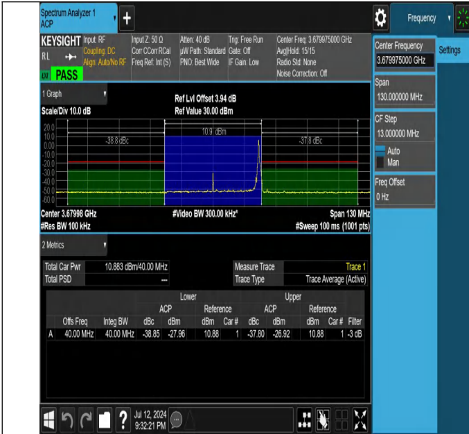
NTNV-N48-PC3-30-40-H-DFT-PI2BPSK-Edge_1RB_Right-Ant1-P
