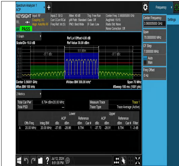
NTNV-N48-PC3-30-20-L-DFT-256QAM-Outer_Full-Ant1-PASS
