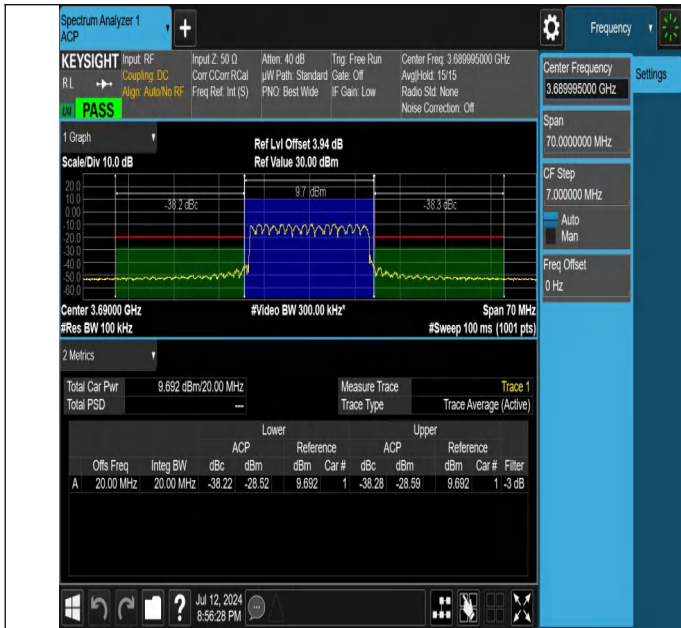
NTNV-N48-PC3-30-20-H-CP-QPSK-Outer_Full-Ant1-PASS
