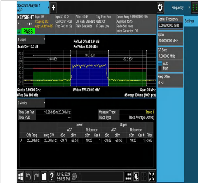
NTNV-N48-PC3-30-20-H-DFT-64QAM-Outer_Full-Ant1-PASS
