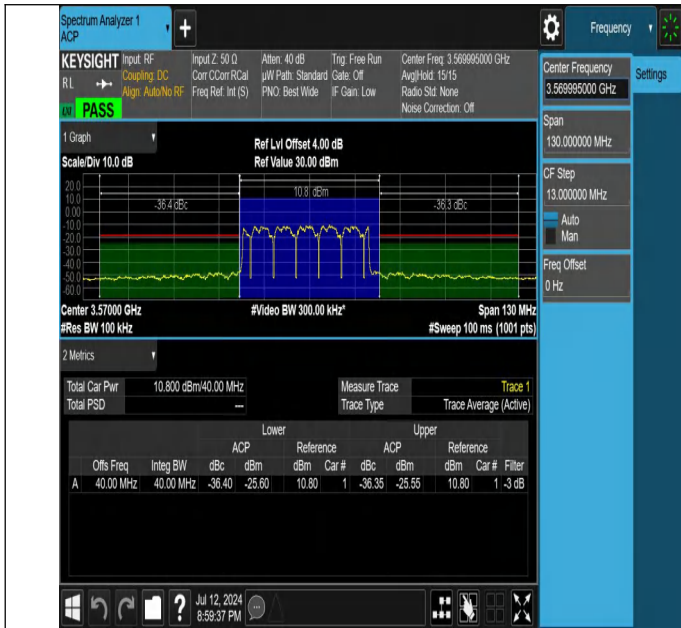
NTNV-N48-PC3-30-40-L-DFT-16QAM-Outer_Full-Ant1-PASS
