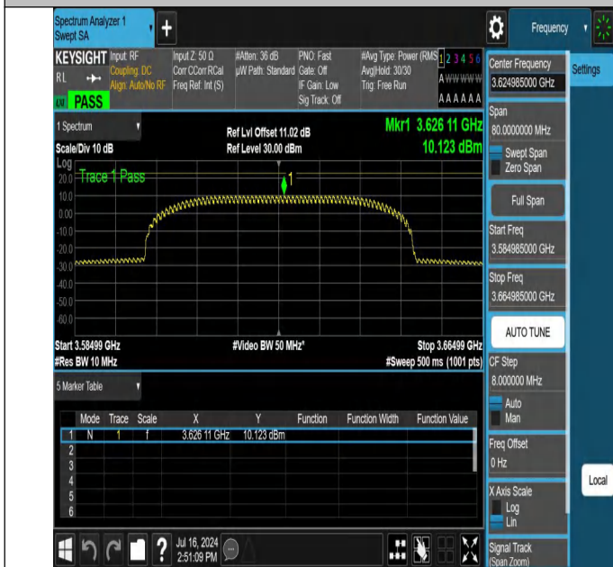
NTNV-N48-PC3-30-40-M-CP-256QAM-Outer_Full-3584.985-3664.985-Ant1-PASS
