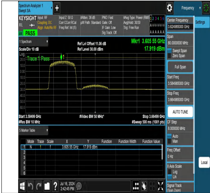
NTNV-N48-PC3-30-40-M-DFT-256QAM-Edge_1RB_Left-3584.985-3664.985-Ant1-PASS
