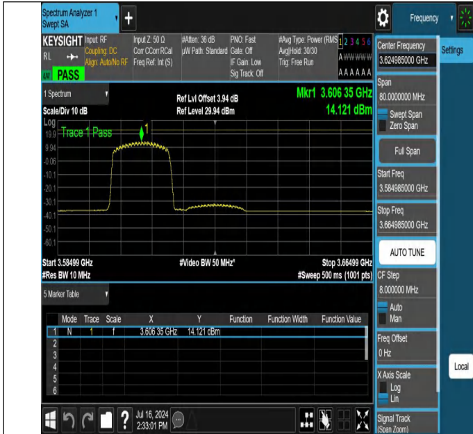
NTNV-N48-PC3-30-40-M-DFT-PI2BPSK-Edge_1RB_Left-3584.985-3664.985-Ant1-PASS
