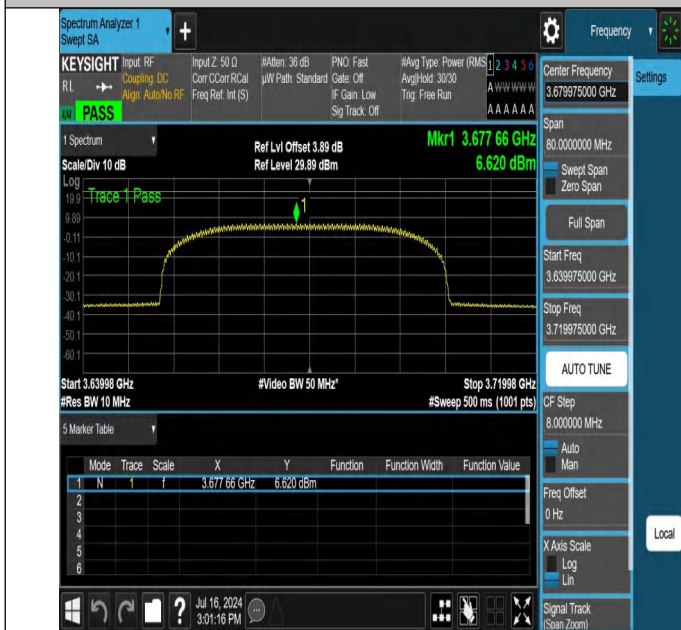
NTNV-N48-PC3-30-40-H-DFT-64QAM-Outer_Full-3639.975-3719.975-Ant1-PASS
