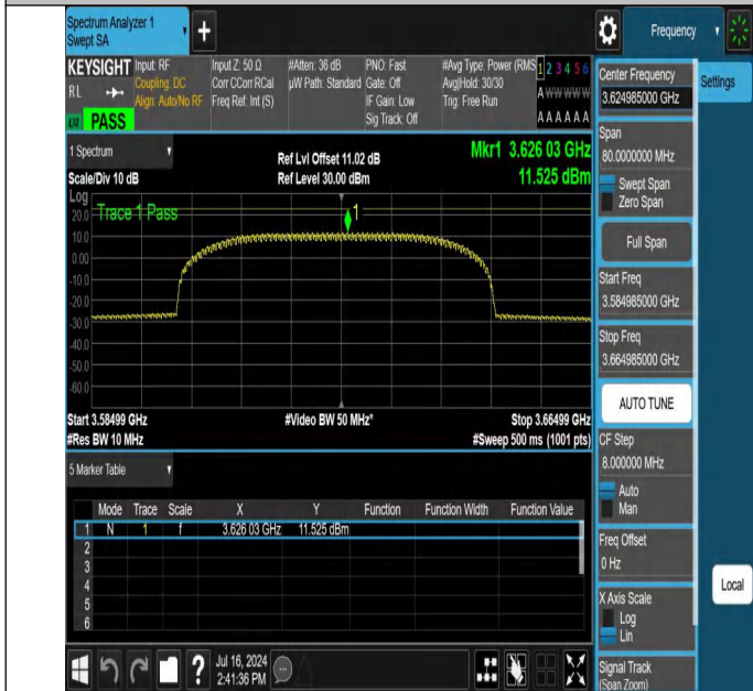
NTNV-N48-PC3-30-40-M-DFT-256QAM-Outer_Full-3584.985-3664.985-Ant1-PASS
