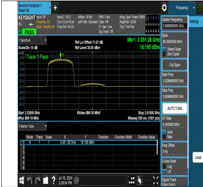
NTNV-N48-PC3-30-40-L-CP-64QAM-Edge_1RB_Left-3529.995-3609.995-Ant1-PASS
