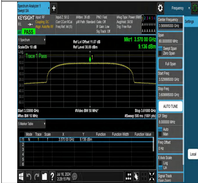
NTNV-N48-PC3-30-40-L-CP-256QAM-Outer_Full-3529.995-3609.995-Ant1-PASS
