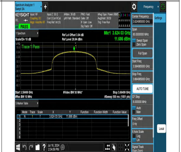
NTNV-N48-PC3-30-40-M-DFT-QPSK-Inner_Full-3584.985-3664.985-Ant1-PASS
