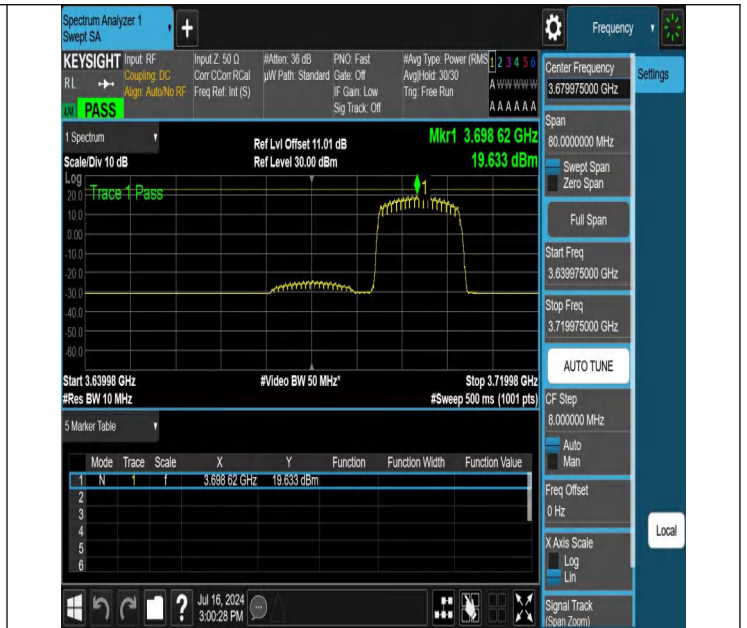
NTNV-N48-PC3-30-40-H-DFT-16QAM-Edge_1RB_Right-3639.975-3719.975-Ant1-PASS
