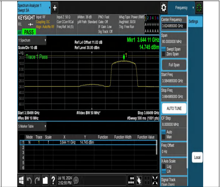
NTNV-N48-PC3-30-40-M-CP-256QAM-Edge_1RB_Right-3584.985-3664.985-Ant1-PASS
