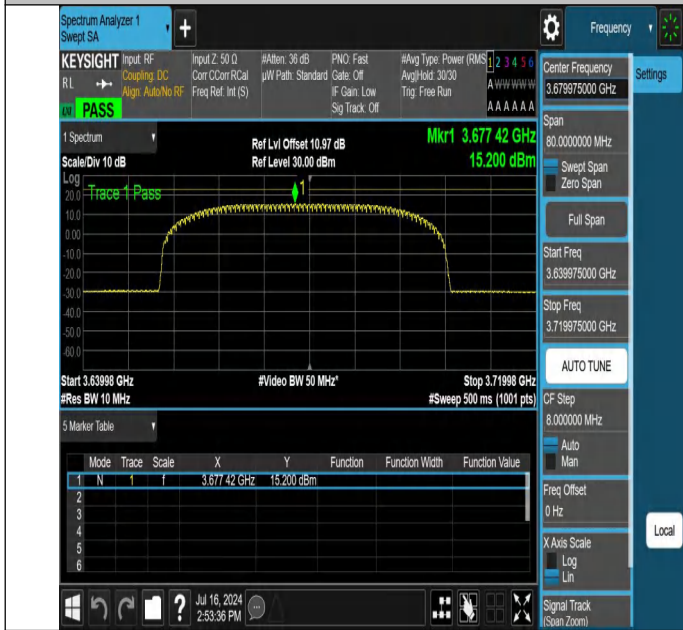
NTNV-N48-PC3-30-40-H-DFT-PI2BPSK-Outer_Full-3639.975-3719.975-Ant1-PASS
