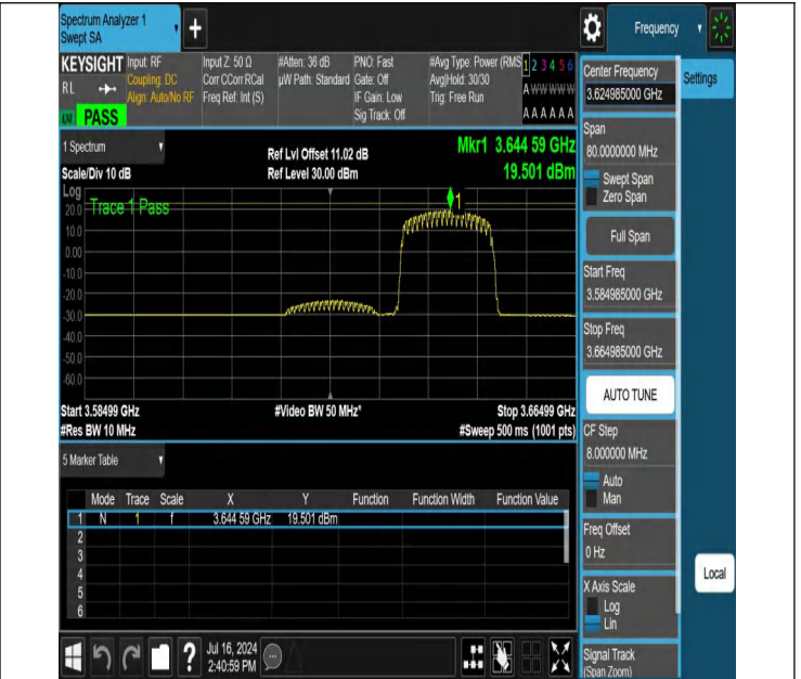
NTNV-N48-PC3-30-40-M-DFT-64QAM-Edge_1RB_Right-3584.985-3664.985-Ant1-PASS
