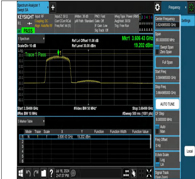
NTNV-N48-PC3-30-40-M-CP-16QAM-Edge_1RB_Left-3584.985-3664.985-Ant1-PASS
