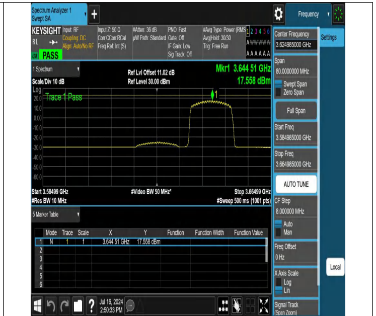
NTNV-N48-PC3-30-40-M-CP-64QAM-Edge_1RB_Right-3584.985-3664.985-Ant1-PASS
