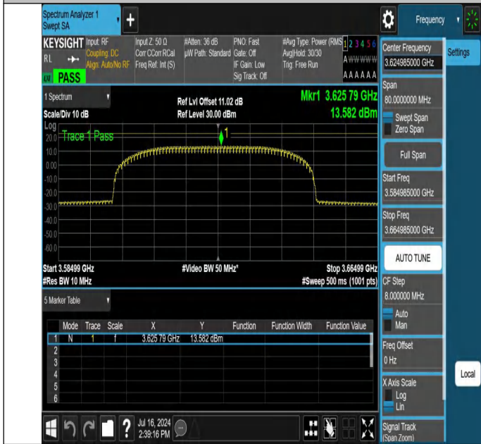
NTNV-N48-PC3-30-40-M-DFT-64QAM-Outer_Full-3584.985-3664.985-Ant1-PASS
