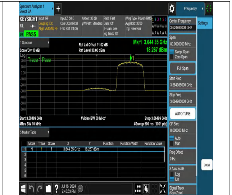
NTNV-N48-PC3-30-40-M-CP-QPSK-Edge_1RB_Right-3584.985-3664.985-Ant1-PASS
