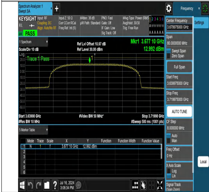
NTNV-N48-PC3-30-40-H-CP-QPSK-Outer_Full-3639.975-3719.975-Ant1-PASS
