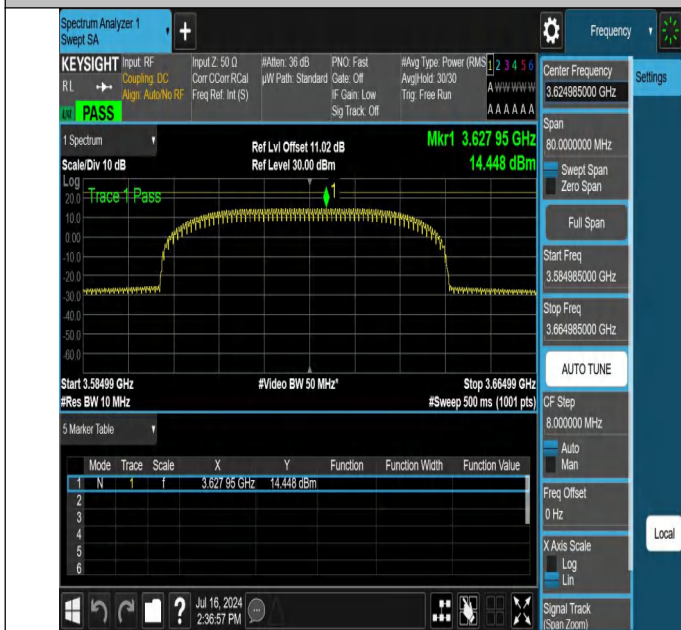
NTNV-N48-PC3-30-40-M-DFT-16QAM-Outer_Full-3584.985-3664.985-Ant1-PASS
