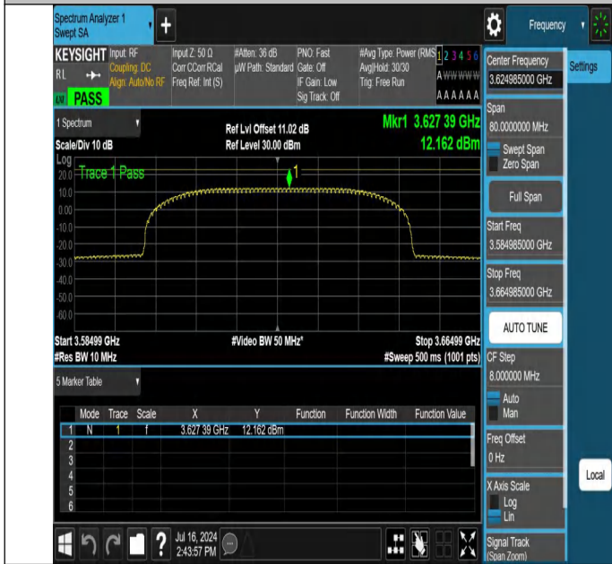
NTNV-N48-PC3-30-40-M-CP-QPSK-Outer_Full-3584.985-3664.985-Ant1-PASS
