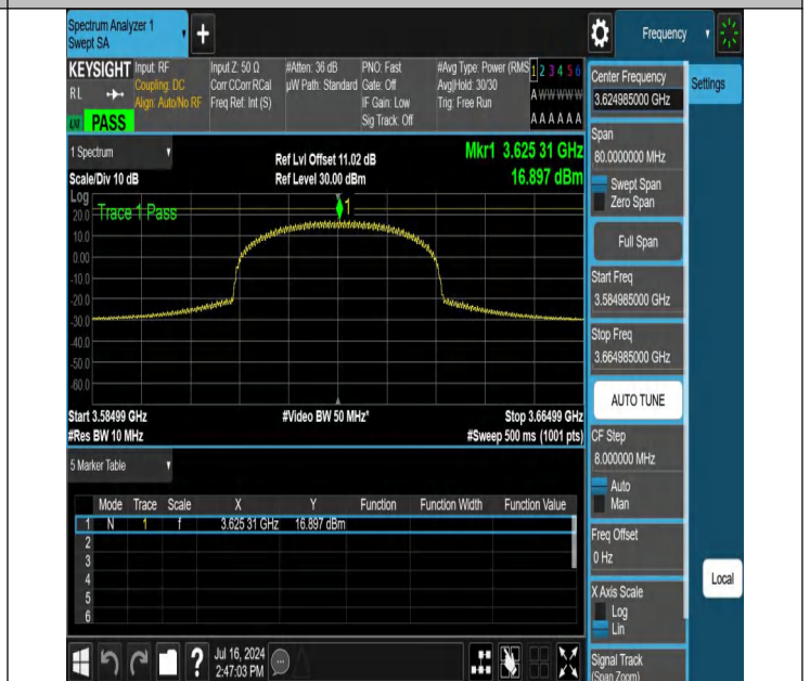
NTNV-N48-PC3-30-40-M-CP-16QAM-Inner_Full-3584.985-3664.985-Ant1-PASS
