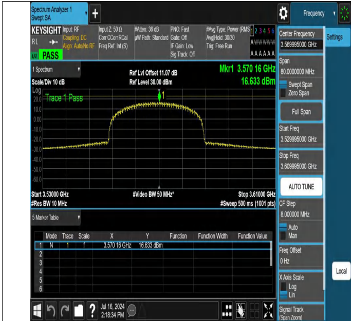
NTNV-N48-PC3-30-40-L-DFT-64QAM-Inner_Full-3529.995-3609.995-Ant1-PASS
