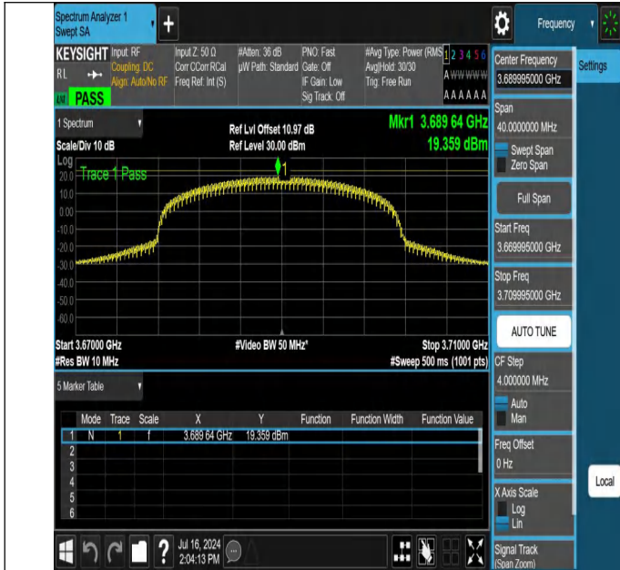
NTNV-N48-PC3-30-20-H-CP-16QAM-Inner_Full-3669.995-3709.995-Ant1-PASS
