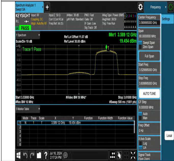
NTNV-N48-PC3-30-40-L-DFT-16QAM-Edge_1RB_Right-3529.995-3609.995-Ant1-PASS
