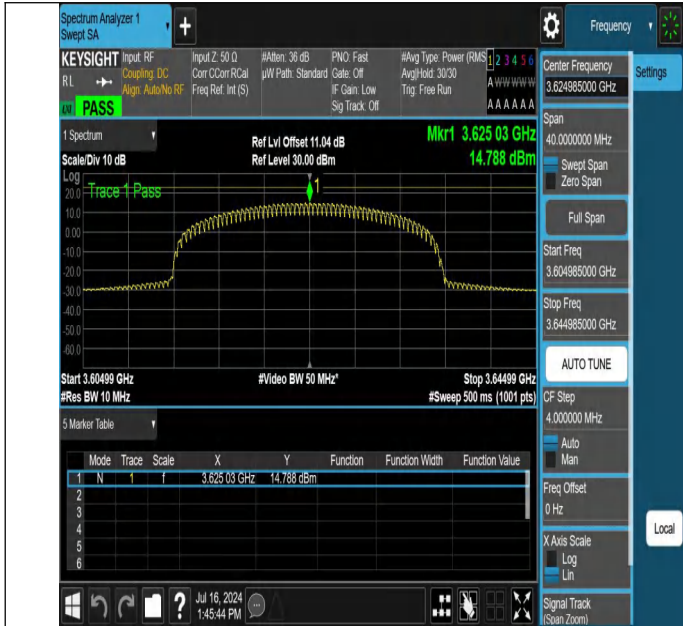
NTNV-N48-PC3-30-20-M-CP-256QAM-Inner_Full-3604.985-3644.985-Ant1-PASS
