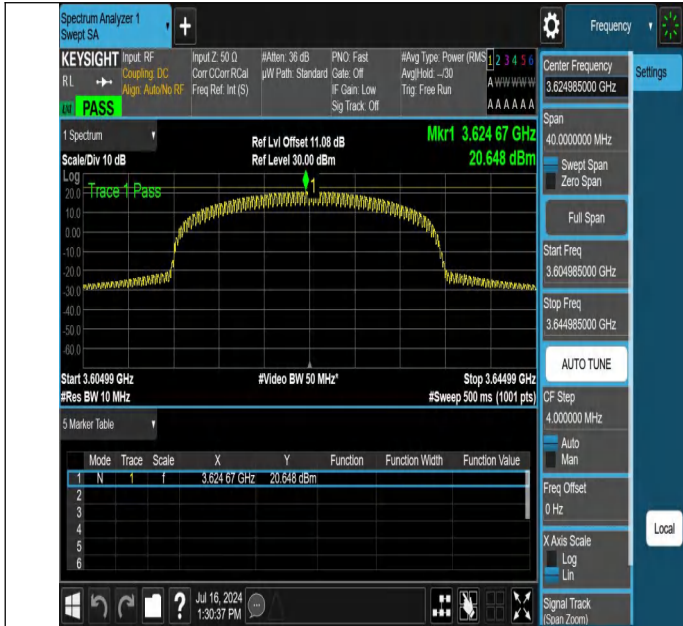
NTNV-N48-PC3-30-20-M-DFT-16QAM-Inner_Full-3604.985-3644.985-Ant1-PASS
