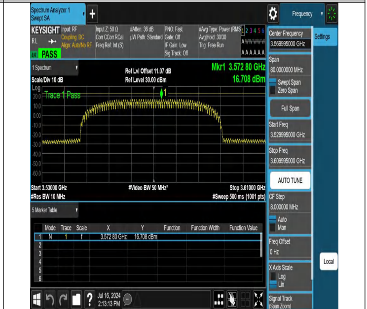
NTNV-N48-PC3-30-40-L-DFT-QPSK-Outer_Full-3529.995-3609.995-Ant1-PASS
