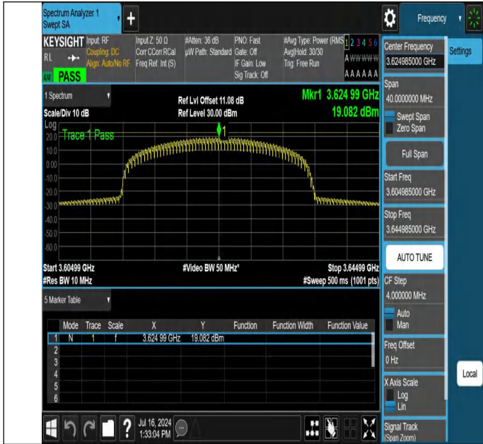
NTNV-N48-PC3-30-20-M-DFT-64QAM-Inner_Full-3604.985-3644.
