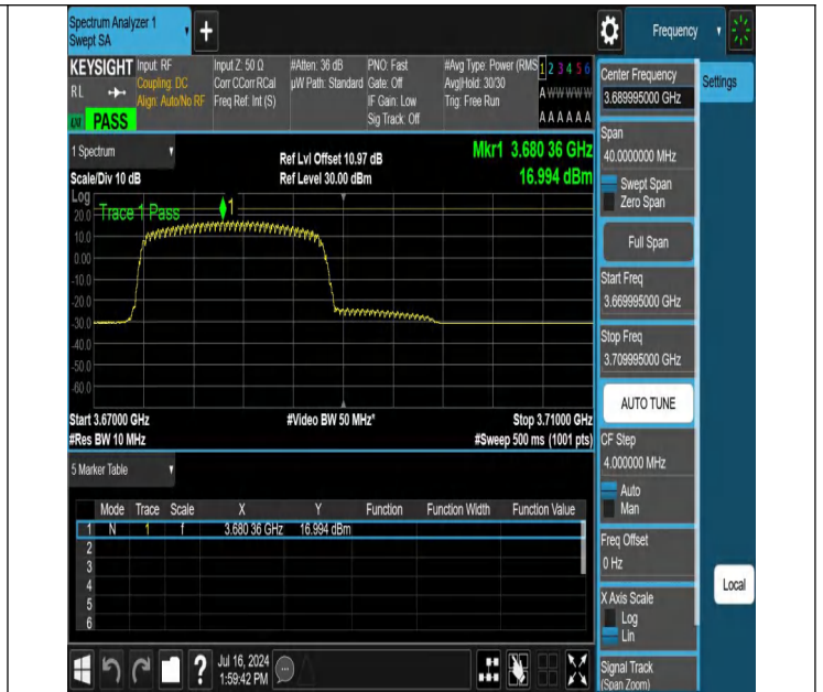
NTNV-N48-PC3-30-20-H-DFT-256QAM-Edge_1RB_Left-3669.995-3709.995-Ant1-PASS
