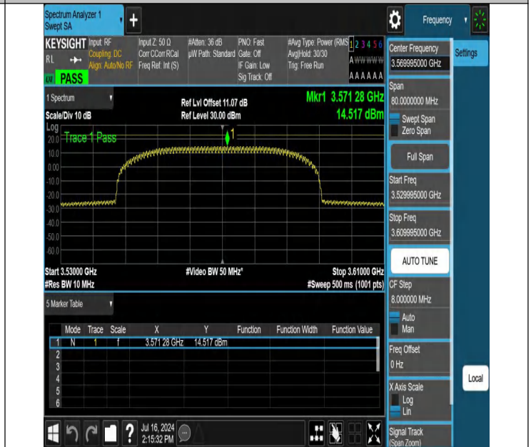
NTNV-N48-PC3-30-40-L-DFT-16QAM-Outer_Full-3529.995-3609.995-Ant1-PASS
