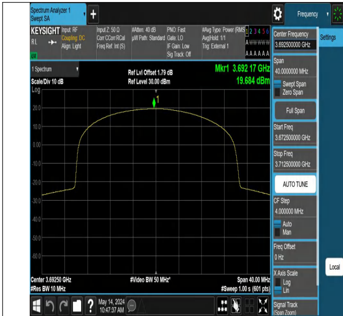
Band48-15MHz-QPSK-56665-75RB#0-PASS
