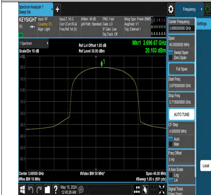
Band48-10MHz-16QAM-56690-25RB#25-PASS
