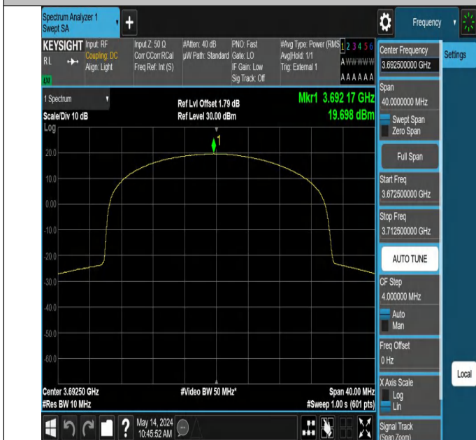
Band48-15MHz-QPSK-56665-38RB#37-PASS
