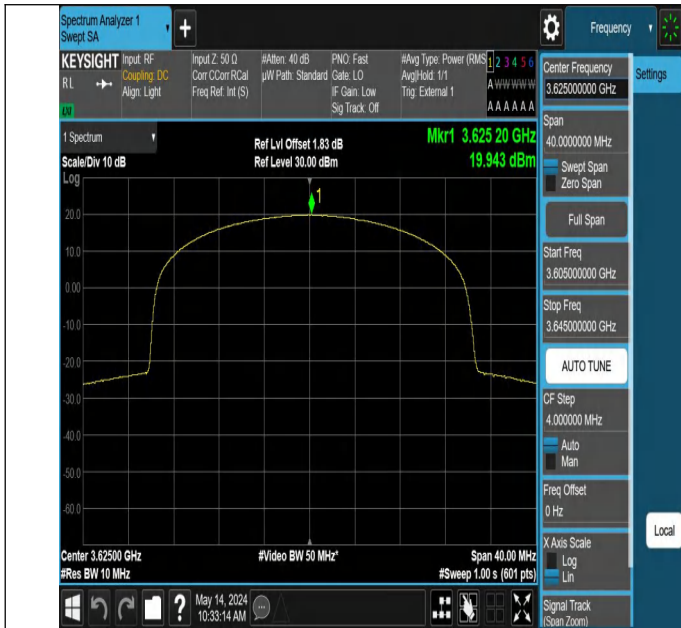
Band48-15MHz-256QAM-55990-38RB#18-PASS
