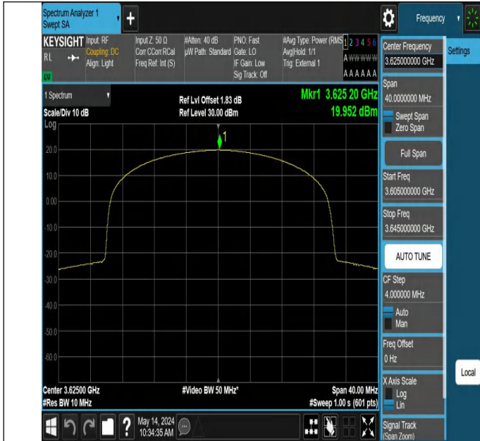
Band48-15MHz-64QAM-55990-38RB#37-PASS
