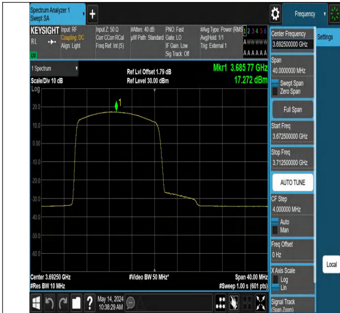
Band48-15MHz-256QAM-56665-1RB#0-PASS
