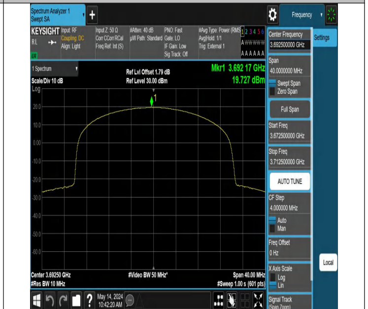
Band48-15MHz-QPSK-56665-38RB#0-PASS
