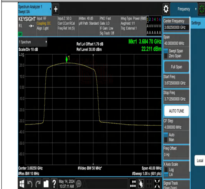
Band48-15MHz-QPSK-56665-1RB#0-PASS
