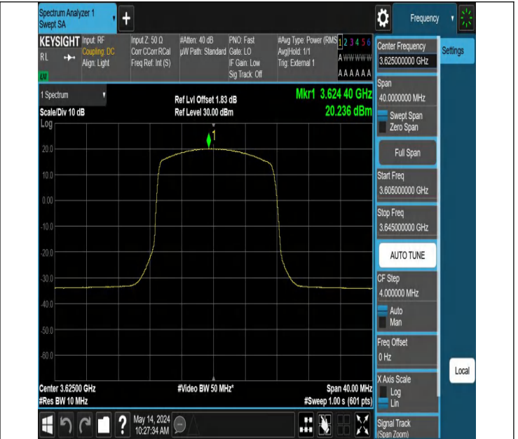
Band48-15MHz-64QAM-55990-1RB#38-PASS
