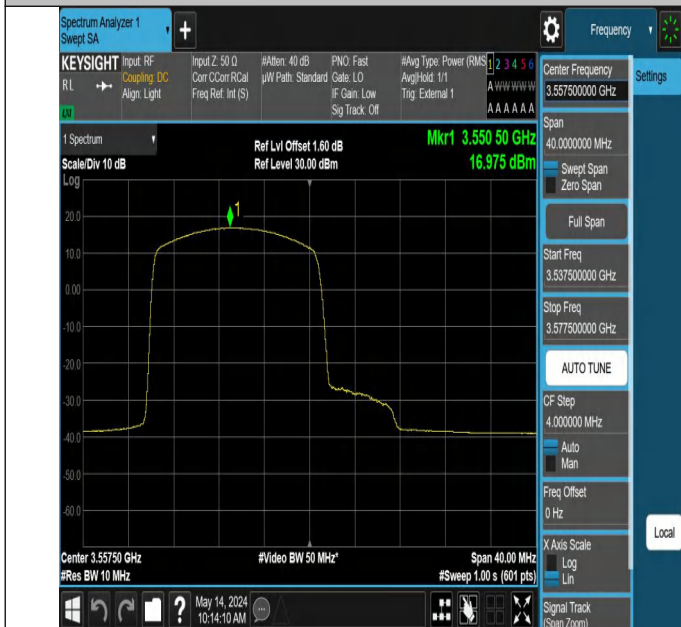
Band48-15MHz-256QAM-55315-1RB#0-PASS
