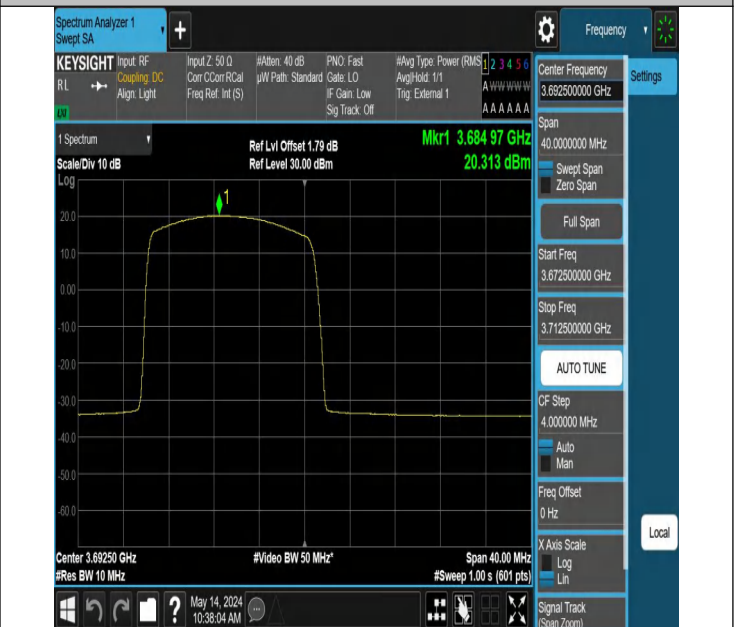
Band48-15MHz-64QAM-56665-1RB#0-PASS
