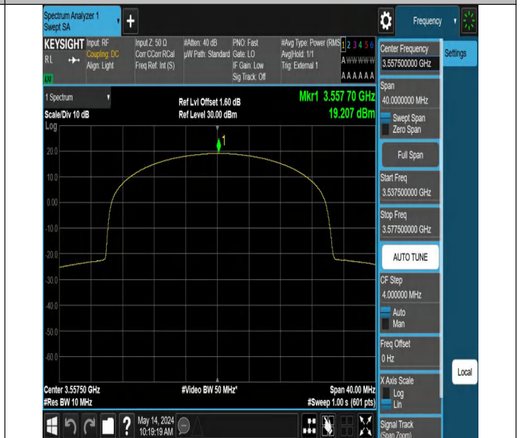
Band48-15MHz-256QAM-55315-38RB#0-PASS
