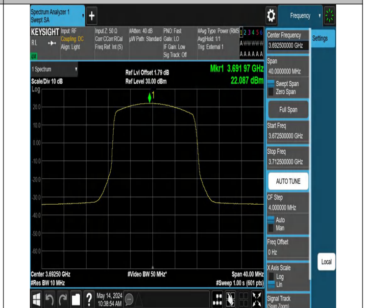
Band48-15MHz-QPSK-56665-1RB#38-PASS
