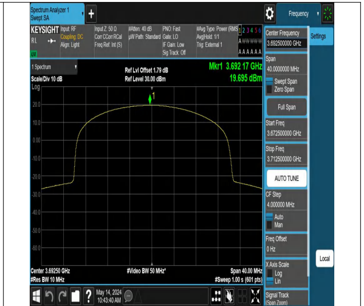
Band48-15MHz-256QAM-56665-38RB#0-PASS
