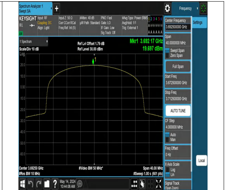
Band48-15MHz-QPSK-56665-38RB#18-PASS
