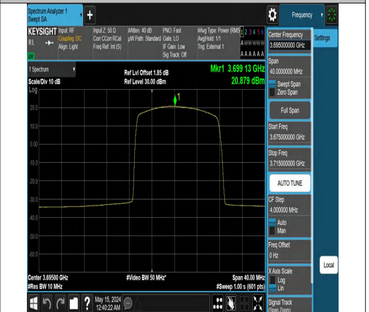
Band48-10MHz-16QAM-56690-1RB#49-PASS
