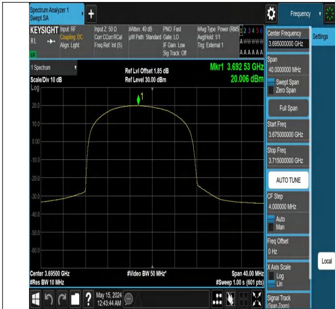
Band48-10MHz-16QAM-56690-25RB#12-PASS
