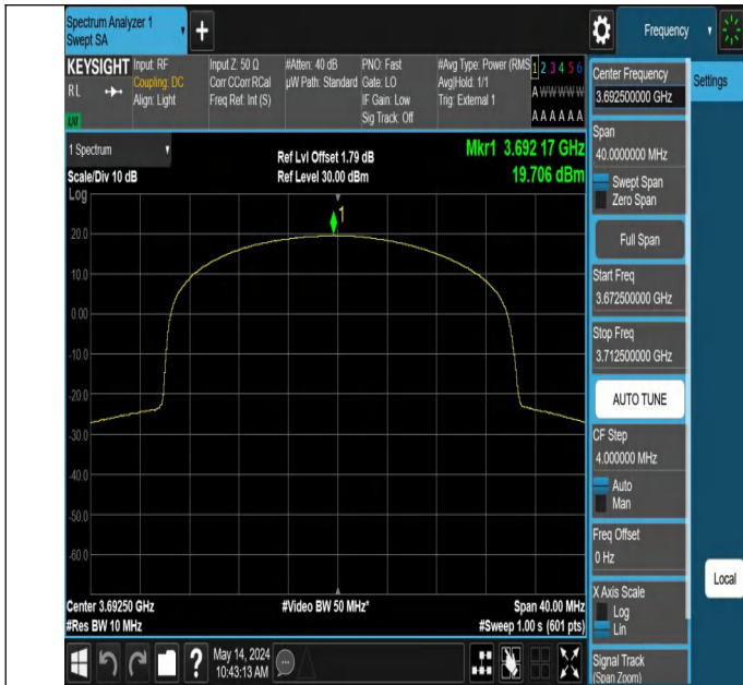
Band48-15MHz-64QAM-56665-38RB#0-PASS
