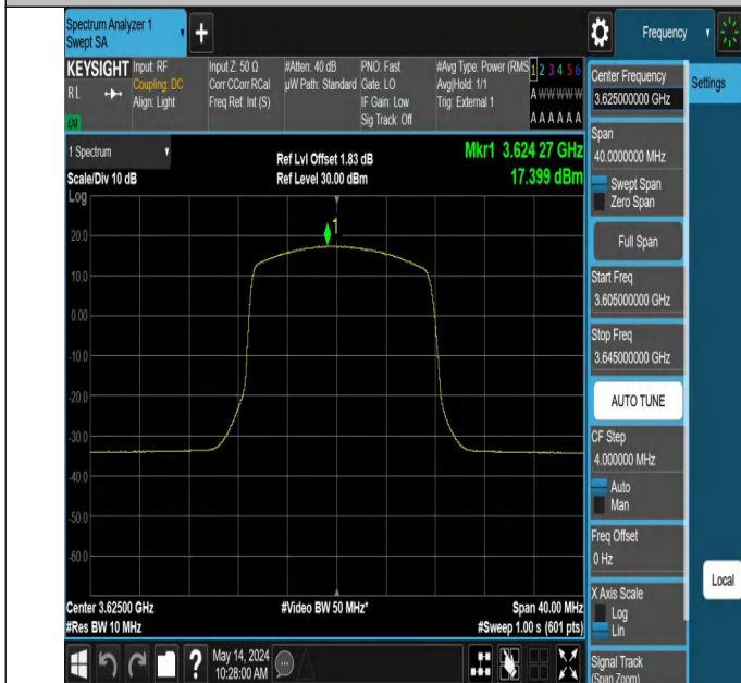
Band48-15MHz-256QAM-55990-1RB#38-PASS
