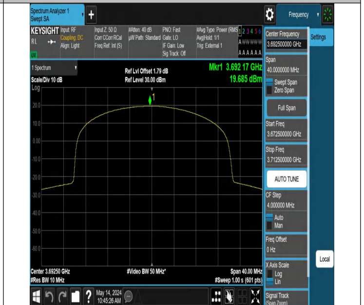
Band48-15MHz-256QAM-56665-38RB#18-PASS
