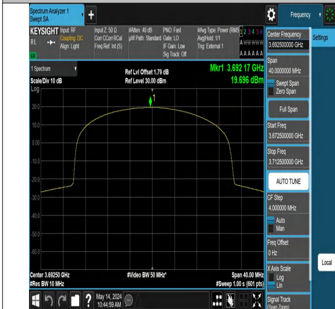
Band48-15MHz-64QAM-56665-38RB#18-PASS
