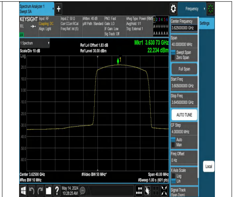
Band48-15MHz-QPSK-55990-1RB#74-PASS
