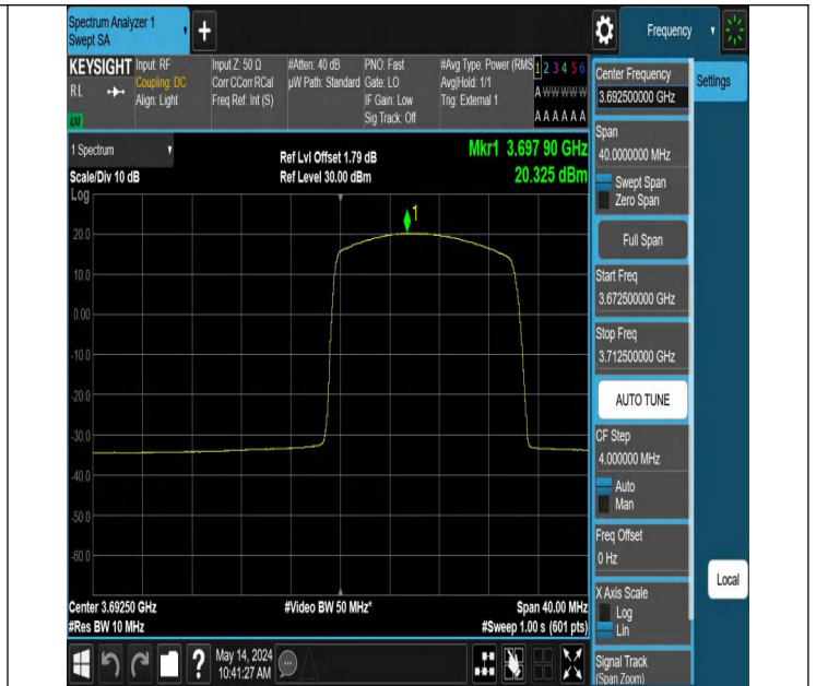
Band48-15MHz-64QAM-56665-1RB#74-PASS
