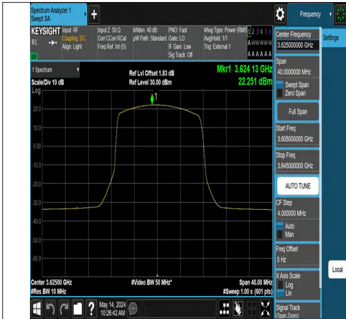
Band48-15MHz-QPSK-55990-1RB#38-PASS
