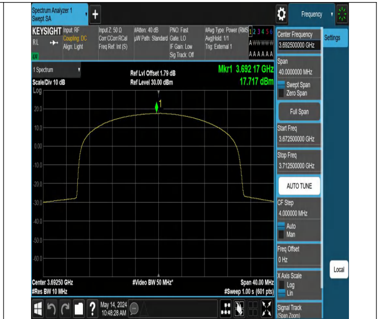
Band48-15MHz-64QAM-56665-75RB#0-PASS
