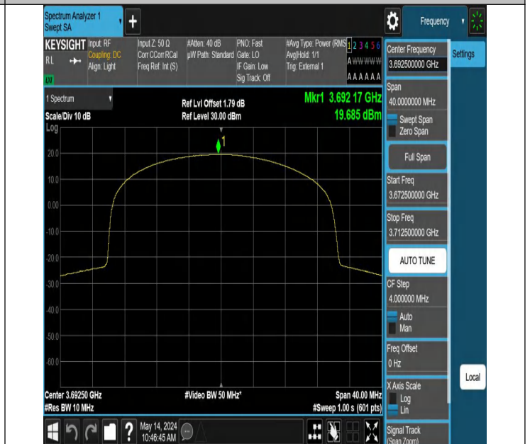
Band48-15MHz-64QAM-56665-38RB#37-PASS
