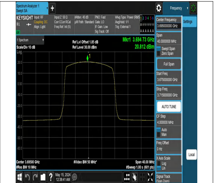
Band48-10MHz-16QAM-56690-1RB#24-PASS
