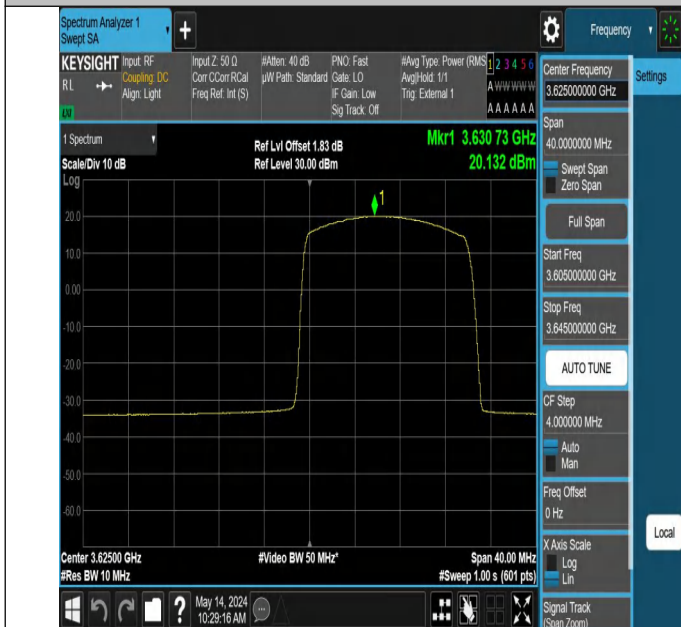
Band48-15MHz-64QAM-55990-1RB#74-PASS
