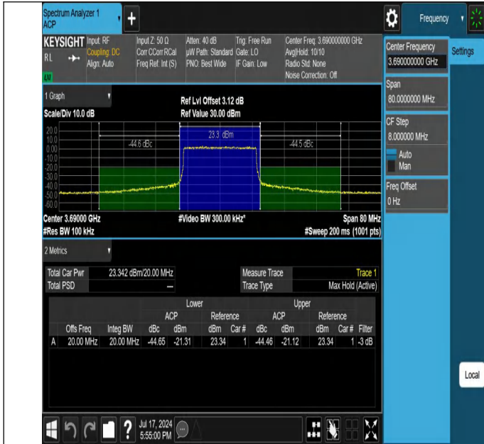
Band48-20MHz-QPSK-56640-100RB#0-PASS
