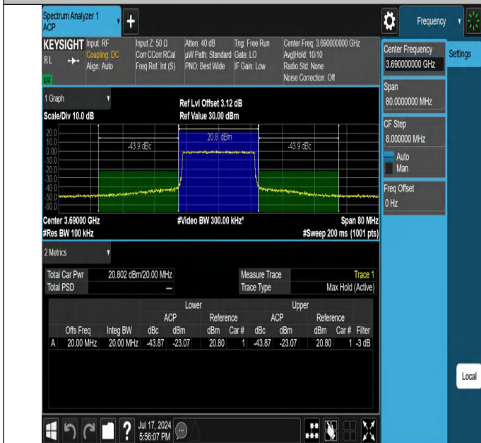
Band48-20MHz-64QAM-56640-100RB#0-PASS
