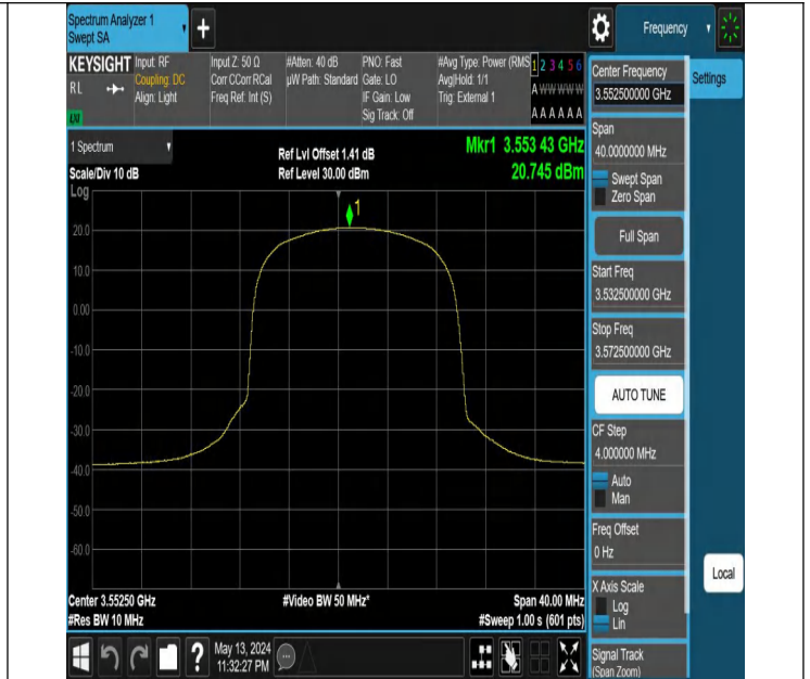
Band48-5MHz-QPSK-55265-12RB#13-PASS
