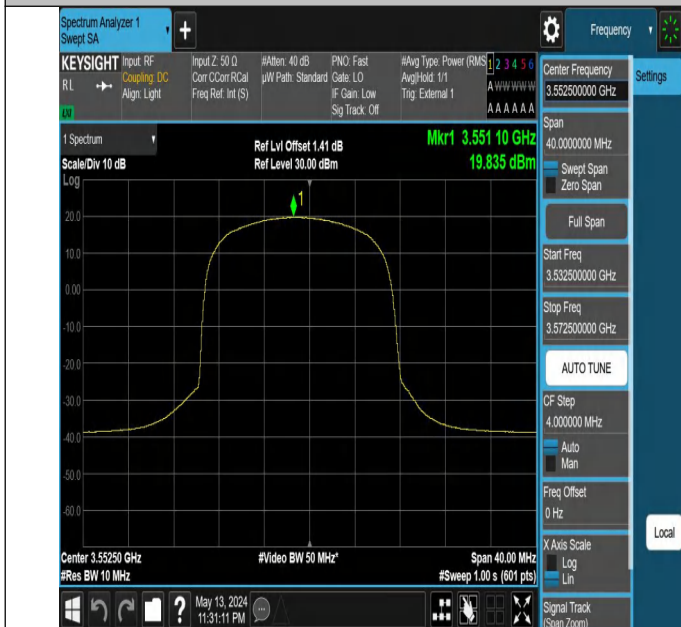
Band48-5MHz-16QAM-55265-12RB#6-PASS
