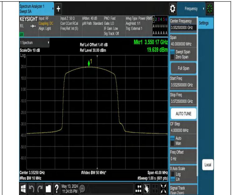
Band48-5MHz-64QAM-55265-1RB#0-PASS
