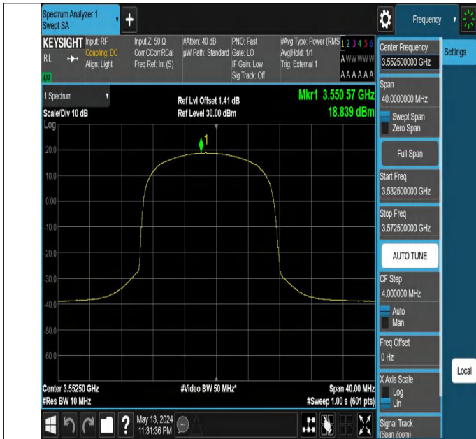
Band48-5MHz-64QAM-55265-12RB#6-PASS
