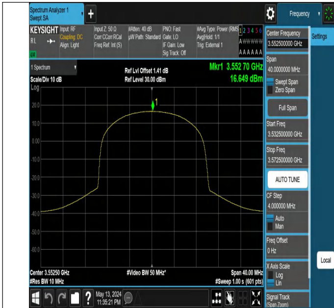
Band48-5MHz-256QAM-55265-25RB#0-PASS
