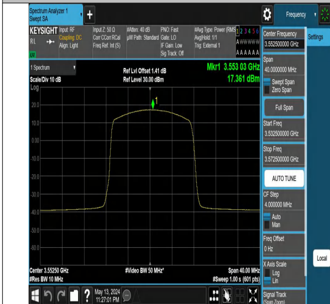
Band48-5MHz-256QAM-55265-1RB#12-PASS
