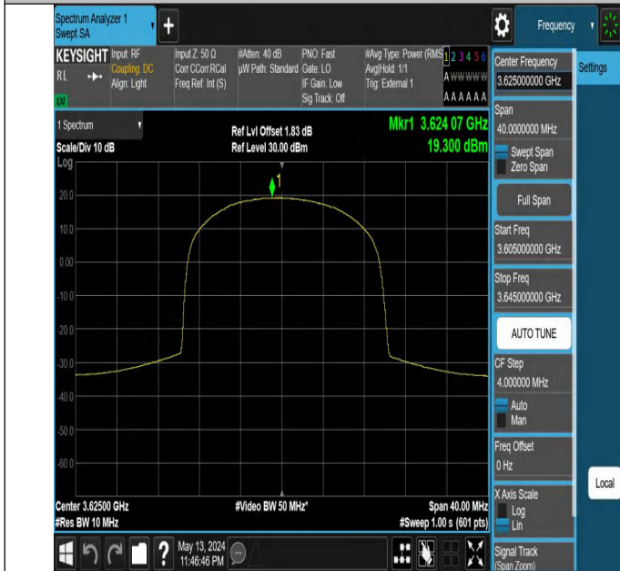
Band48-5MHz-64QAM-55990-25RB#0-PASS
