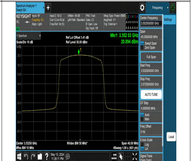
Band48-5MHz-16QAM-55265-1RB#12-PASS
