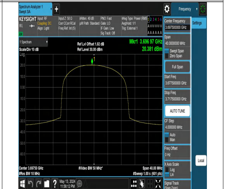
Band48-5MHz-16QAM-56715-25RB#0-PASS
