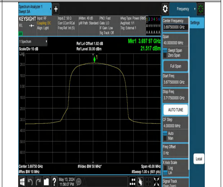
Band48-5MHz-QPSK-56715-12RB#13-PASS
