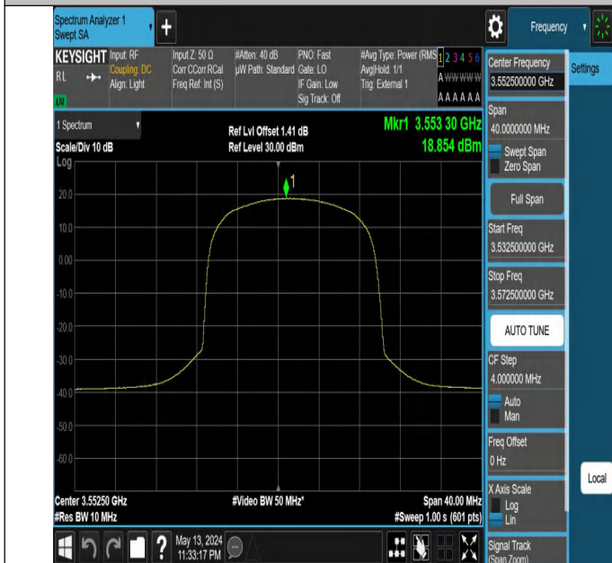
Band48-5MHz-64QAM-55265-12RB#13-PASS
