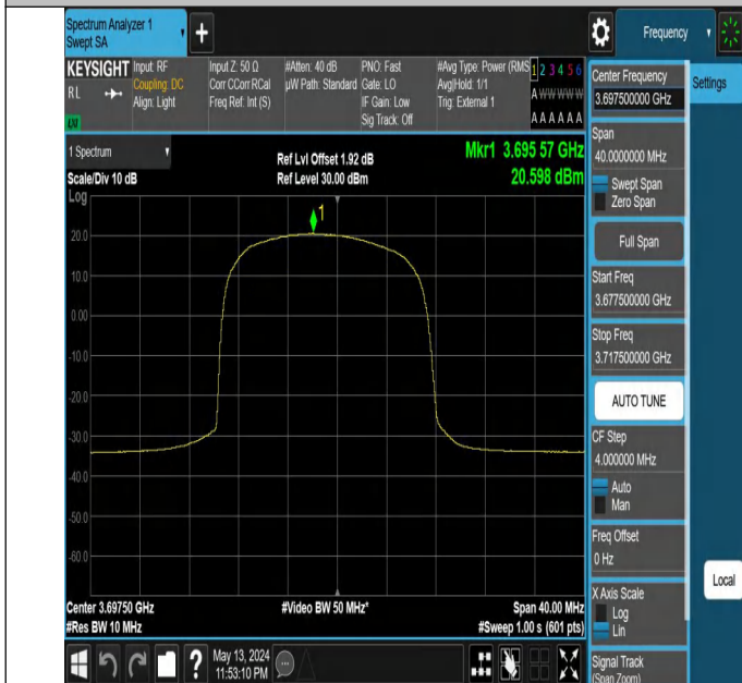
Band48-5MHz-16QAM-56715-12RB#0-PASS
