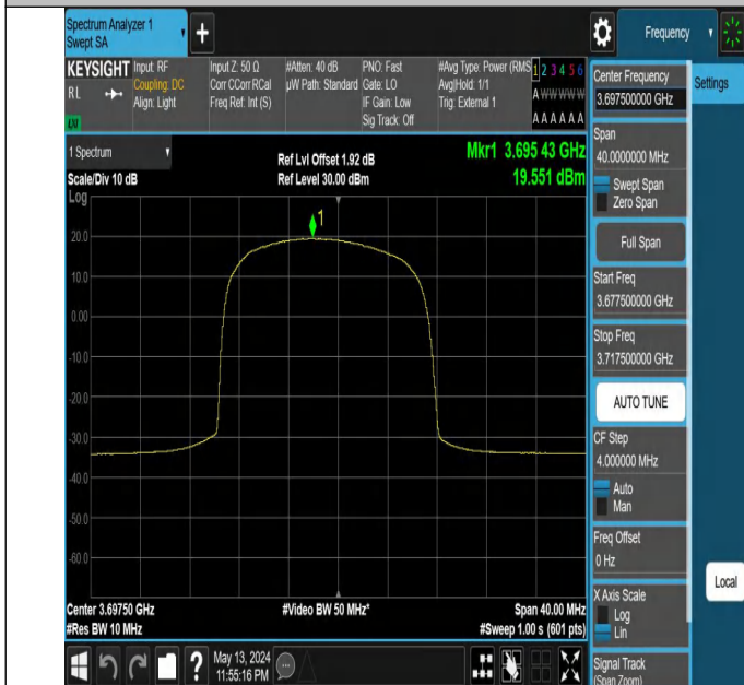
Band48-5MHz-64QAM-56715-12RB#6-PASS
