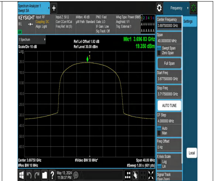
Band48-5MHz-64QAM-56715-25RB#0-PASS
