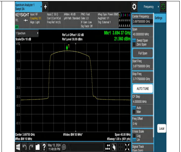
Band48-5MHz-16QAM-56715-1RB#0-PASS
