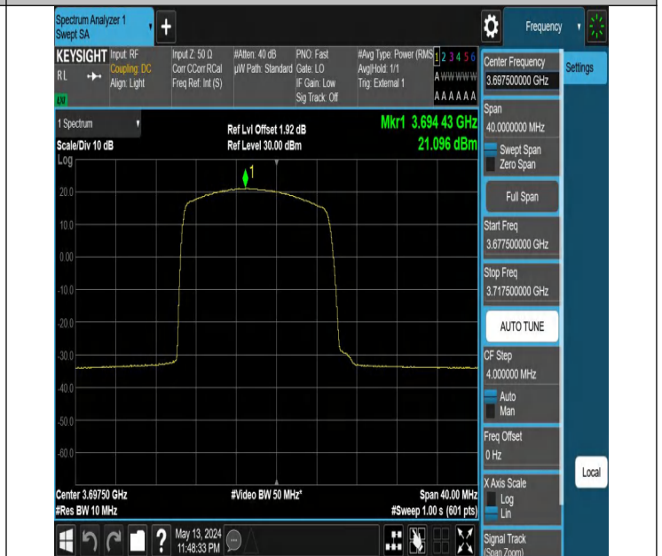
Band48-5MHz-64QAM-56715-1RB#0-PASS
