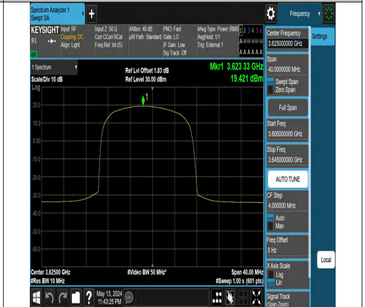
Band48-5MHz-64QAM-55990-12RB#6-PASS
