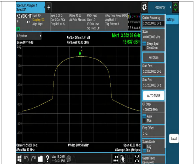
Band48-5MHz-16QAM-55265-25RB#0-PASS
