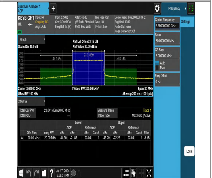
Band48-20MHz-256QAM-56640-100RB#0-PASS
