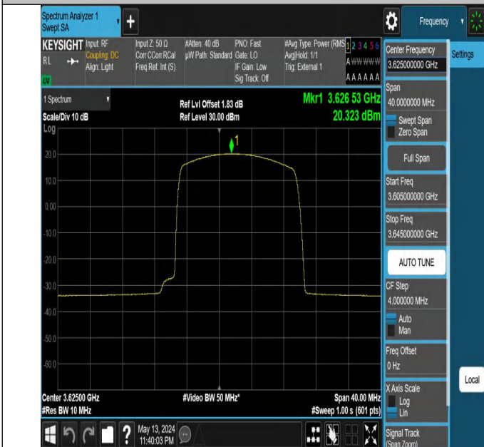
Band48-5MHz-64QAM-55990-1RB#24-PASS
