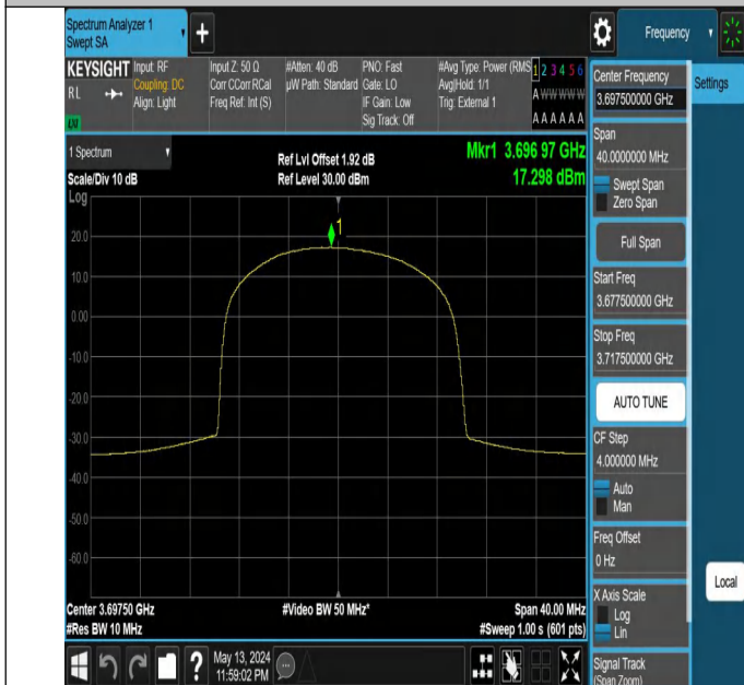
Band48-5MHz-256QAM-56715-25RB#0-PASS
