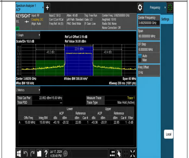
Band48-15MHz-256QAM-56665-1RB#0-PASS
