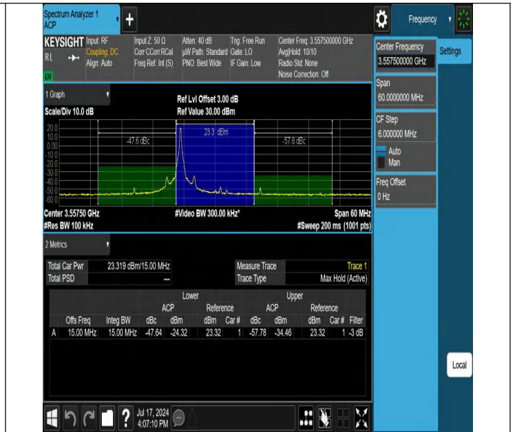
Band48-15MHz-16QAM-55315-1RB#0-PASS
