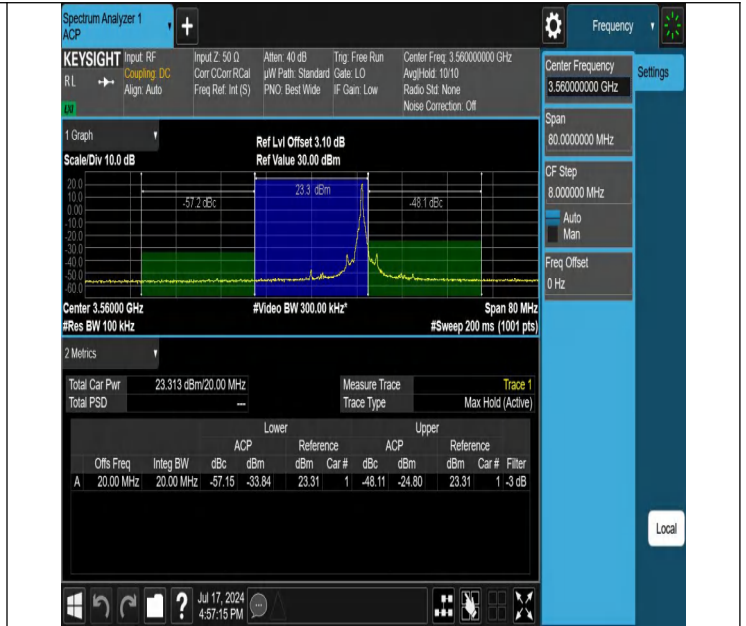
Band48-20MHz-16QAM-55340-1RB#99-PASS
