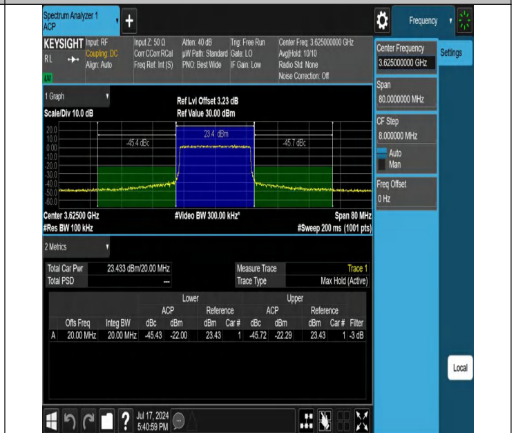
Band48-20MHz-256QAM-55990-1RB#99-PASS
