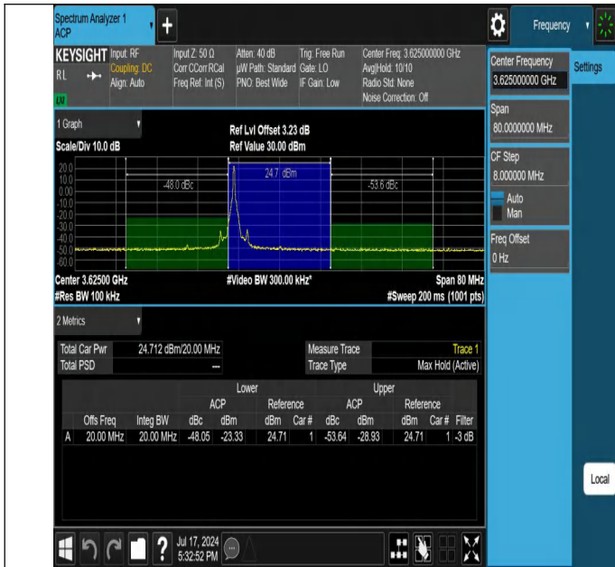
Band48-20MHz-QPSK-55990-1RB#0-PASS
