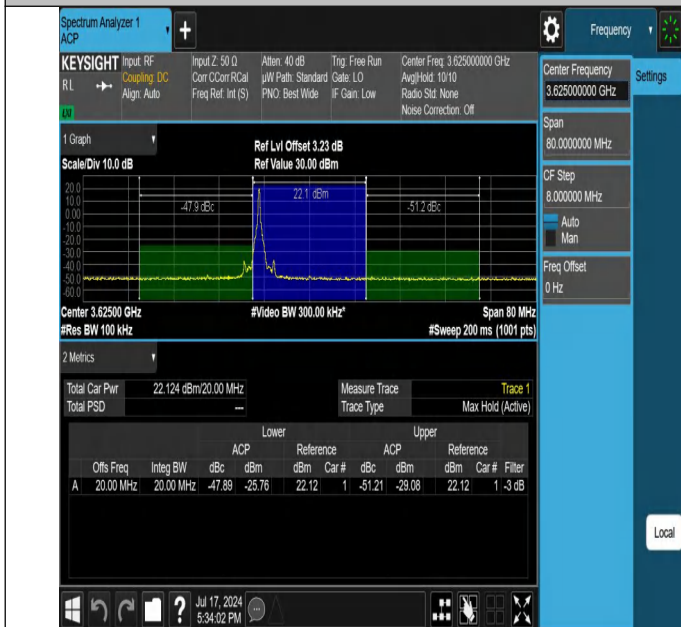
Band48-20MHz-64QAM-55990-1RB#0-PASS
