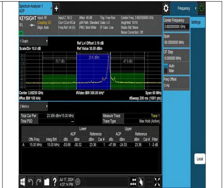
Band48-15MHz-16QAM-56665-1RB#74-PASS
