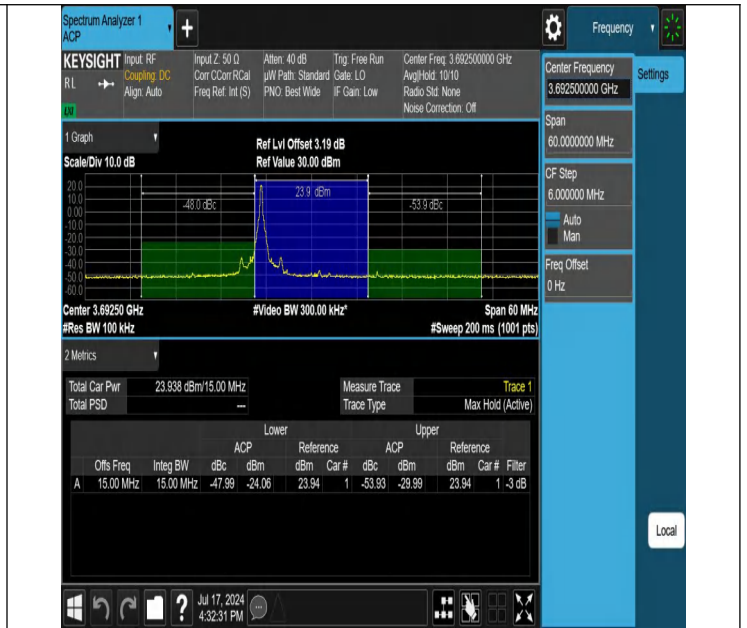
Band48-15MHz-16QAM-56665-1RB#0-PASS
