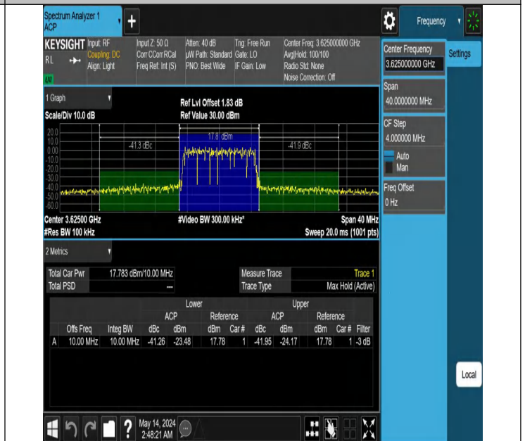
Band48-10MHz-256QAM-55990-50RB#0-PASS
