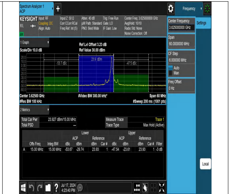
Band48-15MHz-16QAM-55990-1RB#74-PASS
