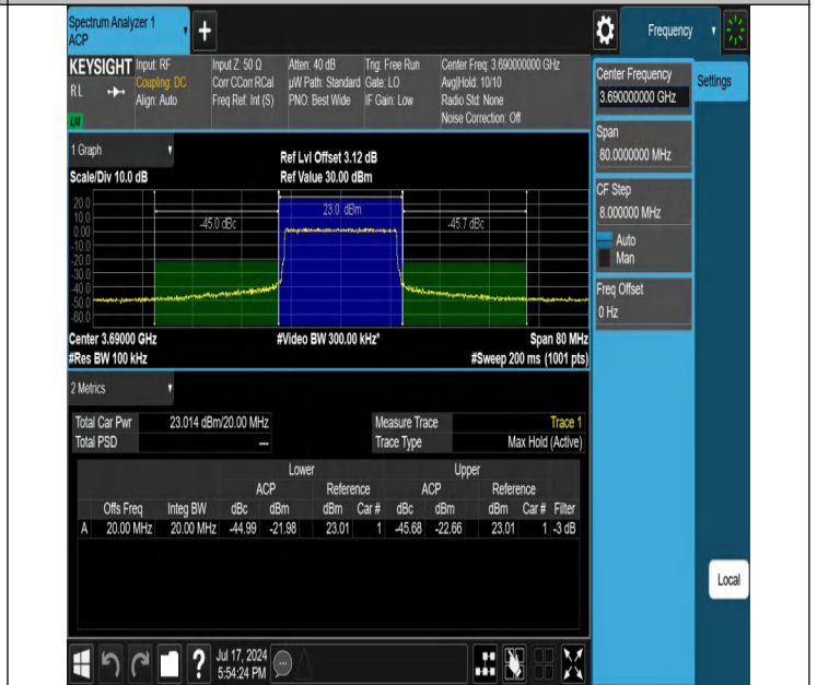
Band48-20MHz-256QAM-56640-1RB#99-PASS
