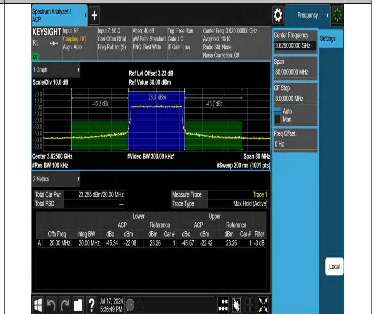
Band48-20MHz-256QAM-55990-1RB#0-PASS
