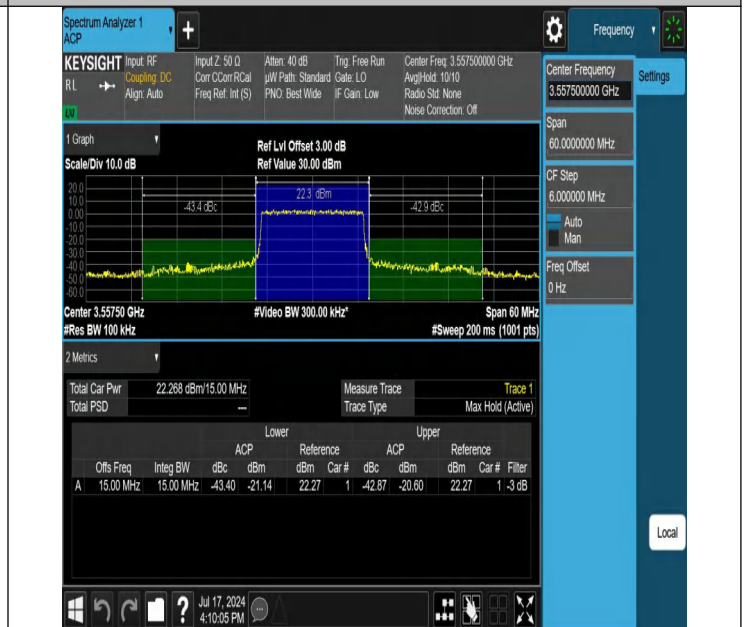
Band48-15MHz-256QAM-55315-1RB#0-PASS
