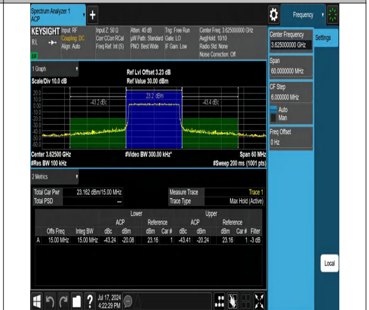
Band48-15MHz-256QAM-55990-1RB#0-PASS
