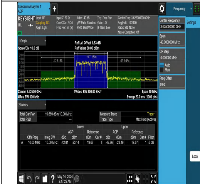
Band48-10MHz-64QAM-55990-50RB#0-PASS
