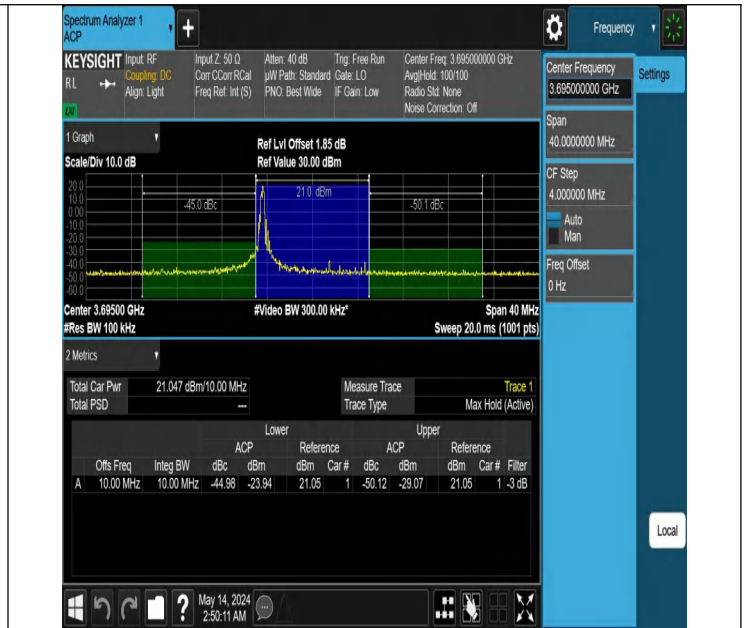
Band48-10MHz-16QAM-56690-1RB#0-PASS
