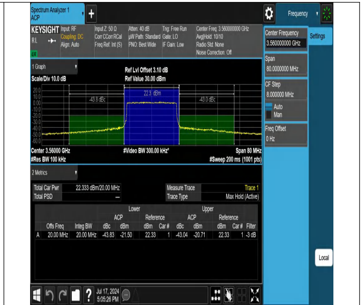
Band48-20MHz-16QAM-55340-100RB#0-PASS
