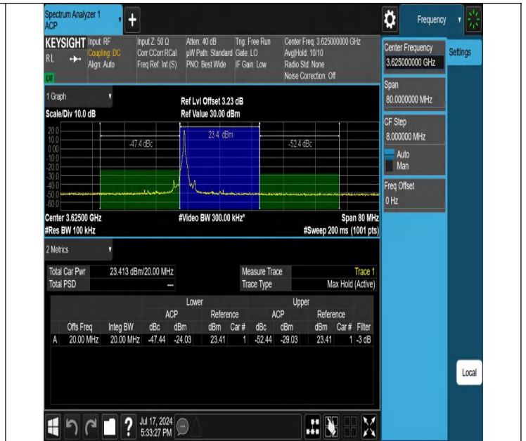
Band48-20MHz-16QAM-55990-1RB#0-PASS
