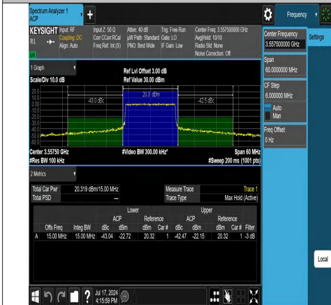
Band48-15MHz-64QAM-55315-75RB#0-PASS
