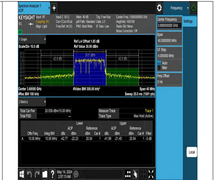
Band48-10MHz-16QAM-56690-50RB#0-PASS
