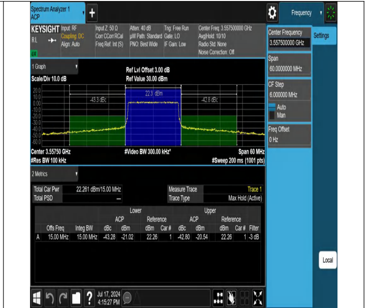
Band48-15MHz-16QAM-55315-75RB#0-PASS
