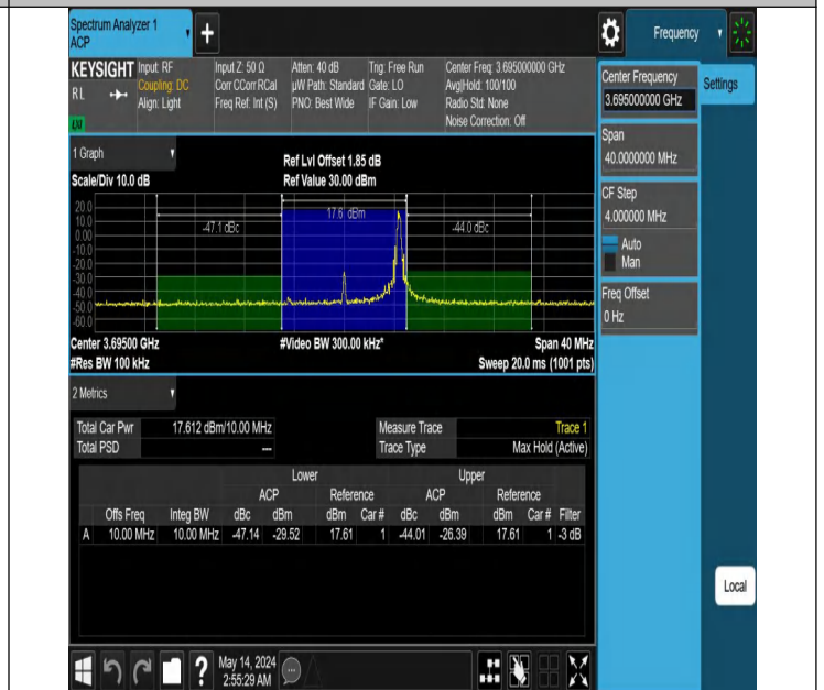
Band48-10MHz-256QAM-56690-1RB#49-PASS
