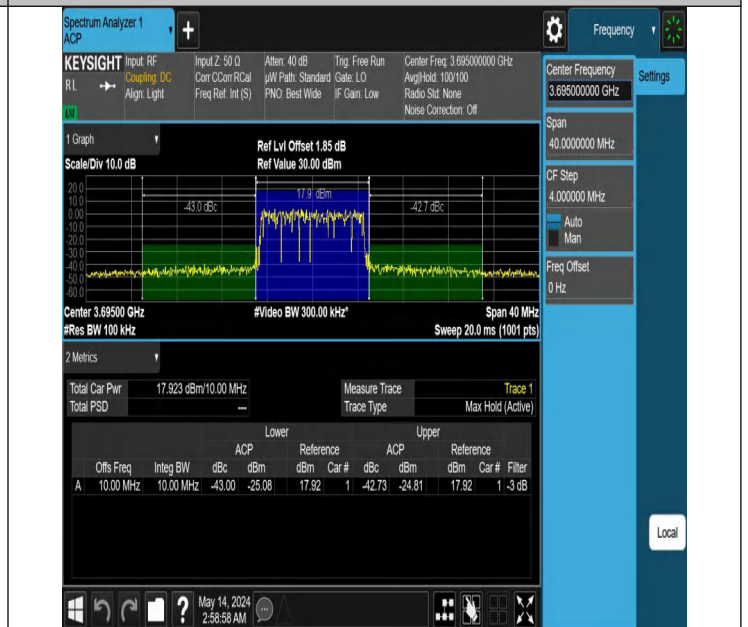
Band48-10MHz-256QAM-56690-50RB#0-PASS
