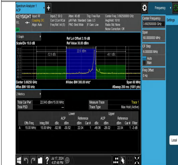
Band48-15MHz-64QAM-56665-1RB#74-PASS
