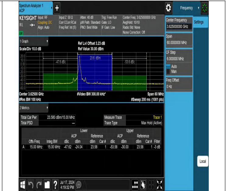
Band48-15MHz-16QAM-55990-1RB#0-PASS
