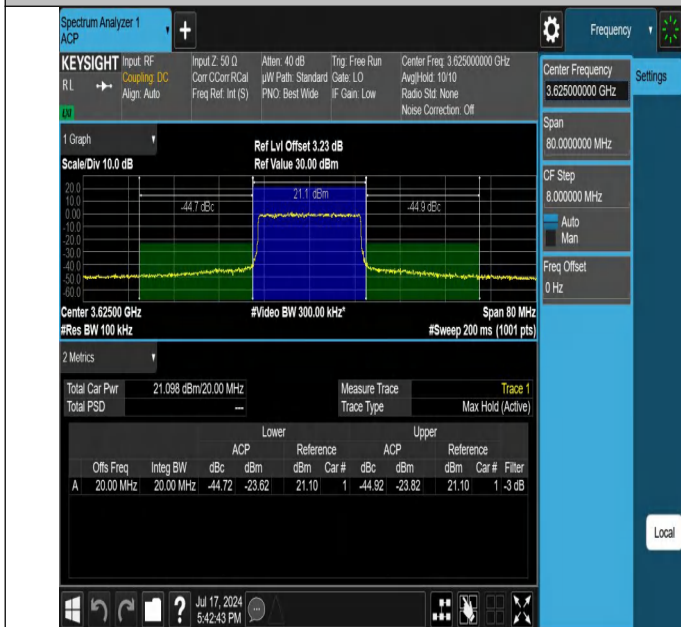
Band48-20MHz-64QAM-55990-100RB#0-PASS
