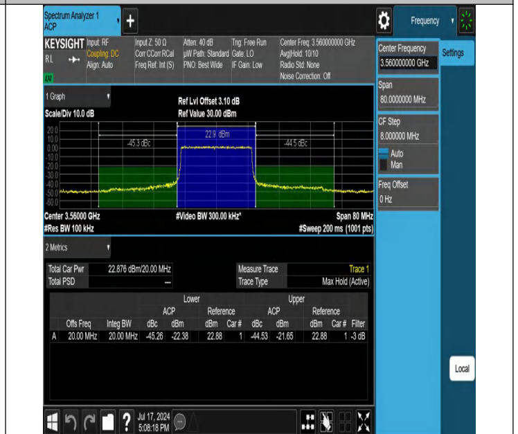
Band48-20MHz-256QAM-55340-100RB#0-PASS
