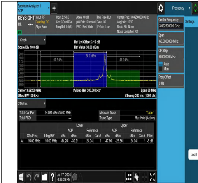
Band48-15MHz-QPSK-56665-1RB#74-PASS
