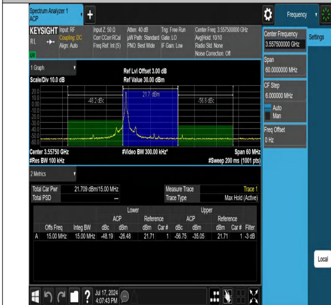
Band48-15MHz-64QAM-55315-1RB#0-PASS
