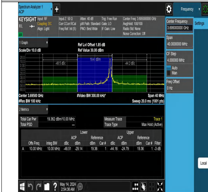
Band48-10MHz-64QAM-56690-1RB#49-PASS
