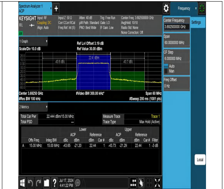
Band48-15MHz-16QAM-56665-75RB#0-PASS
