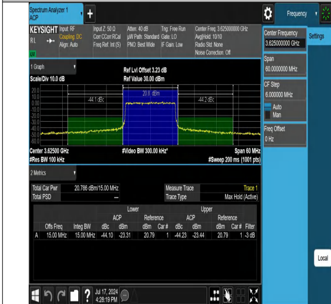
Band48-15MHz-64QAM-55990-75RB#0-PASS
