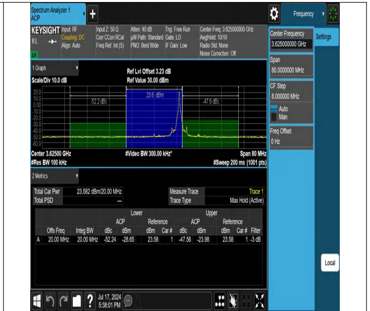
Band48-20MHz-16QAM-55990-1RB#99-PASS
