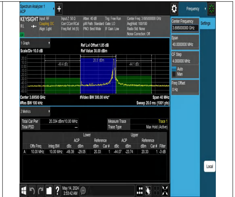
Band48-10MHz-16QAM-56690-1RB#49-PASS
