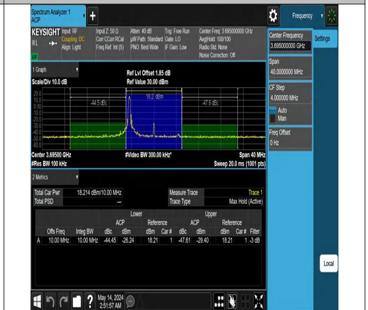
Band48-10MHz-256QAM-56690-1RB#0-PASS
