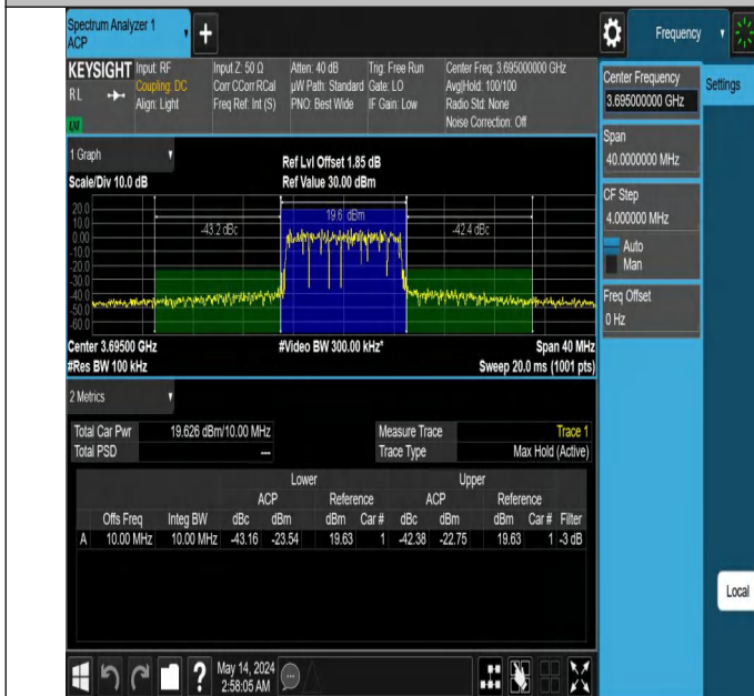
Band48-10MHz-64QAM-56690-50RB#0-PASS
