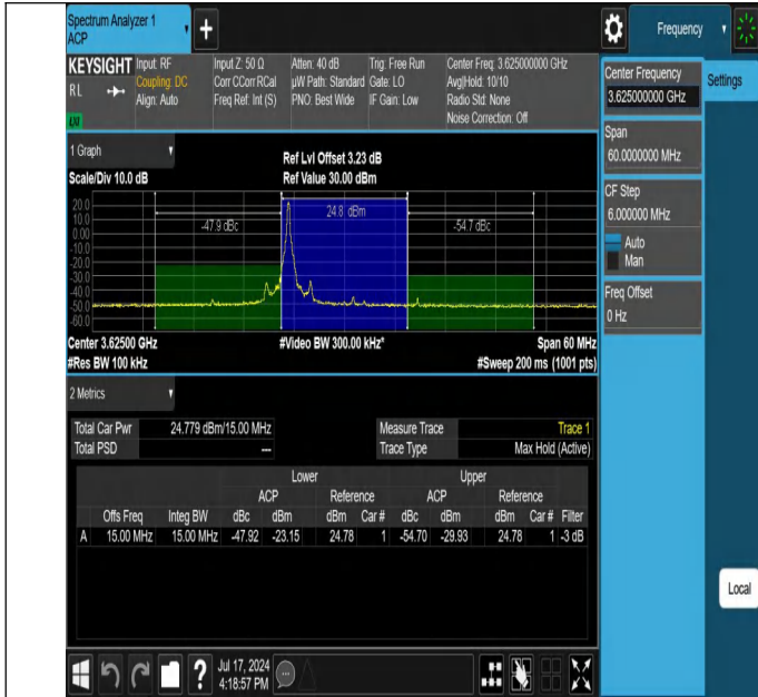
Band48-15MHz-QPSK-55990-1RB#0-PASS
