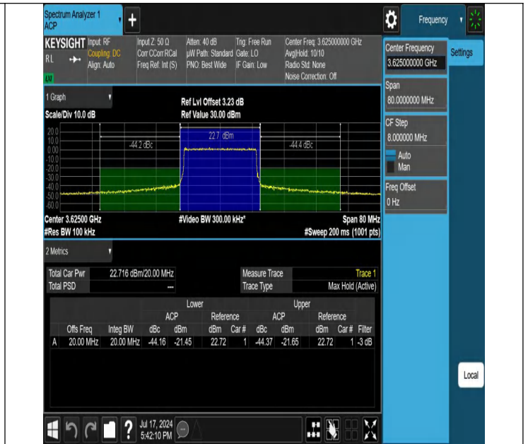
Band48-20MHz-16QAM-55990-100RB#0-PASS
