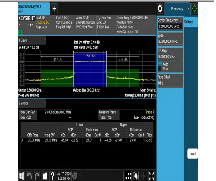
Band48-20MHz-256QAM-55340-1RB#0-PASS
