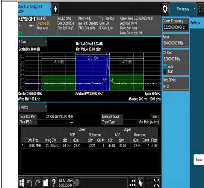
Band48-20MHz-64QAM-55990-1RB#99-PASS
