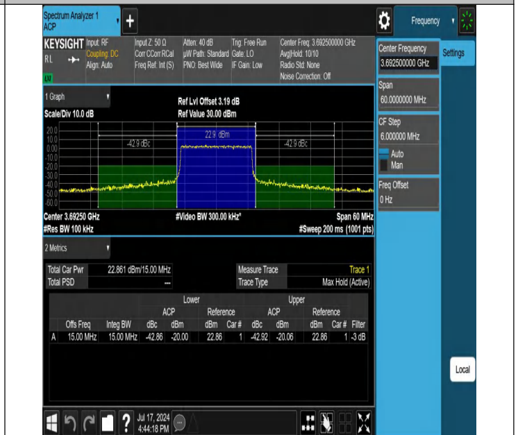
Band48-15MHz-256QAM-56665-75RB#0-PASS
