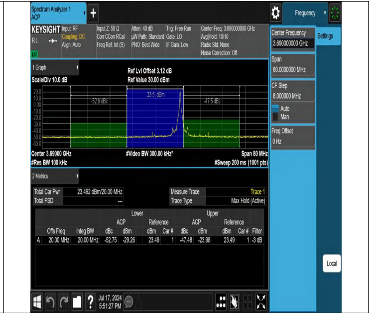
Band48-20MHz-16QAM-56640-1RB#99-PASS
