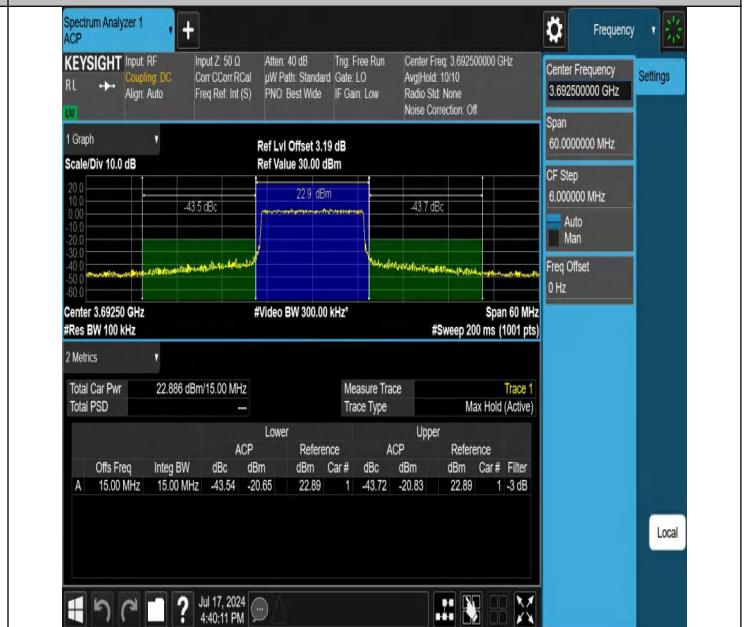
Band48-15MHz-256QAM-56665-1RB#74-PASS
