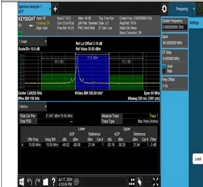
Band48-15MHz-64QAM-56665-1RB#0-PASS
