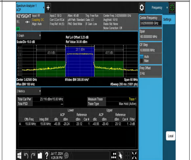
Band48-15MHz-256QAM-55990-1RB#74-PASS
