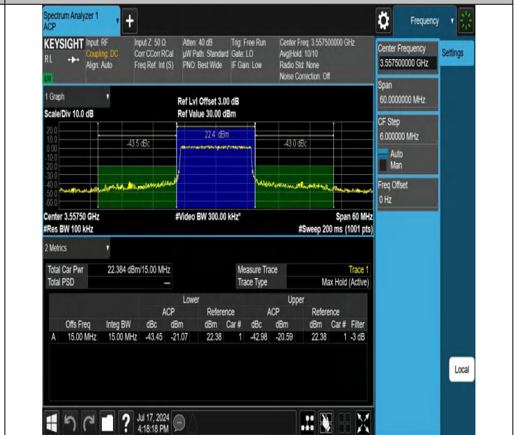
Band48-15MHz-256QAM-55315-75RB#0-PASS
