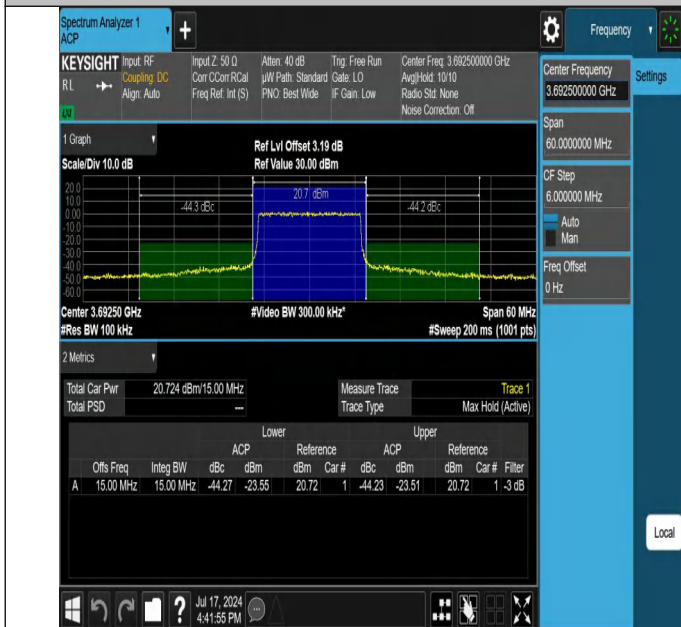
Band48-15MHz-64QAM-56665-75RB#0-PASS
