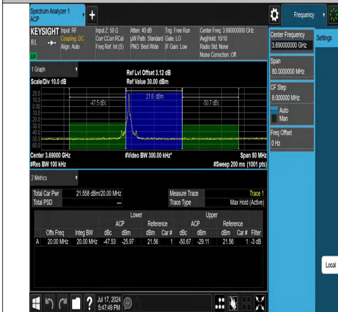
Band48-20MHz-64QAM-56640-1RB#0-PASS
