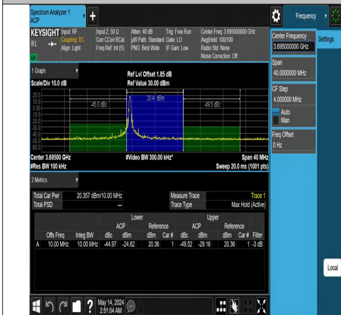
Band48-10MHz-64QAM-56690-1RB#0-PASS
