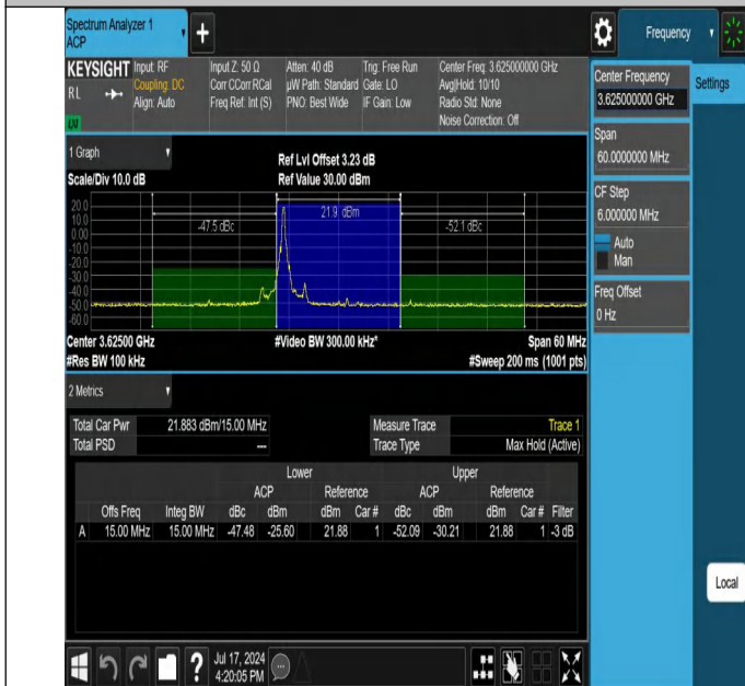
Band48-15MHz-64QAM-55990-1RB#0-PASS
