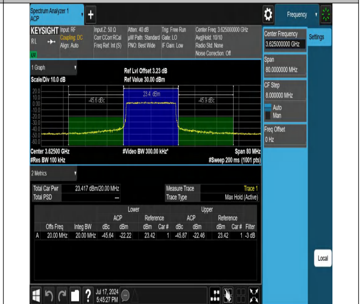
Band48-20MHz-256QAM-55990-100RB#0-PASS
