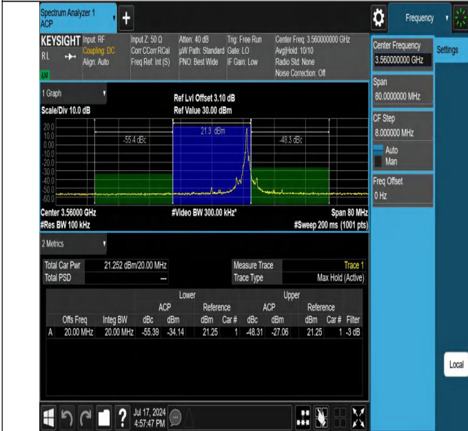
Band48-20MHz-64QAM-55340-1RB#99-PASS
