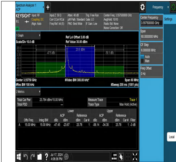
Band48-15MHz-QPSK-55315-1RB#0-PASS
