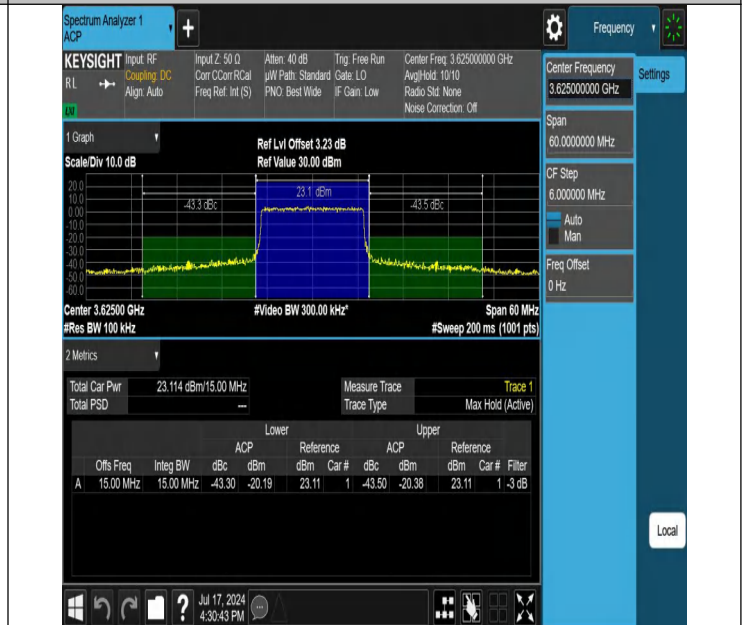
Band48-15MHz-256QAM-55990-75RB#0-PASS
