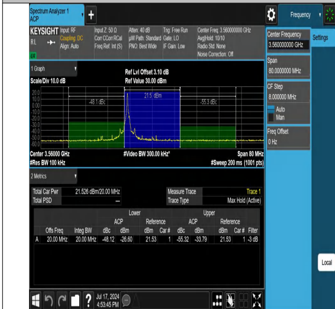
Band48-20MHz-64QAM-55340-1RB#0-PASS
