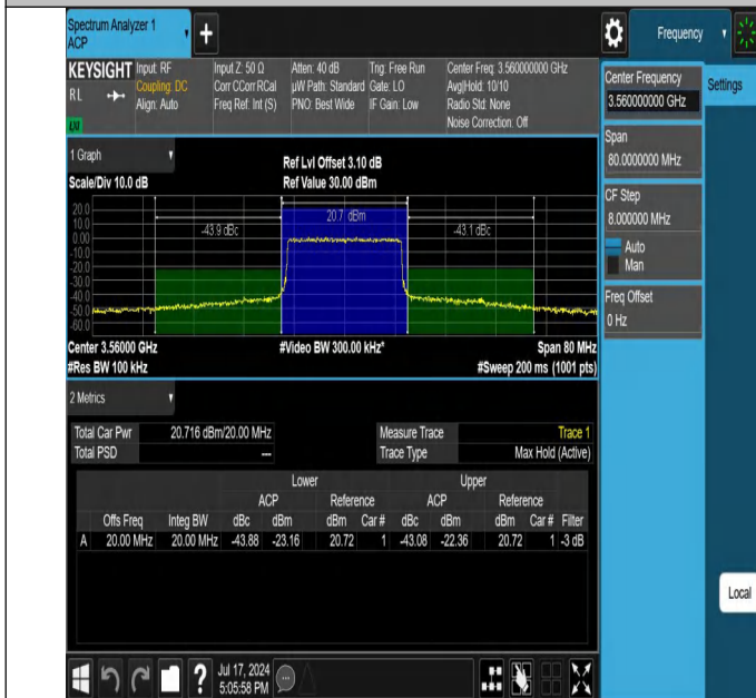
Band48-20MHz-64QAM-55340-100RB#0-PASS
