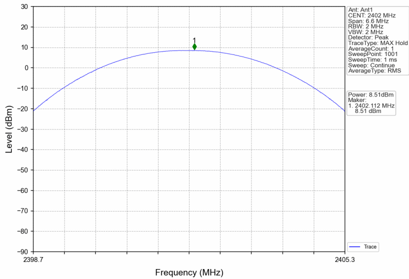
Pi/4QPSK_2DH5_LCH_2402MHz_Ant1_NTNV
