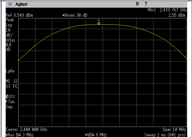
BLE_Mid Ch_2440MHz_2MBit_Output Power
