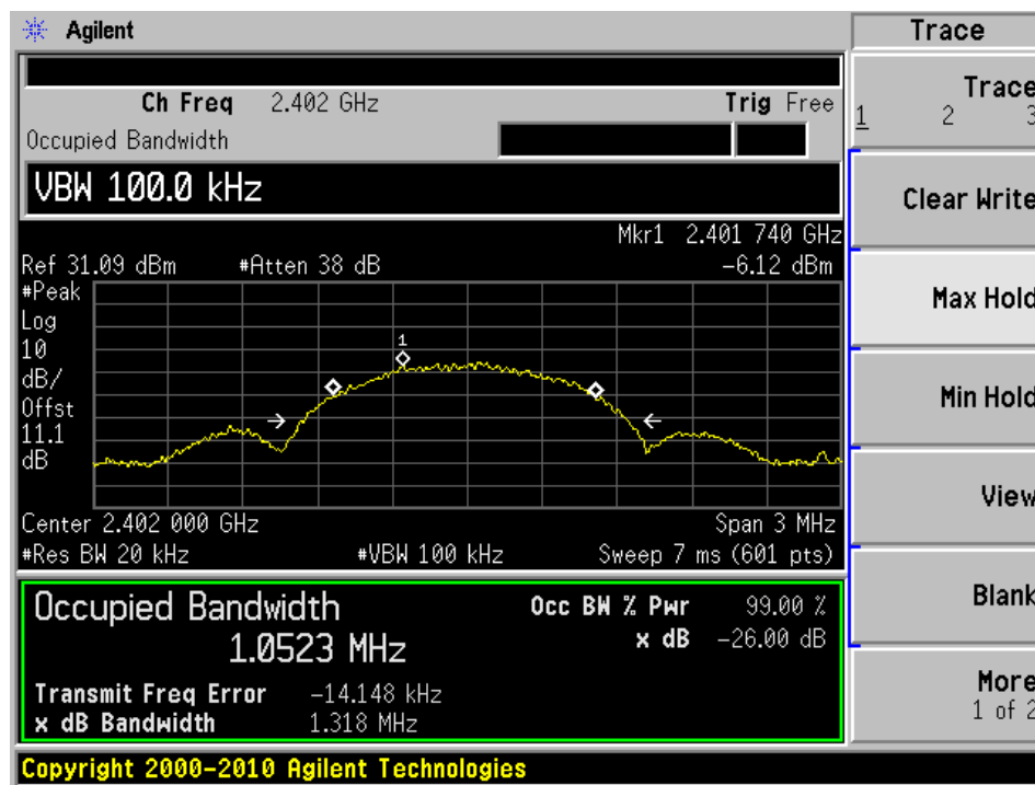
99% OBW, Low Channel: 2402 MHz
