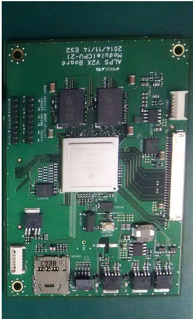
Outer Side
