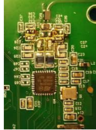
13.56 MHz Radio
