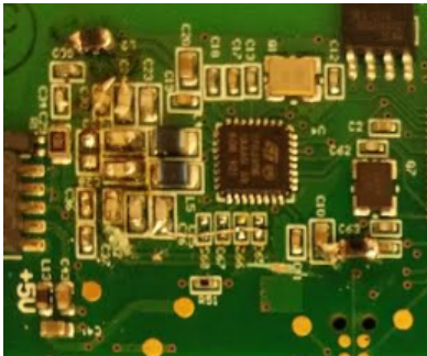
13.56 MHz Radio
