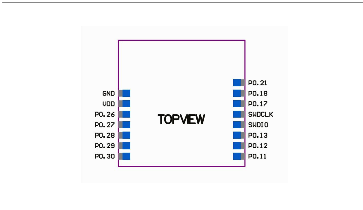
Figure 2: MESHTEK-H52E PINOUT
