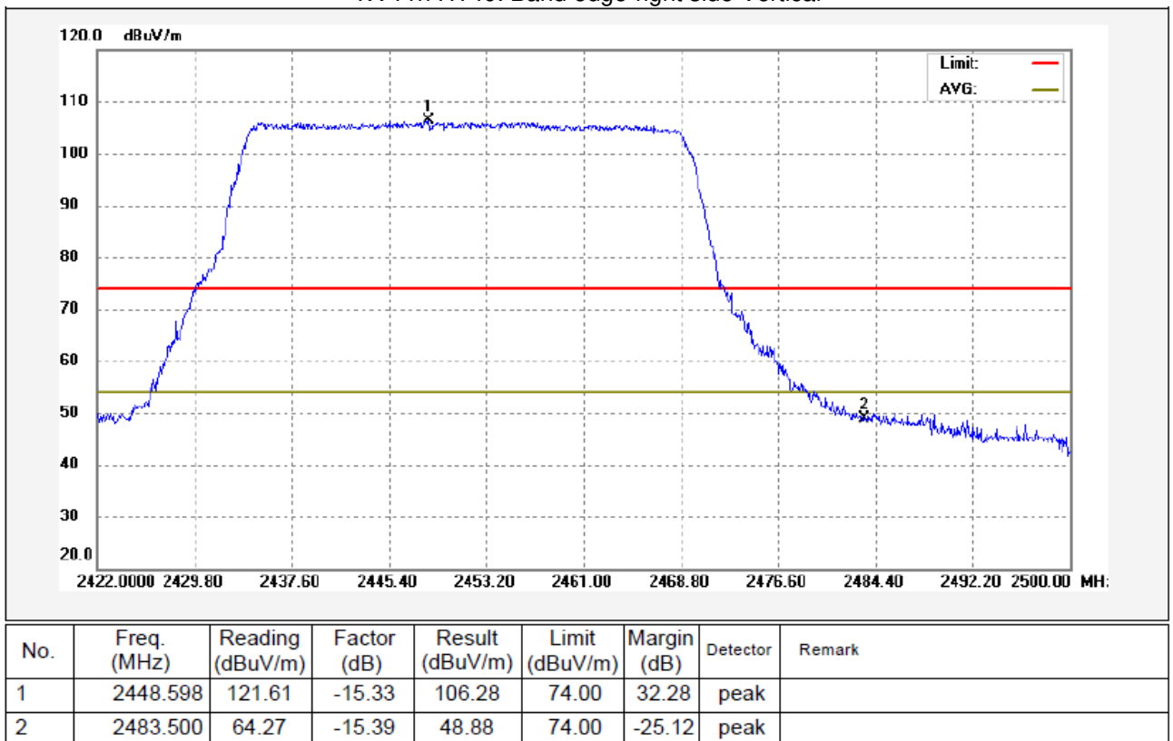
TX 11n HT40: Band edge-right side Vertical
