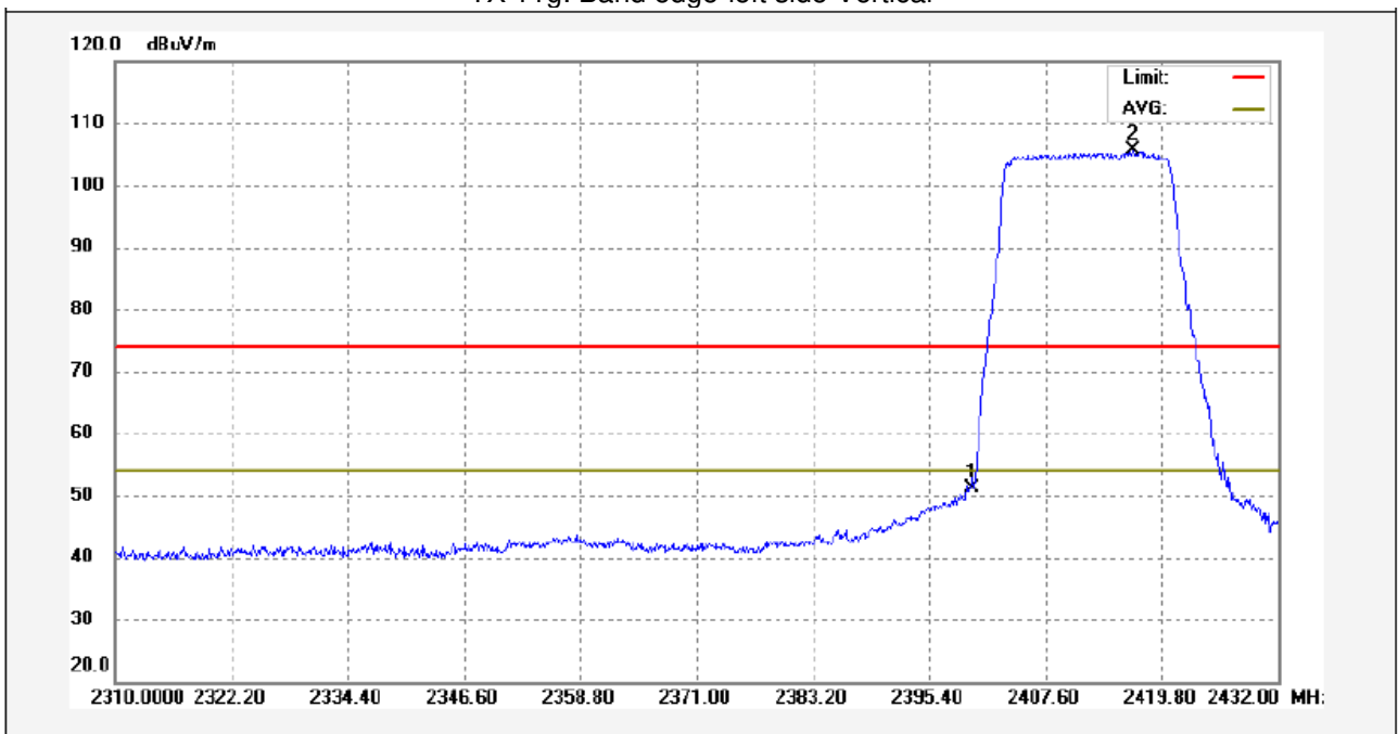
TX 11g: Band edge-left side Vertical
