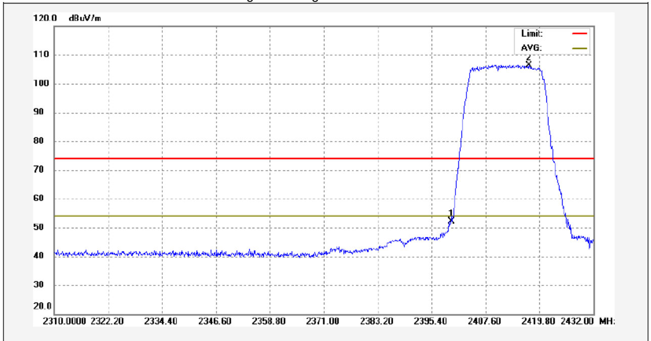
TX 11g: Band edge-left side Horizontal
