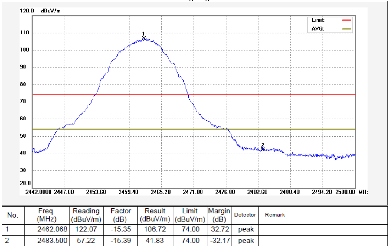
TX 11b: Band edge-right side Vertical
