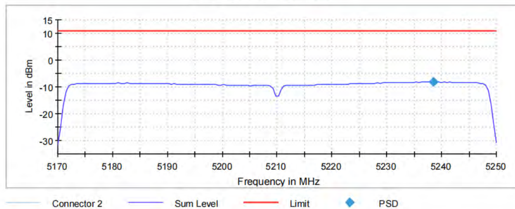
Power Spectral Density (SA-1)(2)
