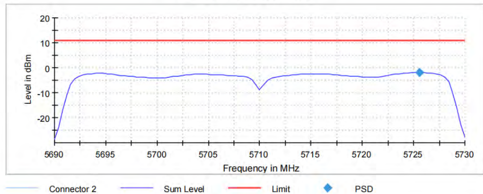
Power Spectral Density (SA-1)(2)
