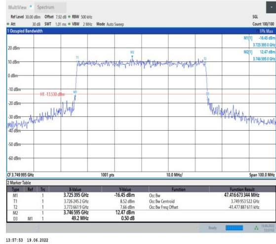
1-N78-3700-3800-PC2-30-50-M-8-CP-64QAM-Outer_Full-133@0-Ant1-47.417-49.200-≤50-PASS
