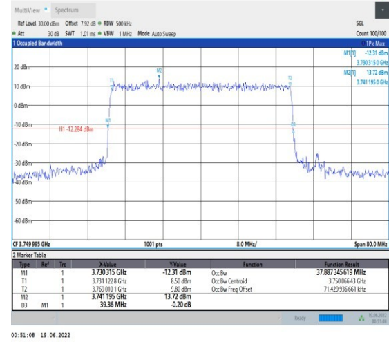
1-N78-3700-3800-PC2-30-40-M-7-CP-16QAM-Out_ Full-106@0-Ant1-37.887-39.360-≤40-PASS
