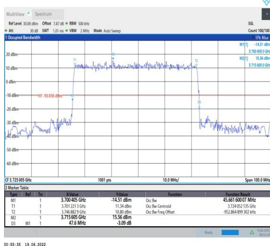
1-N78-3700-3800-PC2-30-50-L-2-DFT-PI2BPSK-Out er Full-128@0-Ant1-45.662-47.600-≤50-PASS
