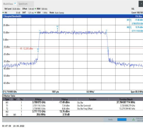
1-N78-3700-3800-PC2-30-40-L-7-CP-16QAM-Outer_Full-106@0-Ant1-37.784-39.600-≤40-PASS
