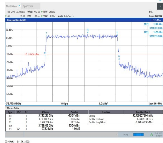
1-N78-3700-3800-PC2-30-40-M-1-DFT-QPSK-Outer_Full-100@0-Ant1-35.729-37.520-≤40-PASS
