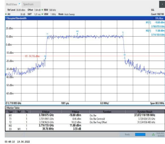
1-N78-3700-3800-PC2-30-40-L-8-CP-64QAM-Outer_Full-106@0-Ant1-37.872-39.760-≤40-PASS
