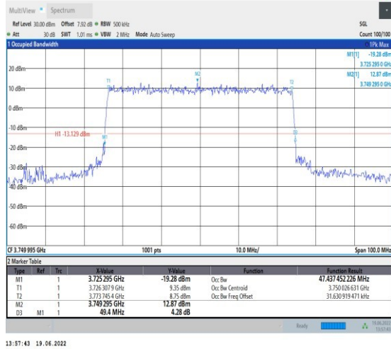
1-N78-3700-3800-PC2-30-50-M-7-CP-16QAM-Outer_Full-133@0-Ant1-47.437-49.400-≤50-PASS
