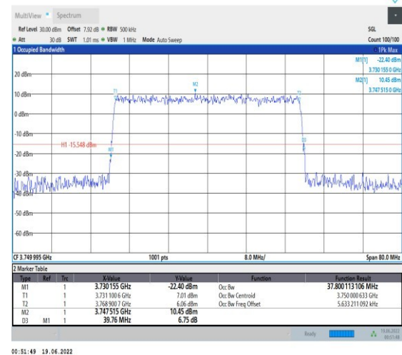
1-N78-3700-3800-PC2-30-40-M-9-CP-256QAM-Out_ Full-106@0-Ant1-37.8-39.760-≤40-PASS
