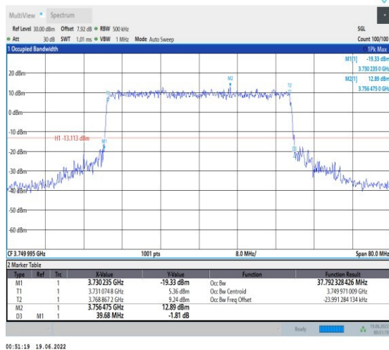
1-N78-3700-3800-PC2-30-40-M-8-CP-64QAM-Out_ Full-106@0-Ant1-37.792-39.680-≤40-PASS
