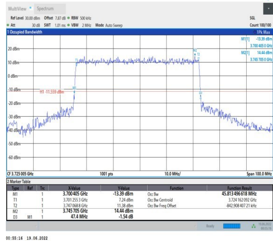
1-N78-3700-3800-PC2-30-50-L-1-DFT-QPSK-Outet_ Full-128@0-Ant1-45.813-47.400-≤50-PASS
