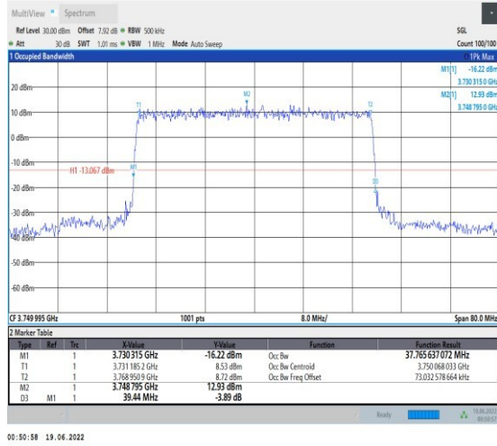
1-N78-3700-3800-PC2-30-40-M-6-CP-QPSK-Out_ Full-106@0-Ant1-37.766-39.440-≤40-PASS
