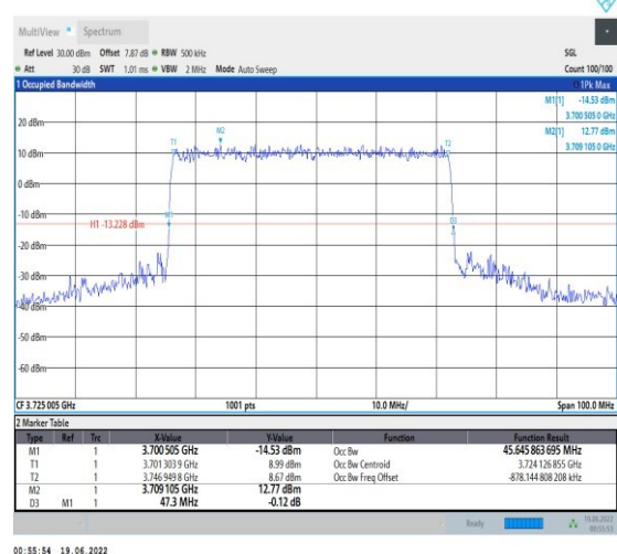
1-N78-3700-3800-PC2-30-50-L-3-DFT-16QAM-Outer Full-128@0-Ant1-45.646-47.300-≤50-PASS
