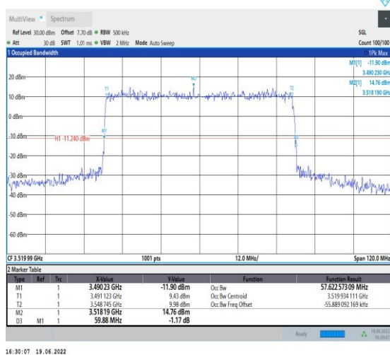
1-N78-3450-3550-PC2-30-60-H-1-DFT-QPSK-Outer_Full-162@0-Ant1-57.623-59.880-≤60-PASS
