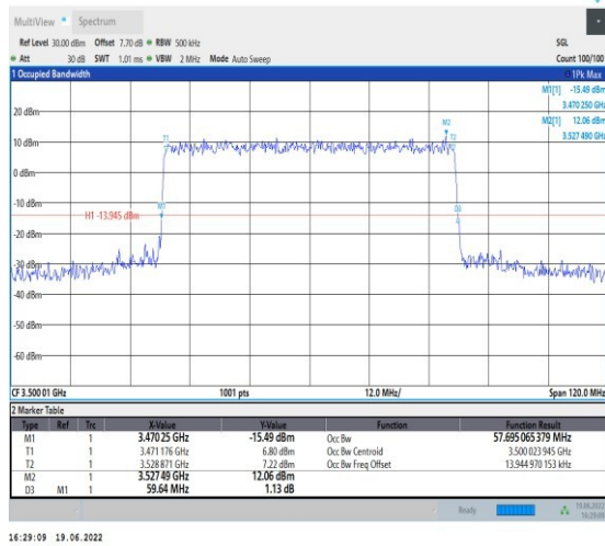
1-N78-3450-3550-PC2-30-60-M-8-CP-64QAM-Outer_Full-162@0-Ant1-57.695-59.640-≤60-PASS
