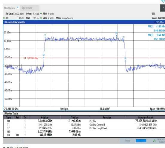
1-N78-3450-3550-PC2-30-80-L-3-DFT-16QAM-Outer_Full-216@0-Ant1-77.176-80.160-≤80-PASS
