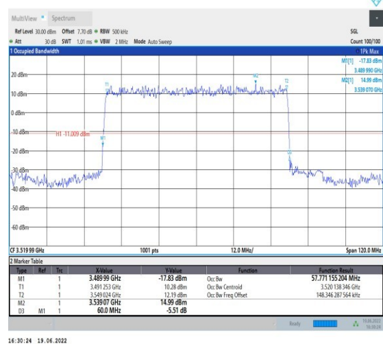
1-N78-3450-3550-PC2-30-60-H-2-DFT-PI2BPSK-Outer_Full-162@0-Ant1-57.771-60.000-≤60-PASS
