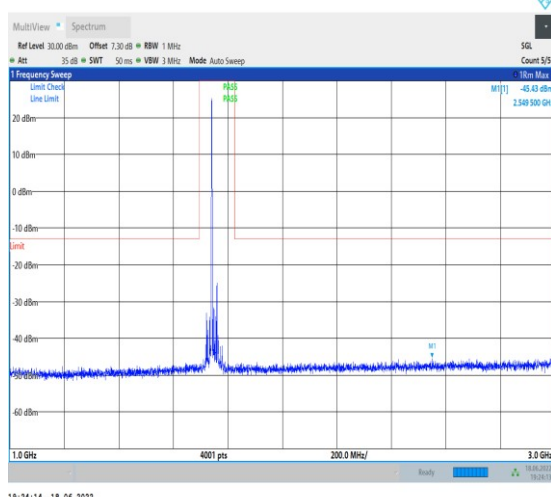
1-N66--15-40-H-1-DFT-PI2BPSK-Inner_1RB_Left-1 @1-1000-3000-Ant1--45.43--13-PASS
