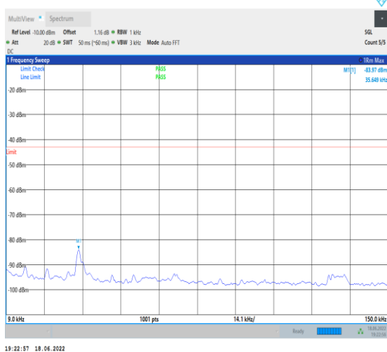
1-N66--15-40-M-1-DFT-PI2BPSK-Inner_1RB_Left-1 @1-0.009-0.15-Ant1--83.97--43-PASS
