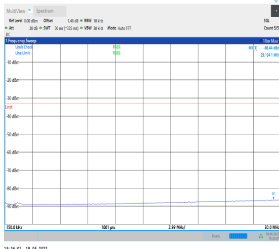
1-N66--15-40-H-1-DFT-PI2BPSK-Inner_1RB_Left-1 @1-0.15-30-Ant1--86.44--33-PASS
