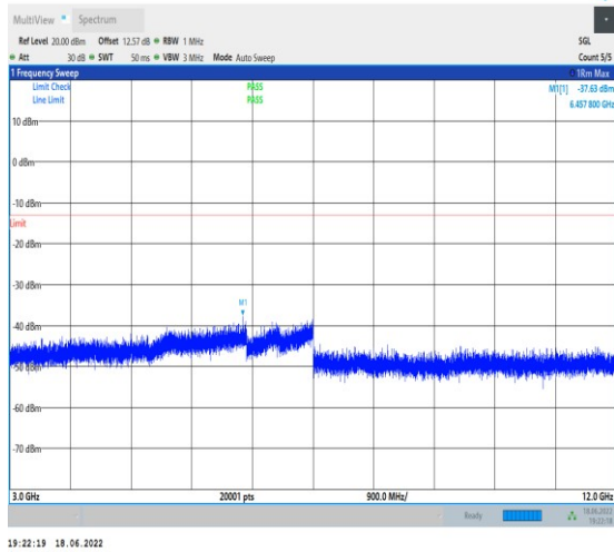
1-N66--15-40-L-1-DFT-PI2BPSK-Inner_1RB_Left-1 @1-3000-12000-Ant1--37.63--13-PASS
