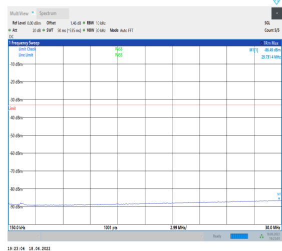
1-N66--15-40-M-1-DFT-PI2BPSK-Inner_1RB_Left-1 @1-0.15-30-Ant1--86.49--33-PASS
