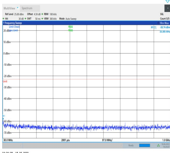
1-N66--15-40-H-1-DFT-PI2BPSK-Inner_1RB_Left-1 @1-30-1000-Ant1--58.74--23-PASS
