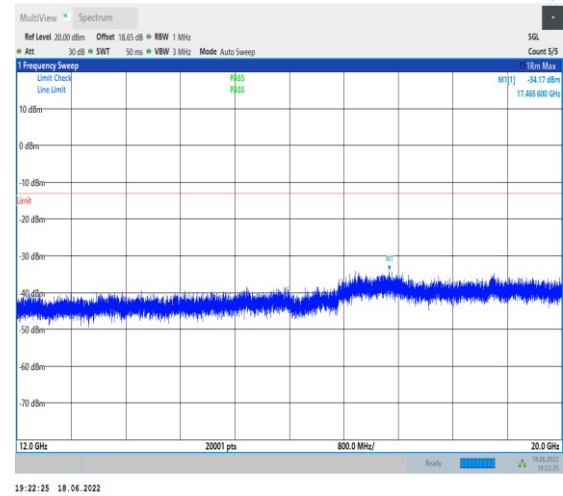
1-N66--15-40-L-1-DFT-PI2BPSK-Inner_1RB_Left-1@ 1-12000-20000-Ant1--34.17--13-PASS
