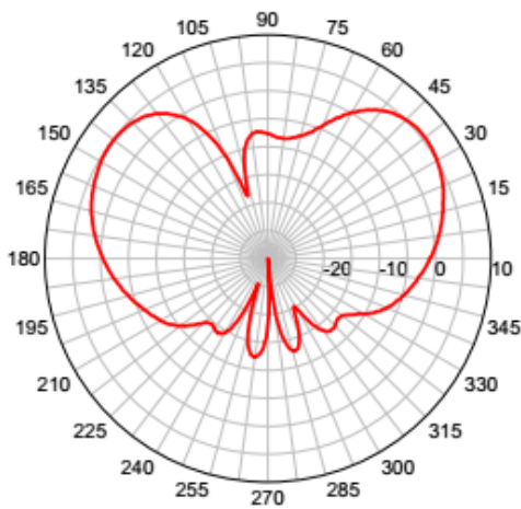
Cable #1 & #2 MGW 2400 MHz Band – Elevation Plot
