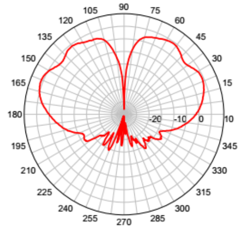
Cable #1 & #2 MGW 5500 MHz – Elevation Plot
