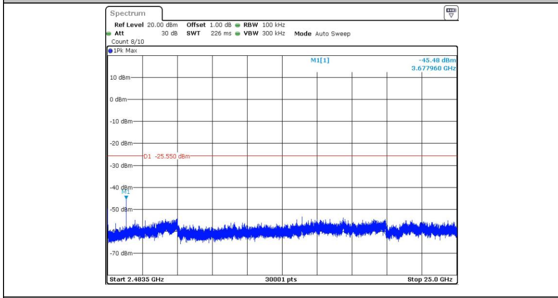
11N40_Ant1_2452_2483.5~25000
