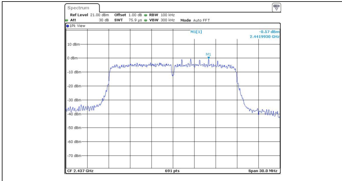
11N20_Ant1_2437_0~Reference
