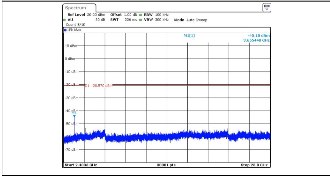
11N20_Ant1_2437_2483.5~25000
