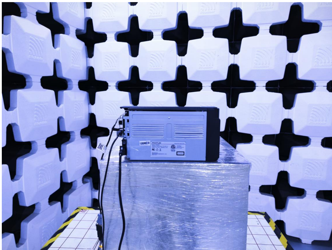
The EUT and transmitting antenna was centered on the turntable
