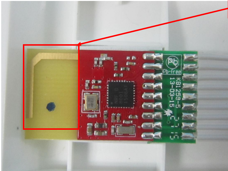
BT antenna
