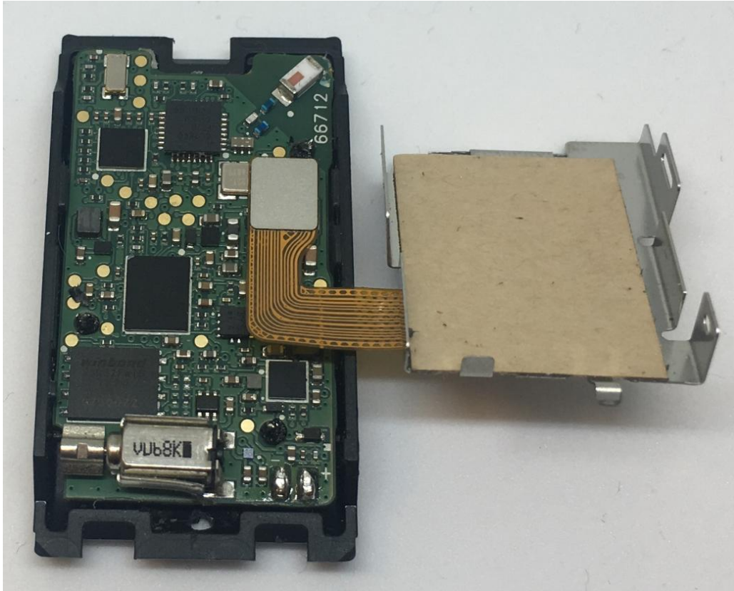
Top side with PCB, display and bracket (disassembled)
