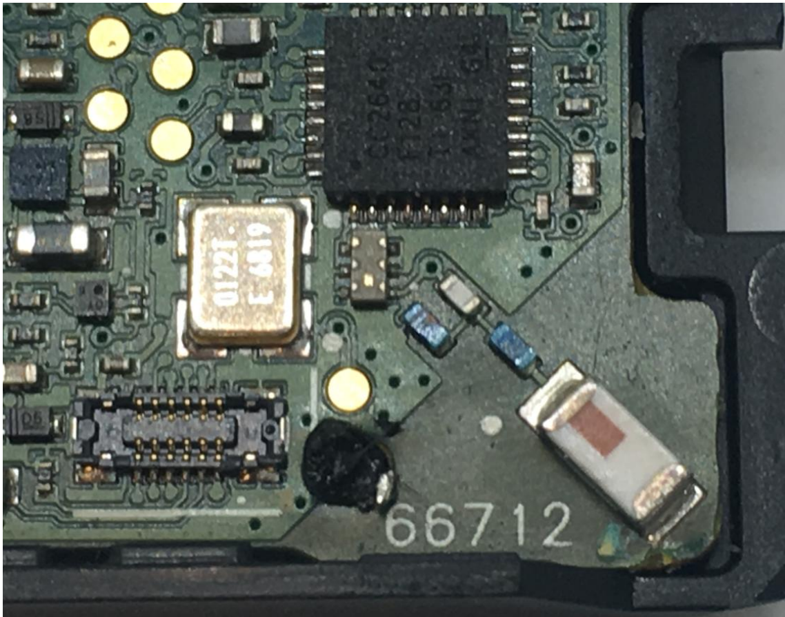
Detail of PCBA showing antenna (1), Balun and matching circuit (2) and Bluetooth controller CC2640 (3)
