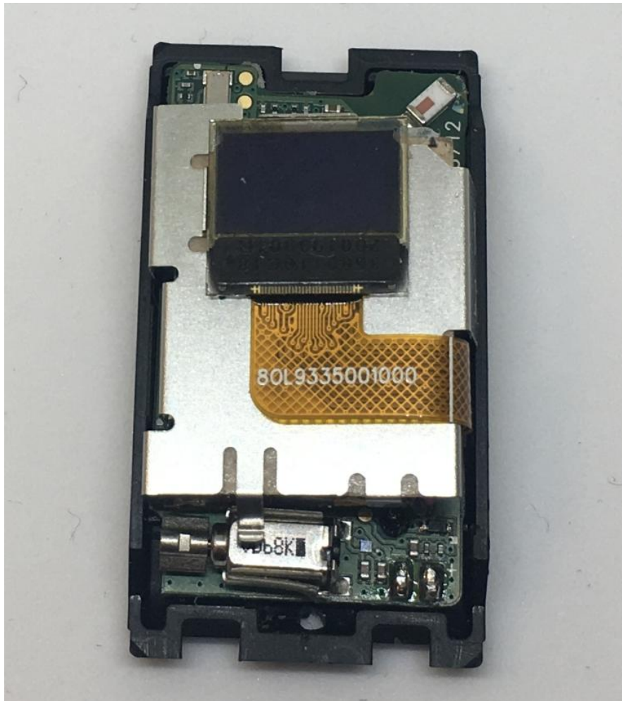
Top side with PCBA, display, battery (hidden) and bracket
