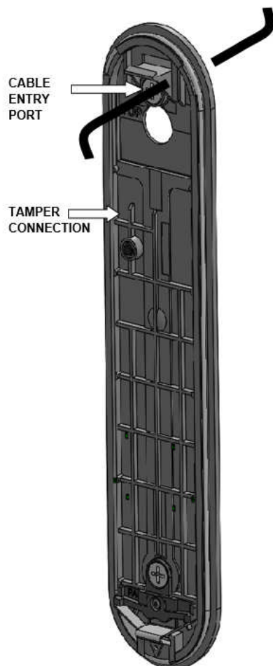
Fixing Plate
