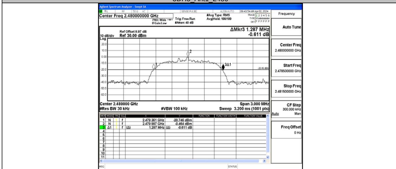
3DH5_Ant1_2480
