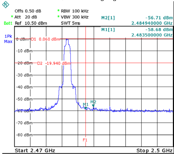
Pi/4 DQPSK Band edge-right side
