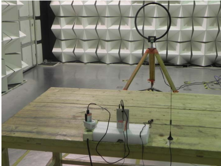
Below 30MHz Test Site 1#
