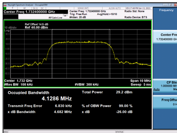
(Plot C2: WCDMA 1700 MHz Channel = 1412 bandwidth)
