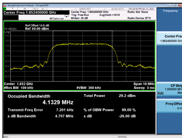
(Plot B1: WCDMA 1900MHz Channel = 9262 Occupied bandwidth)
