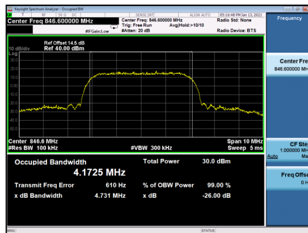
(Plot A3: WCDMA 850MHz Channel = 4233 Occupied bandwidth)
