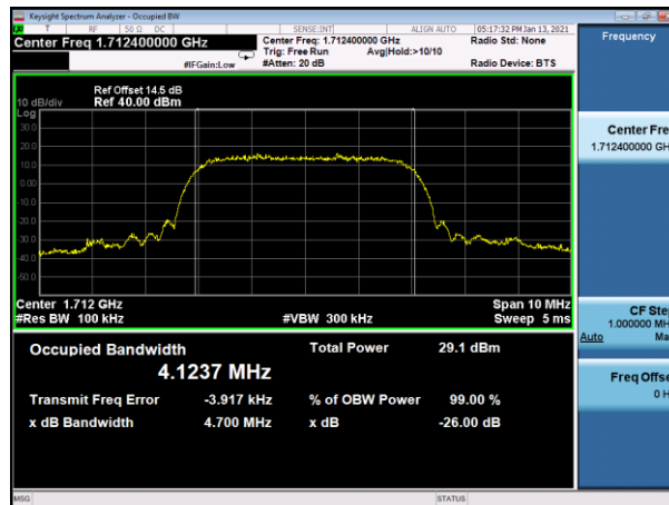
(Plot C1: WCDMA 1700MHz Channel = 1312 bandwidth)
