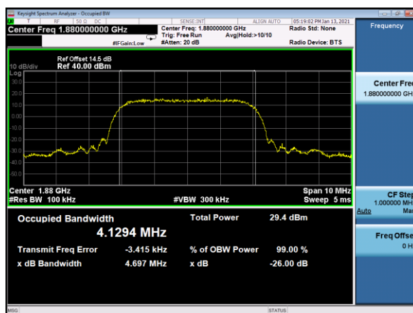
(Plot B2: WCDMA 1900MHz Channel = 9400 Occupied bandwidth)
