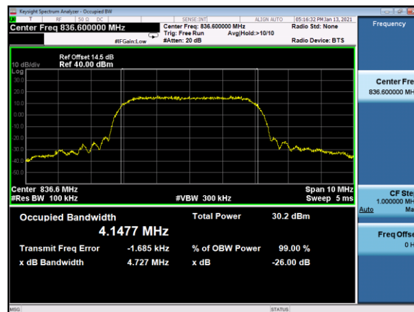
(Plot A2: WCDMA 850MHz Channel = 4183 Occupied bandwidth)
