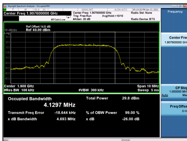
(Plot B3: WCDMA 1900MHz Channel = 9538 Occupied bandwidth)
