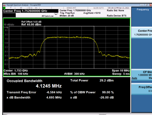
(Plot C3: WCDMA 1700 MHz Channel = 1513 bandwidth)
