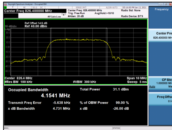
(Plot A1: WCDMA 850MHz Channel = 4132 Occupied bandwidth)
