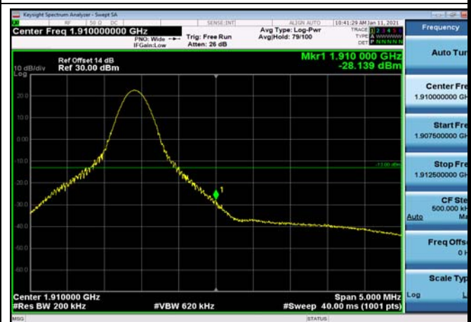
HighRange_FDD02_20MHz_1900_fullIRB _High_Q16
