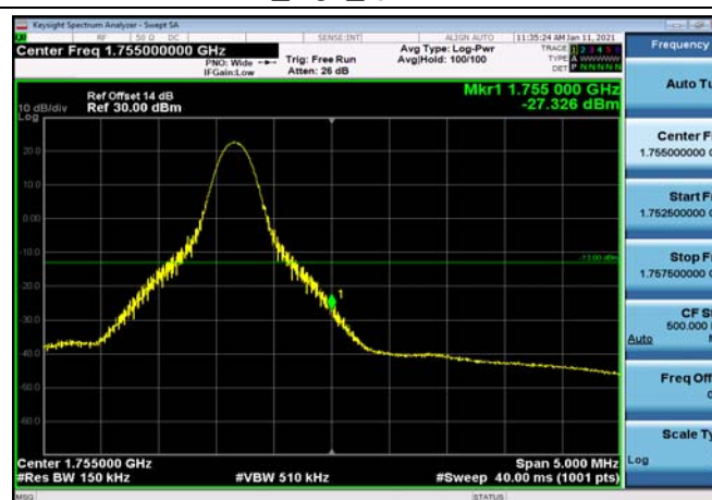
HighRange_FDD04_15MHz_1747.5_fullRB _High_QPSK
