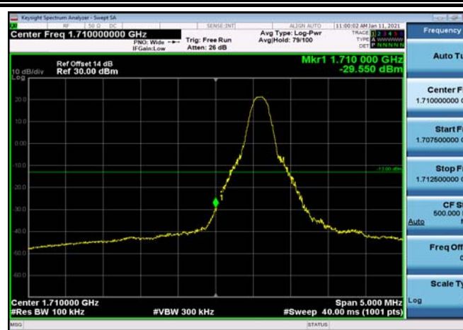
LowRange_FDD04_10MHz_1715_fullRB _Low_QPSK
