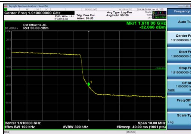
HighRange_FDD02_15MHz_1902.5_OneRB _high_QPSK
