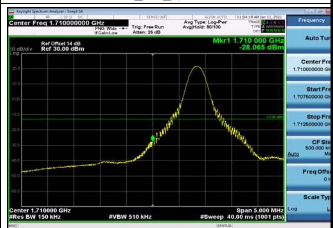
LowRange_FDD04_15MHz_1717.5_fullRB _Low_Q16
