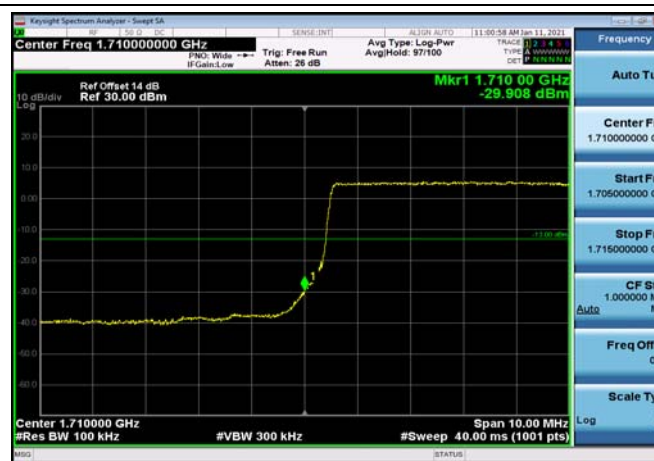
LowRange_FDD04_15MHz_1717.5_OneRB _low_QPSK
