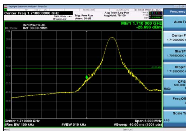
LowRange_FDD04_15MHz_1717.5_fullRB _Low_QPSK
