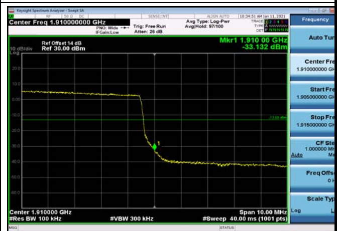
HighRange_FDD02_15MHz_1902.5_OneRB _high_Q16
