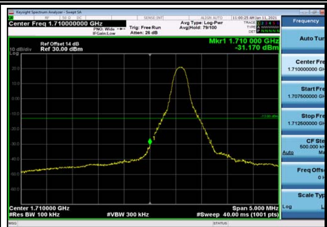
LowRange_FDD04_10MHz_1715_fullRB _Low_Q16
