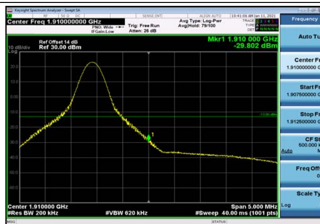
HighRange_FDD02_20MHz_1900_fullIRB _High_QPSK
