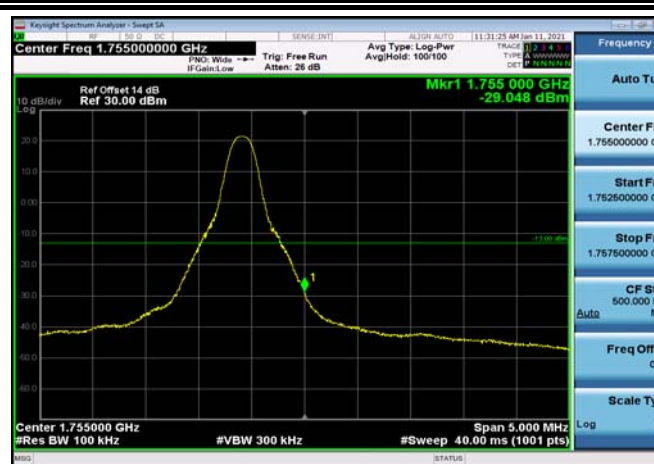
HighRange_FDD04_10MHz_1750_fullRB _High_QPSK
